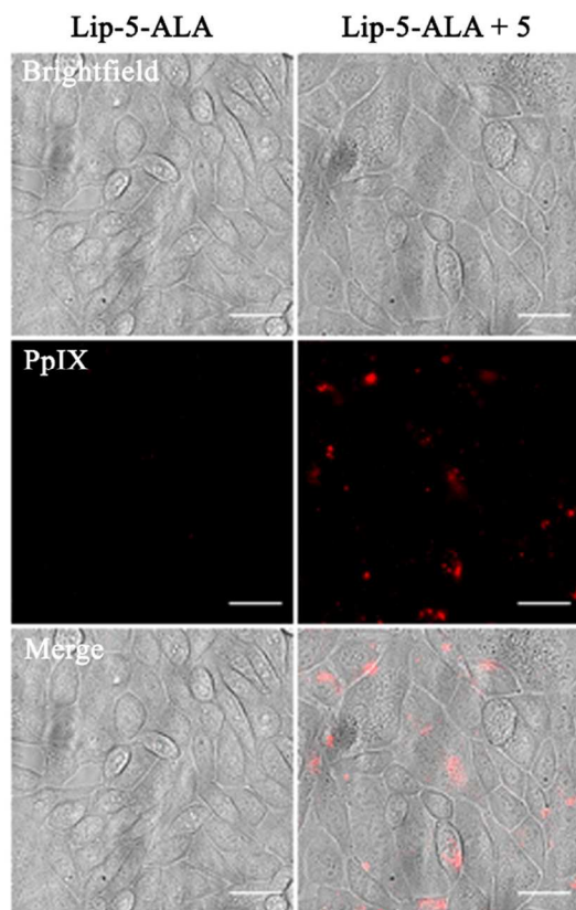
Figure 6: Fluorescence micrographs (Brightfield = top ; Cy 3 (PpIX) = middle ; Merge = bottom ) (60 x) of CHO-K1 cells at six hours after treatment with: ( Left column ) liposomal 5-ALA (100 \mu\text{M} total 5-ALA, 66 \mu\text{M} total lipid), ( Right column ) liposomal-5-ALA (100 \mu\text{M} total 5-ALA, 66 \mu\text{M} total lipid) and 6.6 \mu\text{M} chemical trigger 5 added five minutes later. Scale bar =25 \mu\text{m} .
