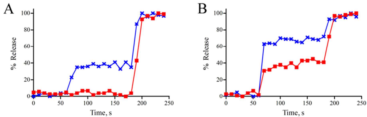
Figure 4: Percent CF release from liposomes (67:28:8:5 DPPC:Chol.:DPPE-PEG 2000 :POPS, 10 \mu M total lipid containing 50 mM CF) treated with either chemical trigger 1 (10 \mu M, A) or 5 (10 \mu M, B) at 60 seconds followed by liposome lysis with Triton-X-100 (20 % v/v, 20 \mu L) at 180 seconds in either PBS buffer ( blue crosses ) or F12-K growth media ( red squares ).
