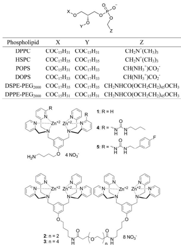
Figure 2: (Top) Chemical structures of relevant phospholipids; (Bottom) Chemical structures of ZnBDPA triggers 1-5.
