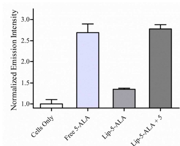
Figure 5: PpIX production by CHO-K1 cells at six hours after addition of media alone, free 5-ALA (100 \mu M), liposomal-5-ALA (Lip-5-ALA, 100 \mu M 5-ALA, 66 \mu M total lipid), or liposomal-5-ALA (100 \mu M 5-ALA, 66 \mu M total lipid) for five minutes followed by chemical trigger 5 (6.6 \mu M). Emission intensities are normalized to cells incubated with media alone, \lambda_{\text{ex}} = 406 nm, \lambda_{\text{em}} = 604 nm.
