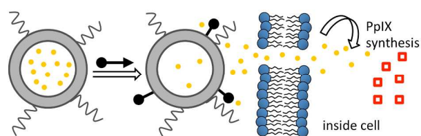
Scheme 1: Cartoon depiction of extracellular triggered release of 5-ALA (yellow circles) from stealth liposomes (grey donut with protruding PEG chains) upon exposure to chemical trigger (black arrow) with subsequent cellular uptake via endogenous amino acid transporters and biochemical conversion to PpIX (red squares).
