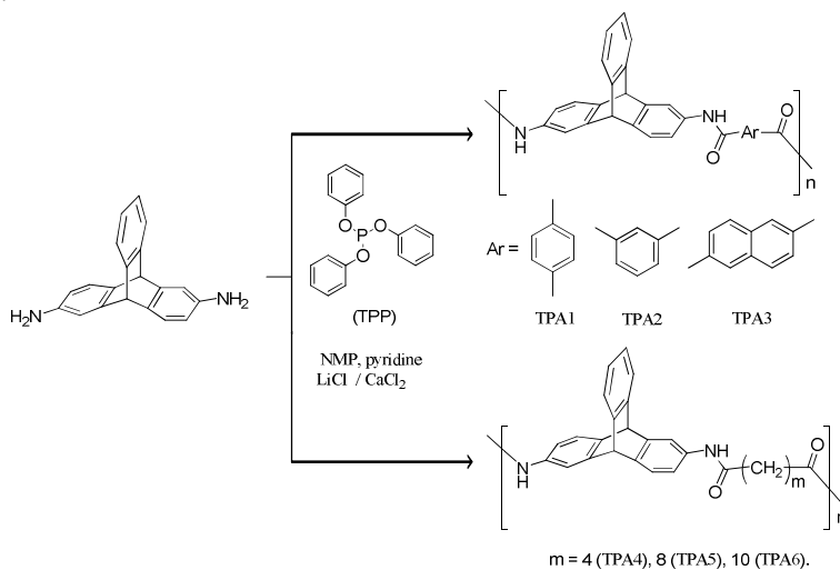
Scheme 2. Synthesis of TPA1-TPA6
