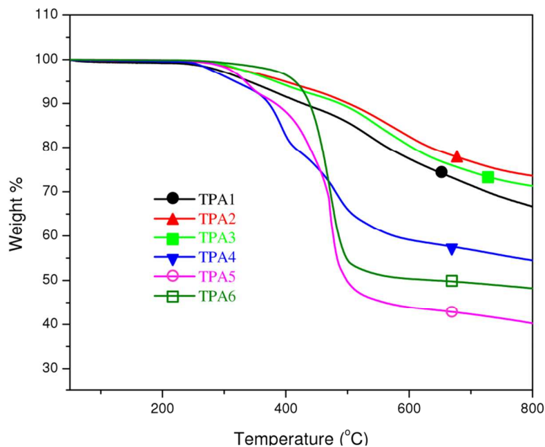
Fig. 3 TGA traces of TPA1-TPA6 under N_2 at a scan rate 10\text{ }^\circ\text{C}/\text{min} .
