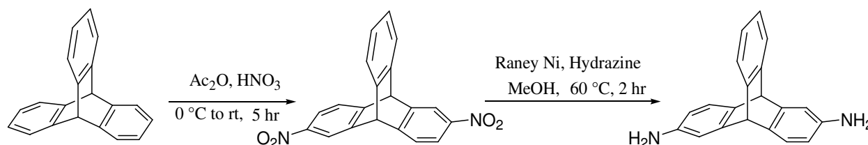
Scheme 1. Synthesis of 2,6-diaminotriptycene ( DAT )
