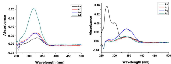
Fig. 2 UV-vis absorbance spectra of the compounds 4d , 4e , 4f , 4p , 4q , 4r , 4u , and 4v in dichloromethane ( c = 1 \times 10^{-6} mol/L).
