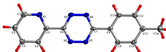
Fig. 5 X-ray crystal structure of 4a .
