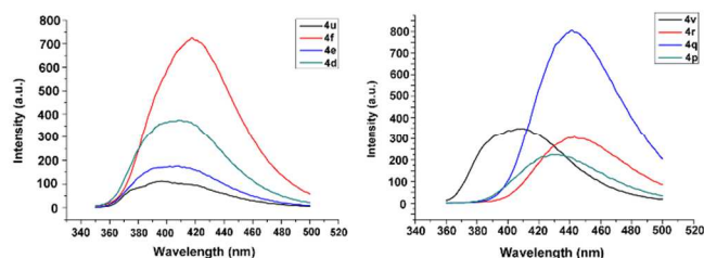
Fig. 3 Fluorescence spectra of the compounds 4d , 4e , 4f , 4p , 4q , 4r , 4u , and 4v in dichloromethane ( c = 1 \times 10^{-6} mol/L).
