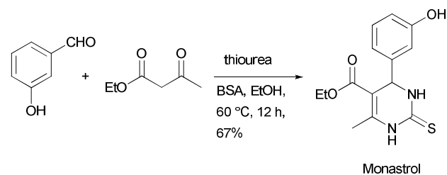
Scheme 14. BSA catalyzed gram scale synthesis of Monastrol.
