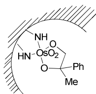
Figure 1. OsO 4 -BSA- \alpha -methylstyrene complex.
