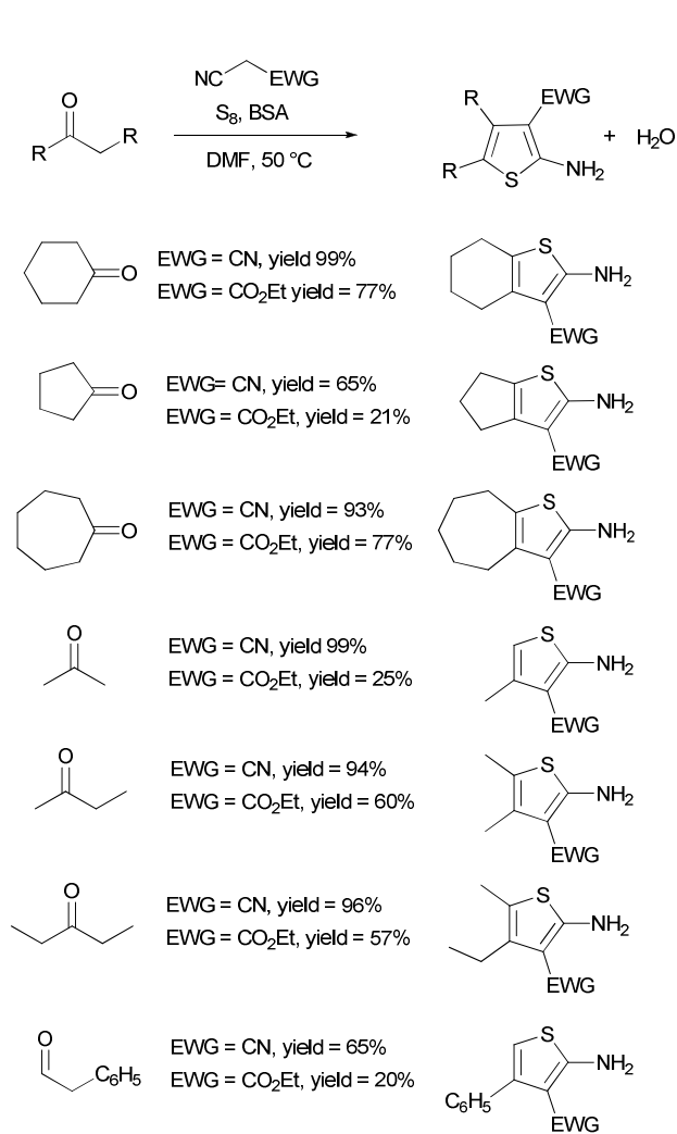
Scheme 7. Gewald reaction catalyzed by BSA.
