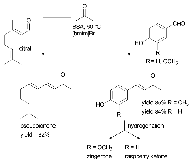
Scheme 8. BSA-[bmim]Br catalyzed synthesis of key intermediates of biologically active compounds.
