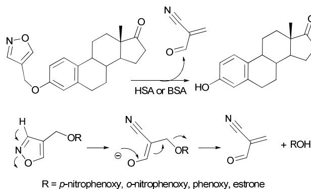
Scheme 17. Activation of estrone prodrug by a tandem Kemp elimination/ \beta -elimination reaction catalyzed by albumin.
