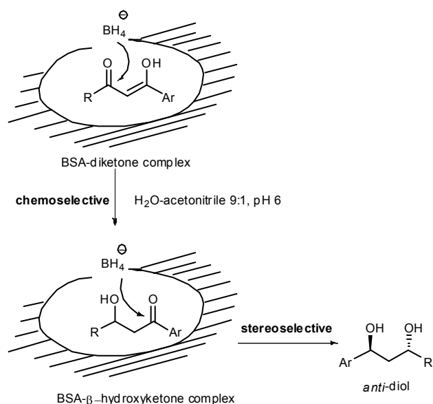
Figure 3. Proposed mechanism of \text{NaBH}_4 -BSA reduction.
