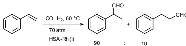
Scheme 1. Hydroformylation of styrene promoted by HSA-Rh complex.
