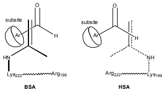
Figure 2. Proposed mechanism for the enamine mediated addition of acetone to 6-methoxy-2-naphthaldehyde promoted by albumin.
