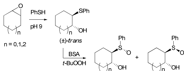
Scheme 21. One pot biomimetic approach to \beta -hydroxy sulfoxides.
