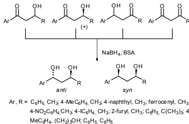
Scheme 23. NaBH 4 -albumin reduction of \beta -hydroxyketones and 1,3-diketones
