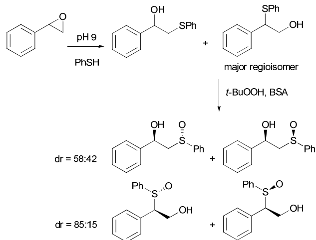
Scheme 22. One pot sulfoxidation of styrene oxide by BSA.
