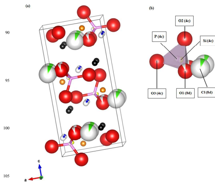
Figure 7. (a) Ball and stick drawing of unit cell of \text{Li}_{10}\text{Si}_{1.5}\text{P}_{1.5}\text{Cl}_{0.5}\text{O}_{11.5} . (b) Enlarged view of the selected P/SiO/Cl 4 polyhedra. Li1 ions: black spheres, Li2 ions: orange spheres, Li3 ions: blue spheres, P ions: pink spheres, Si ions: yellow spheres, O ions: red spheres, Cl ions: green spheres.
