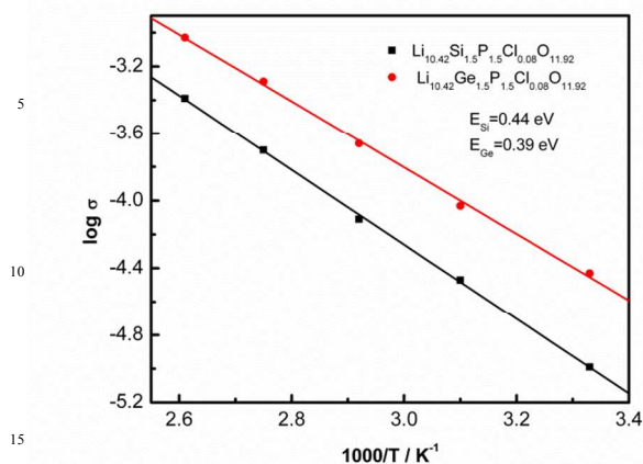
Figure 2. Arrhenius plots of \text{Li}_{10.42}\text{Si}/\text{Ge}_{1.5}\text{P}_{1.5}\text{Cl}_{0.08}\text{O}_{11.92} in the range between 27 °C and 110 °C.
