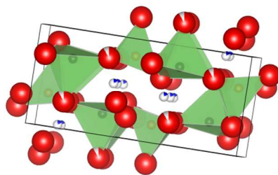
Crystal structure of \text{Li}_{10}\text{Si}_{1.5}\text{P}_{1.5}\text{Cl}_{0.5}\text{O}_{11.5}
