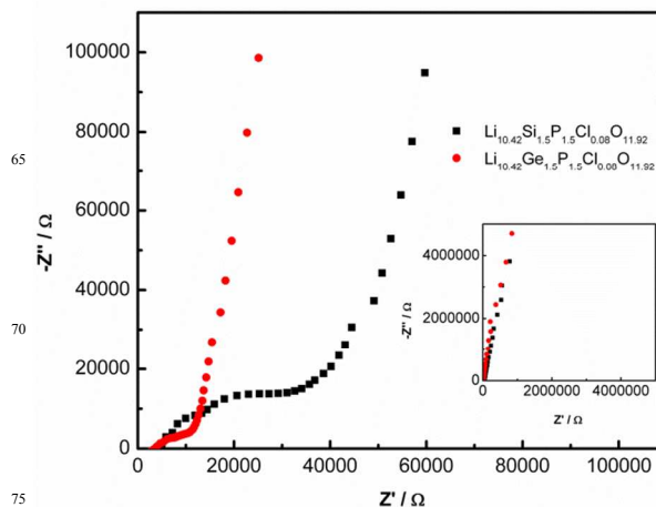
Figure 1. Typical Nyquist plots of \text{Li}_{10.42}\text{Si}_{1.5}\text{P}_{1.5}\text{Cl}_{0.08}\text{O}_{11.92} (square symbol) and \text{Li}_{10.42}\text{Ge}_{1.5}\text{P}_{1.5}\text{Cl}_{0.08}\text{O}_{11.92} (circle symbol) measured at 27 °C.
