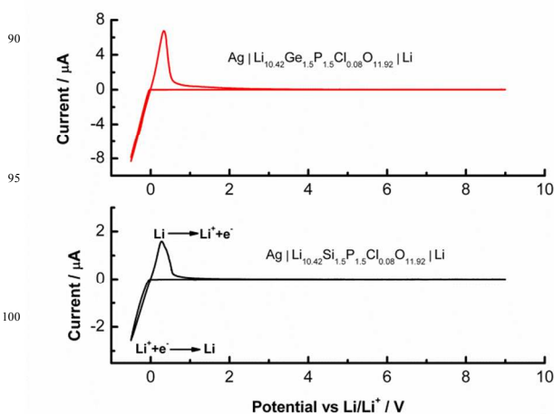
Figure 5. The current-potential curves of \text{Li}_{10.42}\text{Si}/\text{Ge}_{1.5}\text{P}_{1.5}\text{Cl}_{0.08}\text{O}_{11.92} .
