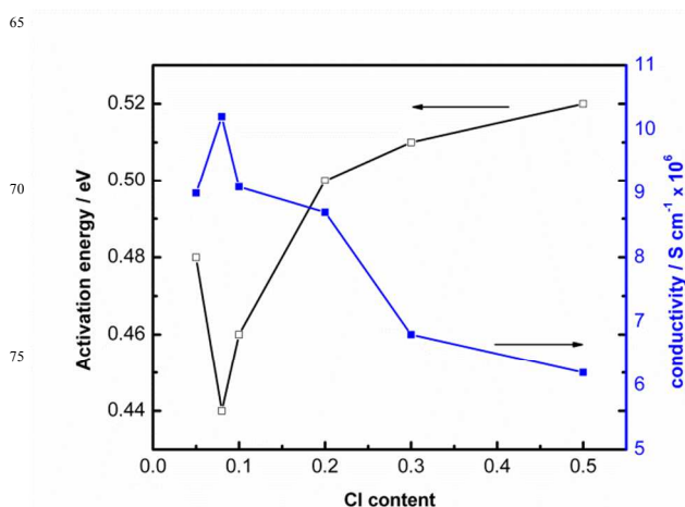
Figure 4. The plots of room-temperature conductivity and activation energy versus Cl content.
