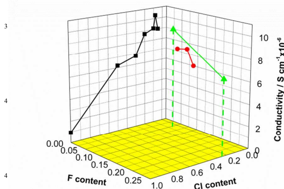
Figure 3. Effect of halide substitution on the room-temperature conductivity of \text{Li}_{10.5-x}\text{Si}_{1.5}\text{P}_{1.5}\text{Cl}/\text{F}_x\text{O}_{12-x} ( 0.05 \leq x \leq 1.0 ).
