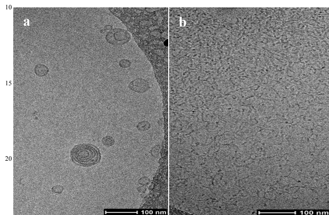
Fig. 3 Cryo-TEM images show that the shape and size of molecular self-assemblies of CD-PG dendrimers in aqueous solution depend on the volume of their hydrophilic PG head groups. G1PG-CD creates multilamellar vesicular structures (a), while G2PG-CD with bigger PG dendrons forms worm-like structures (b).
