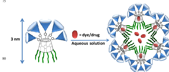
Fig.1 Self-assembly of amphiphilic CD-PG dendrimers in aqueous solutions leads to nanostructures with two different domains to deliver hydrophobic guest molecules.
