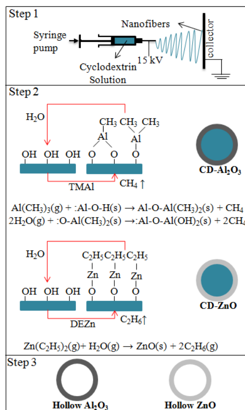
Figure 1. Schematic diagram showing the three step process to fabricate the metal oxide tubes and the mechanism involved in the ALD process.
