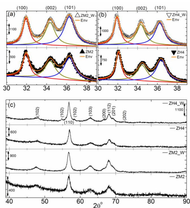
Figure 5. XRD patterns of ALD processed (ZnO) samples before and after washing steps. (a) ZM2, ZM2_W, (b) ZH4, ZH4_W within 30–39° and depicting the deconvolution of three reflections, viz (100), (002) and (101), and (c) 39–90° range is shown for the above samples.
