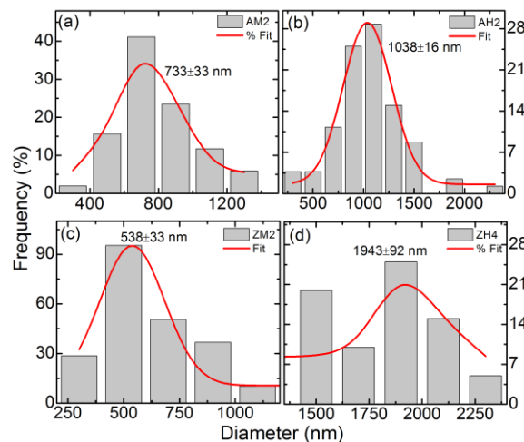
Figure 3. Diameter distribution and the AFD of samples from SEM images. (a) AM2, (b) AH2, (c) ZM2, and (d) ZH4. The center of Gaussian peak (i.e., average fiber diameter) is annotated on each of the distributions.
