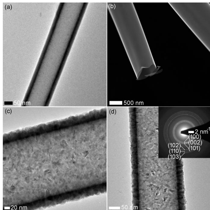
Figure 4. TEM of images of (a) AM2_W, (b) AH2_W, (c) ZM4_W, and (d) ZH4_W. The inset shows ED from ZH4.
