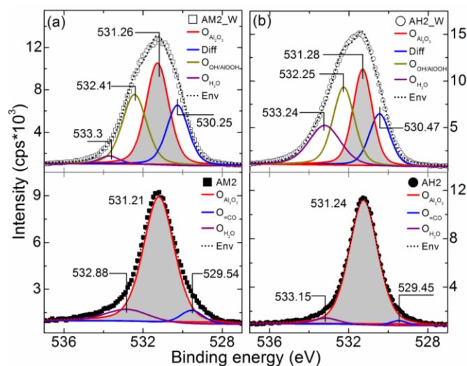
Figure 7. O1s core level XPS spectra from \text{Al}_2\text{O}_3 coated electrospun samples before and after washing steps, (a) AM2, AM2_W and (b) AH2, AH2_W. The peak positions are annotated on the plot in eV.
