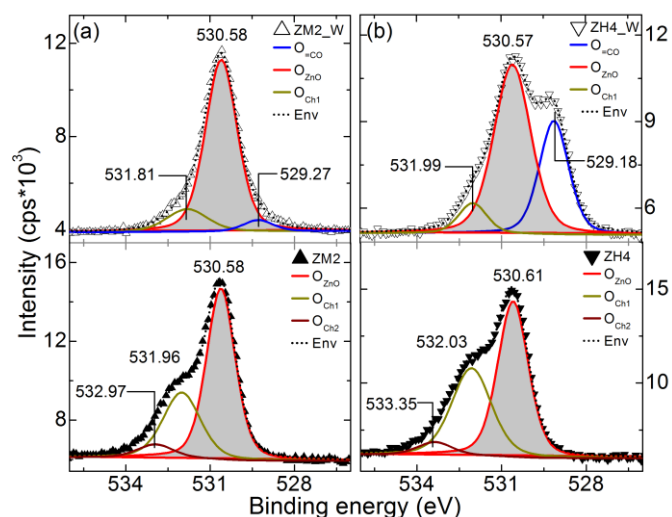
Figure 8. O1s core level XPS spectra from samples before and after washing steps, (a) ZM2, ZM2_W and (b) ZH4, ZH4_W. The peak positions are annotated on the plot in eV.
