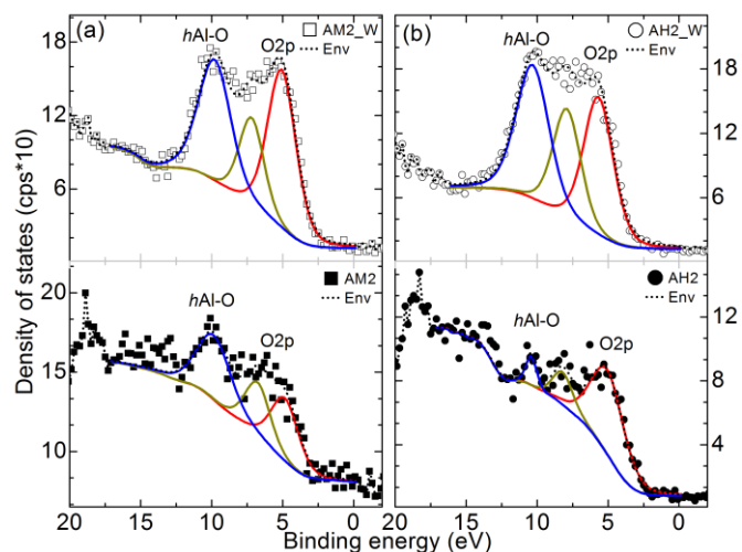
Figure 9. Valence band spectra from Al 2 O 3 coated samples before and after washing steps, (a) AM2, AM2_W and (b) AH2, AH2_W.
