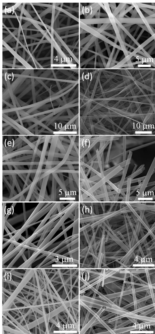
Figure 2. SEM images of samples before and after washing steps. (a) M \beta CD nanofibers, (b) HP \beta CD nanofibers (c) AM2, (d) AM2_W, (e) AH2, (f) AH2_W, (g) ZM2, (h) ZM2_W, (i) ZH4, and (j) ZH4_W.
