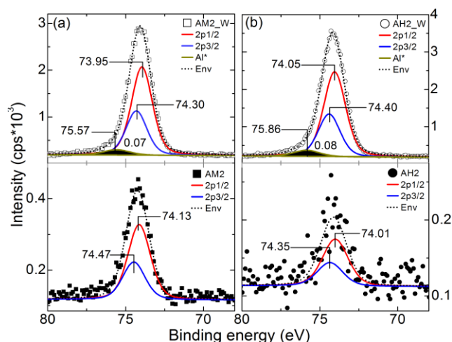
Figure 6. Al core level XPS spectra from \text{Al}_2\text{O}_3 coated samples before and after washing steps, (a) AM2, AM2_W and (b) AH2, AH2_W. The peak positions are annotated on the image in eV. The area ratio of the peak corresponding to hydroxyl bonded Al is annotated for washed samples.
