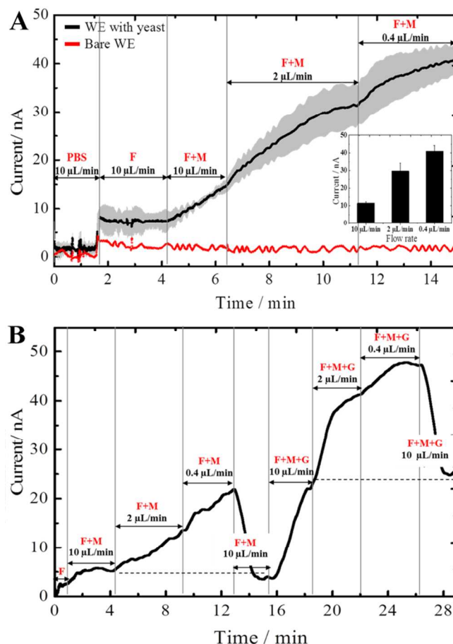
Fig. 2 (A) An averaged current-time recording for three yeast populations each monitored in a different chamber (black line). The grey band represents the SD. The control current-time trace was recorded in a microfluidic chamber without cells (red line). Insert: The signal variation with changing flow rate in the presence of F and M. (B) Current response of a S. cerevisiae population in the presence of ferricyanide (F) and menadione (M) at different flow rates (F+M: basal level of redox activity; F+M+G: redox activity upon accelerated metabolism). Each arrow marks the period of a specific flow rate. The signal intensity is dynamically changing with the flow rate. WEs were biased at +350 mV vs. on-chip Au RE.
