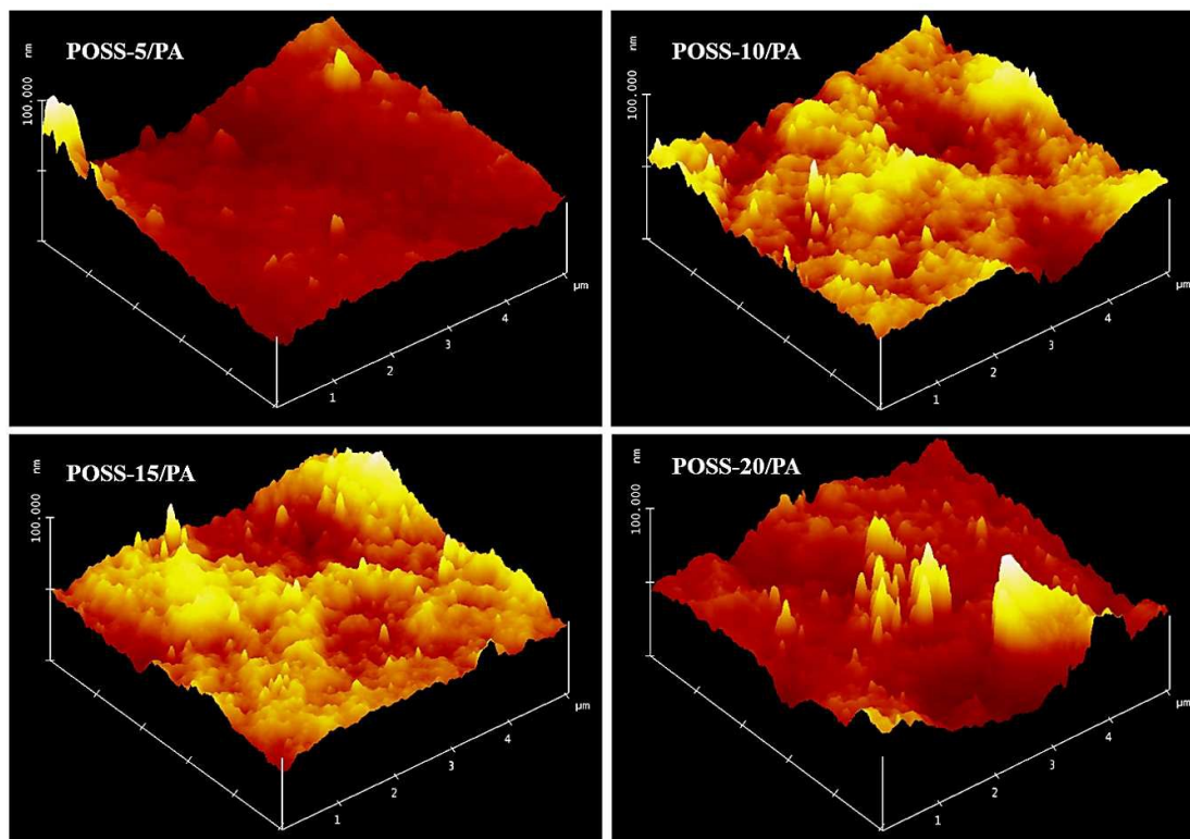
Figure 8: The AFM 3D images ( 5\ \mu\text{m} \times 5\ \mu\text{m} ) exhibit high protuberant and clearly visible flakes with a thickness of \sim 100\ \text{nm} . Atomic force microscopy (topographic image) presents the change in the surface roughness of POSS/PA membranes by changing the POSS content (from 5% to 20 %). The dim and bright regions denote the highest and lowest points of the surface of POSS/PA bio-nanocomposite.
