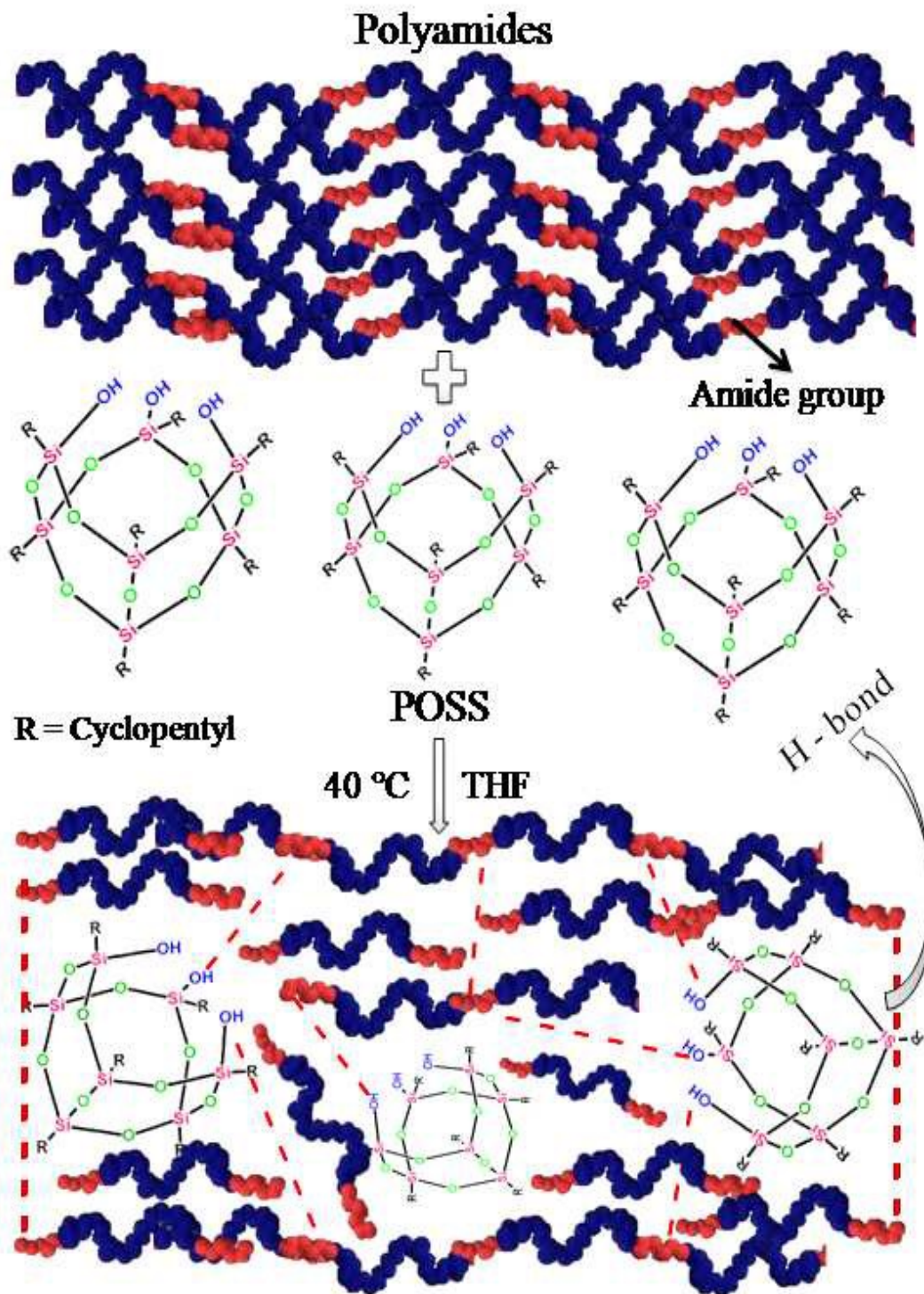
Scheme 1. Systematic methodology for preparing POSS/PA bio-nanocomposite membranes under the condition of 40 °C and in the presence of THF solvent (The possible ways of formation of H-bonds between POSS and polyamides).
