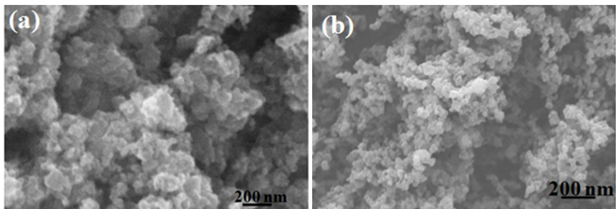
Fig. 2 SEM micrographs of (a) SnO 2 (b) ZnO nanoparticles
