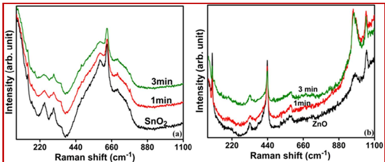
Fig. 8 Raman spectra of (a) SnO 2 and (b) ZnO nanoparticles taken in ammonia environment at different exposure time.
