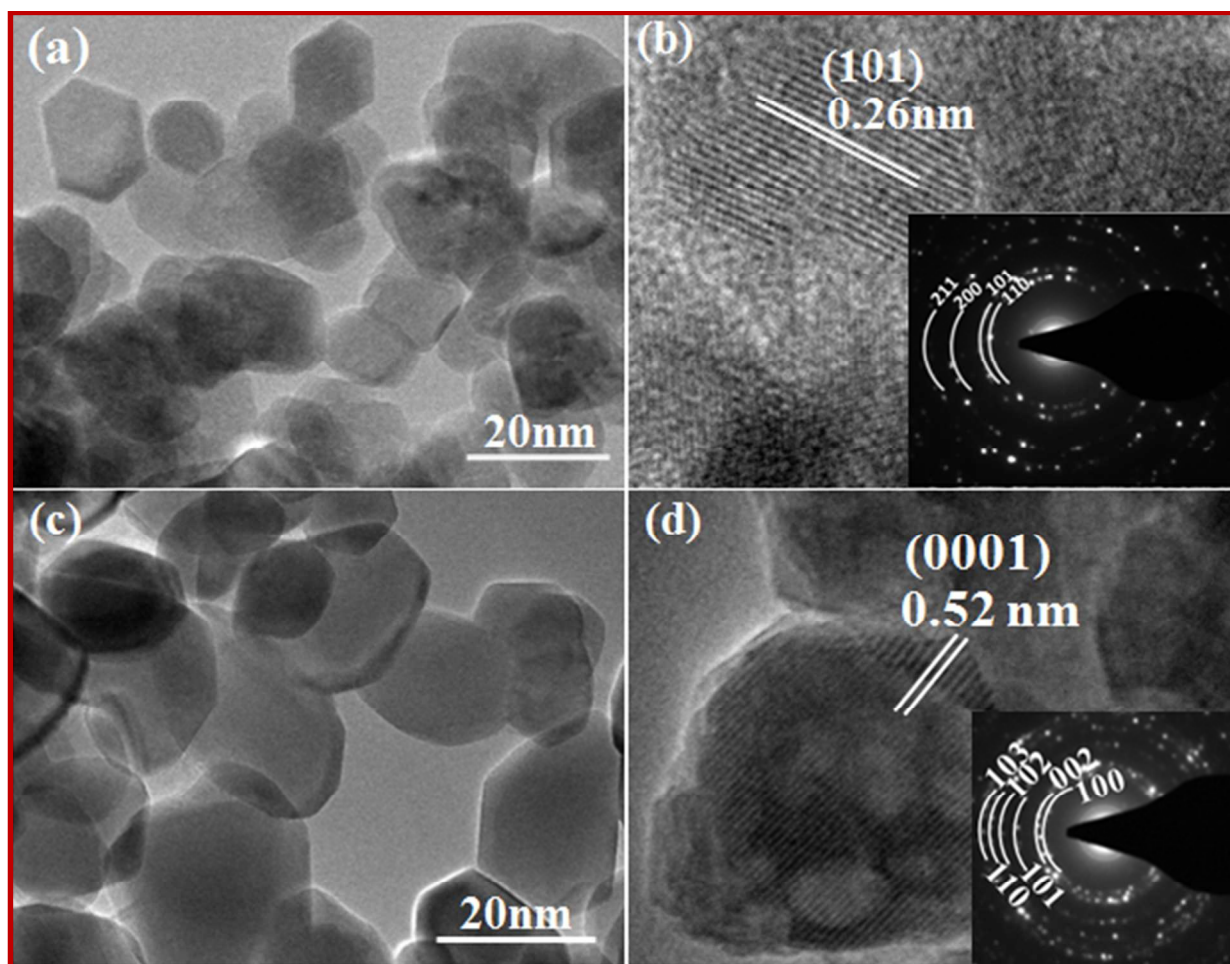
Fig.3 TEM images of (a) SnO 2 (b) HRTEM micrograph SnO 2 (inset SEAD pattern of SnO 2 ) (c) TEM images of (c) ZnO and (d) HRTEM micrograph of ZnO (inset SEAD pattern of ZnO) nanoparticles
