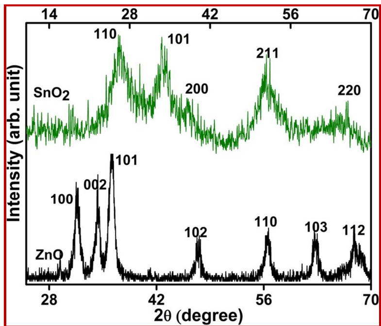
Fig.1 XRD patterns of SnO 2 and ZnO nanoparticles
