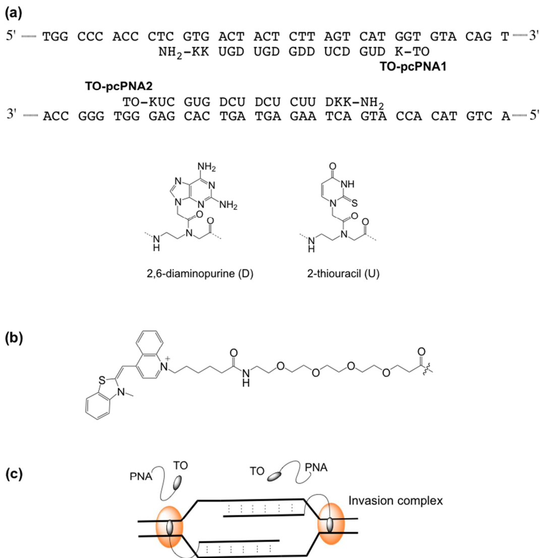
Fig. 1 (a) The sequences of target site in substrate DNA and TO-conjugated pcPNAs (TO-pcPNA1/TO-pcPNA2) with the structures of pseudo-complementary bases D and U. (b) Chemical structures of TO (thiazole orange) and PEG linker. (c) Schematic representation of invasion complex between dsDNA and TO-conjugated pcPNAs. The two TO moieties should intercalate to the adjacent sites in the dsDNA.
