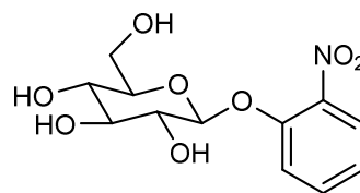
2-nitrophenyl- \beta -D-glucoside
