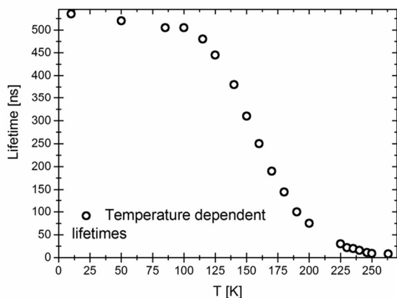
Figure 5: Temperature dependence of the lifetimes of \text{LiSrH}_3:\text{Eu}^{2+} 0.0037 mol %. Excitation at 376.8 nm, emission at 580 nm.
