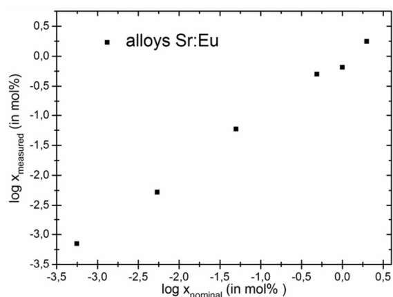
Figure 2 Log-log plot showing the relation between the nominal and real europium contents in the intermetallic phases \text{Eu}_x\text{Sr}_{1-x} .
