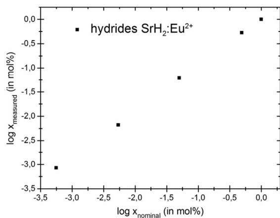
Figure 3 Log-log plot showing the relation between nominal and real europium contents in the hydrides \text{Eu}_x\text{Sr}_{1-x}\text{H}_2 .
