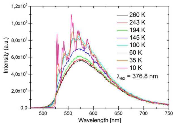
Figure 4 Temperature dependent emission spectra of \text{LiSrH}_3:\text{Eu}^{2+} 0.0037 mol % under UV excitation (376.8 nm).
