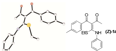
Figure 1 Molecular structure of ( Z )- 1a
