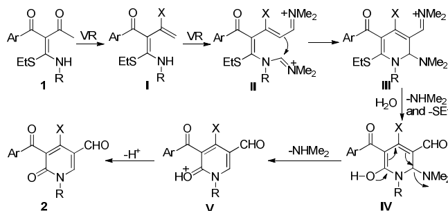
Scheme 3 Plausible Mechanism of Vilsmeier cyclization of \alpha -acetyl- \alpha -aroil ketene- N , S -acetals 1
