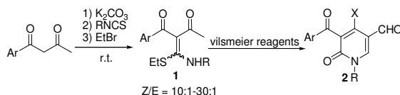
Scheme 1 Vilsmeier cyclization of acyclic substrates
