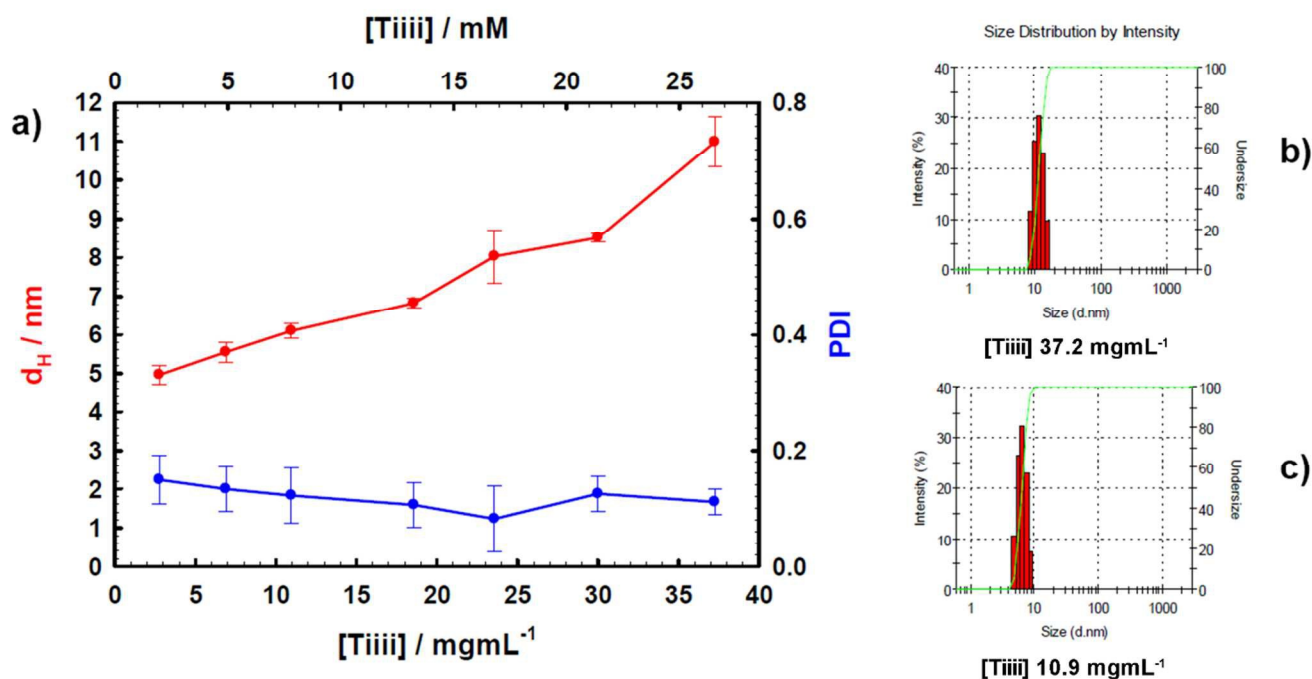
Fig. 1 DLS analysis (CHCl 3 , 25 °C): a) hydrodynamic diameter and PDI of the homopolymer 5 as function of concentration; b), c) examples of size intensity distributions at different concentrations
