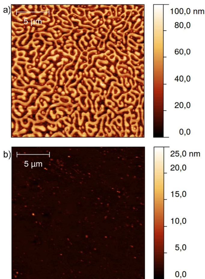
Fig. 4 a) AFM topographic image of PS/PBMA mixture, deposited by spin coating of a dichloromethane solution, displaying large lateral inhomogeneities; b) the same for a film made of 1:1 molar mixture PS-Host/PBMA-Sarc, exhibiting an homogeneous and flat morphology.
