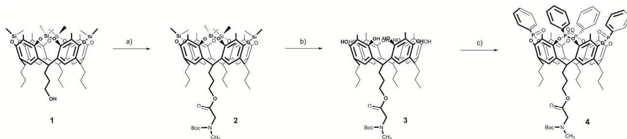
Scheme 1 Synthesis of Tiiii [3 C 3 H 7 , 1 sarcosine BOC protected, CH 3 , Ph], I: a) N -Boc-Sarcosine, DCC/DMAP, CHCl 3 , r.t., 12 h, 40%; b) TBAF, THF, r.t., 1 h, 60%; c) 1) PhPCl 2 , Py, 75 °C, 3h; 2) H 2 O 2 , r.t., 1h, 92% (over two steps); d) TFA, DCM, r.t., 3h, quantitative.
