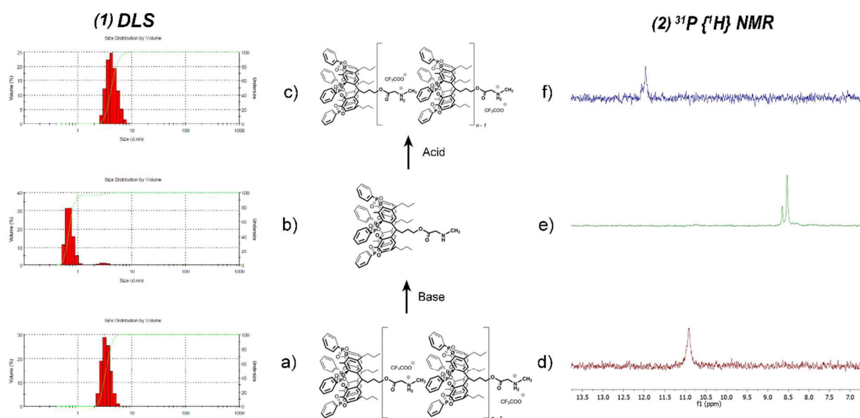
Fig. 2 (1) DLS experiments (hydrodynamic diameter, \text{CHCl}_3 , 10.5 mM, 25 °C): a) homopolymer; b) homopolymer + 3 eq. DBU; c) homopolymer + 3 eq. DBU + 5 eq. trifluoroacetic acid; (2) ^{31}\text{P}\{^1\text{H}\} NMR spectra ( \text{CDCl}_3 , 400 MHz, 10 mM, 25 °C) of: d) homopolymer; e) homopolymer + 3 eq. DBU; f) homopolymer + 3 eq. DBU + 5 eq. of TFA.
