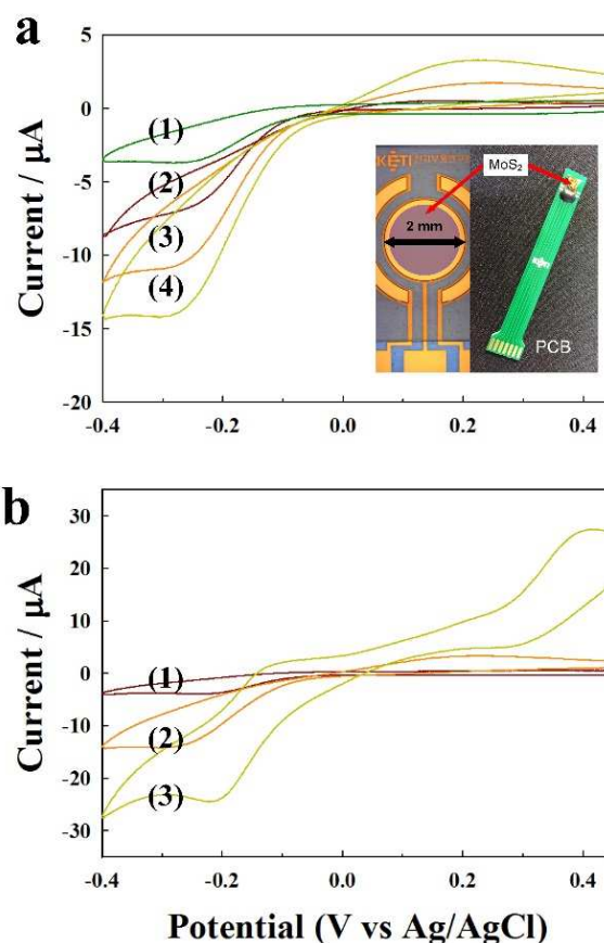
Fig. 2 Cyclic voltammetry (CV) MoS 2 thin film deposited on Au electrode at different scan rate (a) (1) only 10 mM PBS without 5 mM \text{H}_2\text{O}_2 (used as buffer) at a scan rate of 10 mVs -1 , (2) 5 mM \text{H}_2\text{O}_2 at a scan rate of 10 mVs -1 , (3) 50 mVs -1 , and (4) 100 mVs -1 . The inset shows fabricated gold electrode chip on glass wafer and it mounted on printed circuit board (PCB). (b) (1) Only 10 mM PBS without \text{H}_2\text{O}_2 at a scan rate of 10 mVs -1 , (2) 5 mM \text{H}_2\text{O}_2 at 100 mVs -1 , (3) Redox cycling that combines 1 ng/mL IgG-HRP at 100 mVs -1
