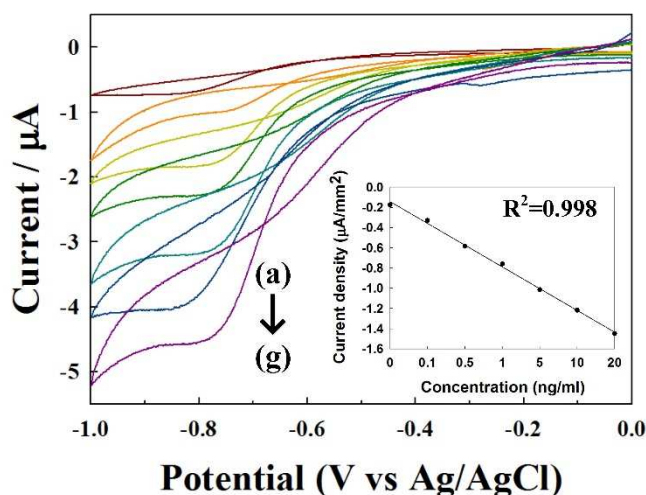
Fig. 3 CV of surface modification by MoS 2 combine various concentration of IgG-HRP, (a) 0, (b) 0.1, (c) 0.5, (d) 1, (e) 5, (f) 10 and (g) 20 ng/mL at 100 mVs -1 . The inset is the calibration curve of the current density to the concentration of IgG-HRP from 0 to 20 ng/mL at -0.8 V.
