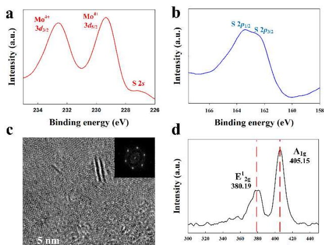
Fig. 1 Chemical composition analysis of as-prepared MoS 2 thin films using PECVD by X-Ray photoemission spectroscopy (XPS) (a) Mo 3d and (b) the S 2p region. (c) A typical HR-TEM image taken from the center of MoS 2 at 300 °C. The insets are the selected area electron diffraction (SAED) (d) The Raman spectra, which is the E 12g and A 1g vibrational modes of MoS 2 on an Au electrode.
