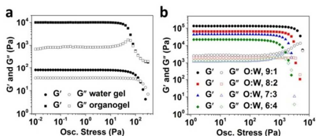
Fig. 3 a) Amplitude stress sweeps (elastic and viscous moduli, G' and G'' versus oscillatory stress) of water gel (prepared using 1 wt% LBG:Car at a ratio of 1:1) and organogel (at 15 wt% A150); b) Amplitude stress sweeps for bigels prepared at different O:W ratios.
