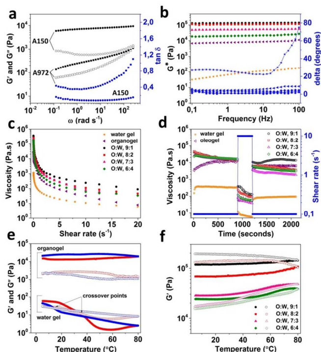
Fig. 5 a) Comparative plots from frequency sweeps of organogels prepared using 15 wt% of hydrophilic (A 150) and hydrophobic (A 972) silica particles; b) & c) Curves from frequency sweeps and flow measurements respectively for water gel, organogel and bigels prepared at different O:W ratios, the figure legends in figure 5c applies to 5b as well; d) curves from 3 interval thixotropy test done on water gel, organogel and bigels prepared at different O:W ratios; e) G' and G'' measured as a function of temperature for water gel and organogel subjected to heating (red symbols) and cooling (blue symbols) steps, the filled and open symbols represent G' and G'' respectively; f) G' measured as a function of temperature for bigels prepared at different O:W ratios, filled and open symbols represent heating and cooling steps respectively.
