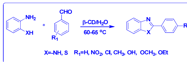
70 Scheme 1. Synthesis of benzothiazoles/benzimidazoles.
