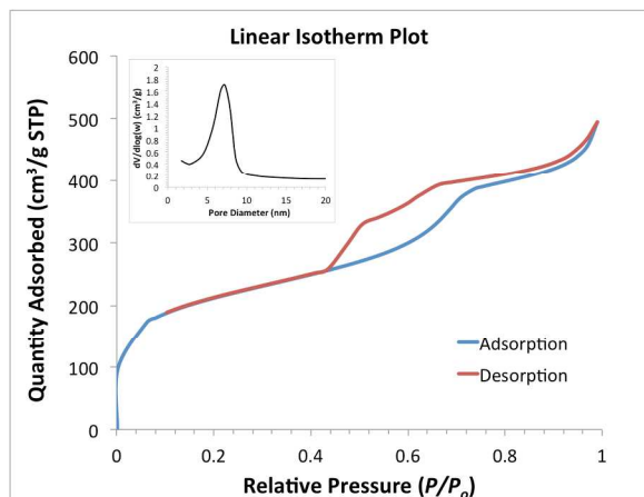
Figure 2. N_2 adsorption-desorption of Pd/SBA-15 and the pore size distribution of the adsorption branch (inset).
