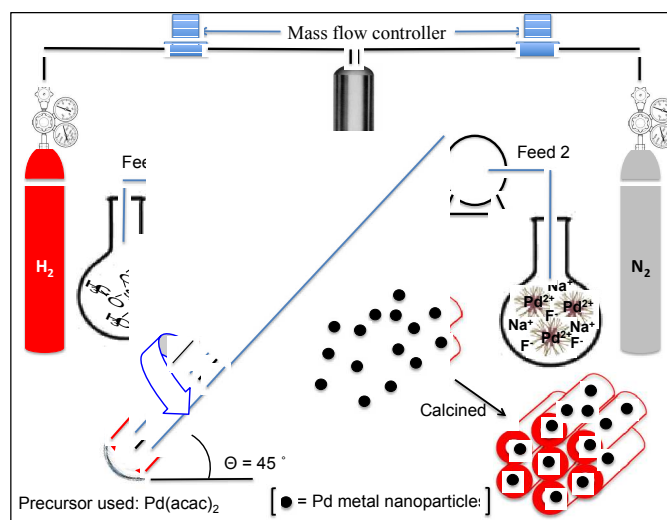
Figure 1. Schematic of the continuous synthesis of Pd/SBA-15 using a vortex fluidic device (VFD).
