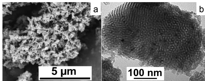
Figure 3. (a) SEM image of Pd/SBA-15 and (b) TEM image of Pd/SBA-15.
