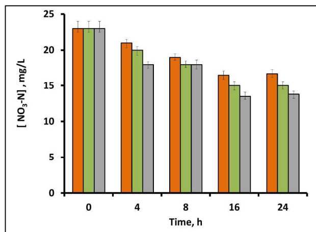
Figure 4. Nitrate-nitrogen [ NO_3^- -N] content of aqueous media in mg/L versus time for three different Pd/SBA-15 loading concentrations: (1) 10 mg adsorbent (brown column); (2) 25 mg adsorbent (green column); and (3) 50 mg adsorbent (grey column).
