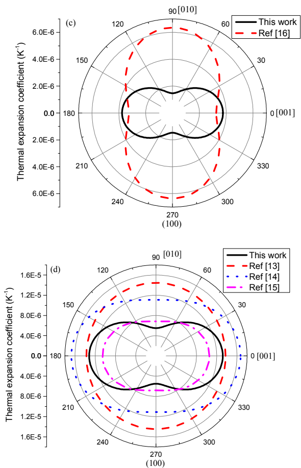
Figure. 8 Two-dimensional polar plot of linear thermal expansion coefficient on (100) plane. For 2H-WS 2 , we use the absolute values of the TEC tensor components in the calculation.
