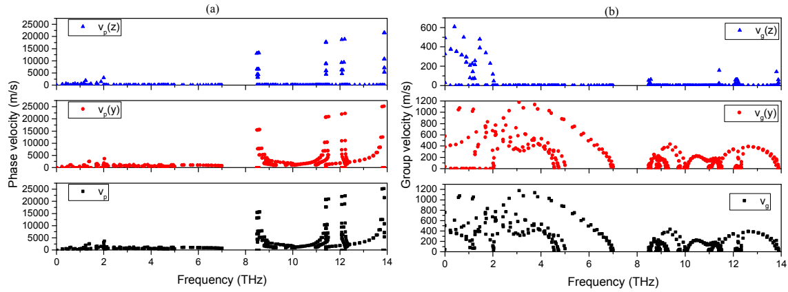
Figure. 6 Phonon velocities of 2H-MoS 2 . (a): Phase velocities; (b): Group velocities.
