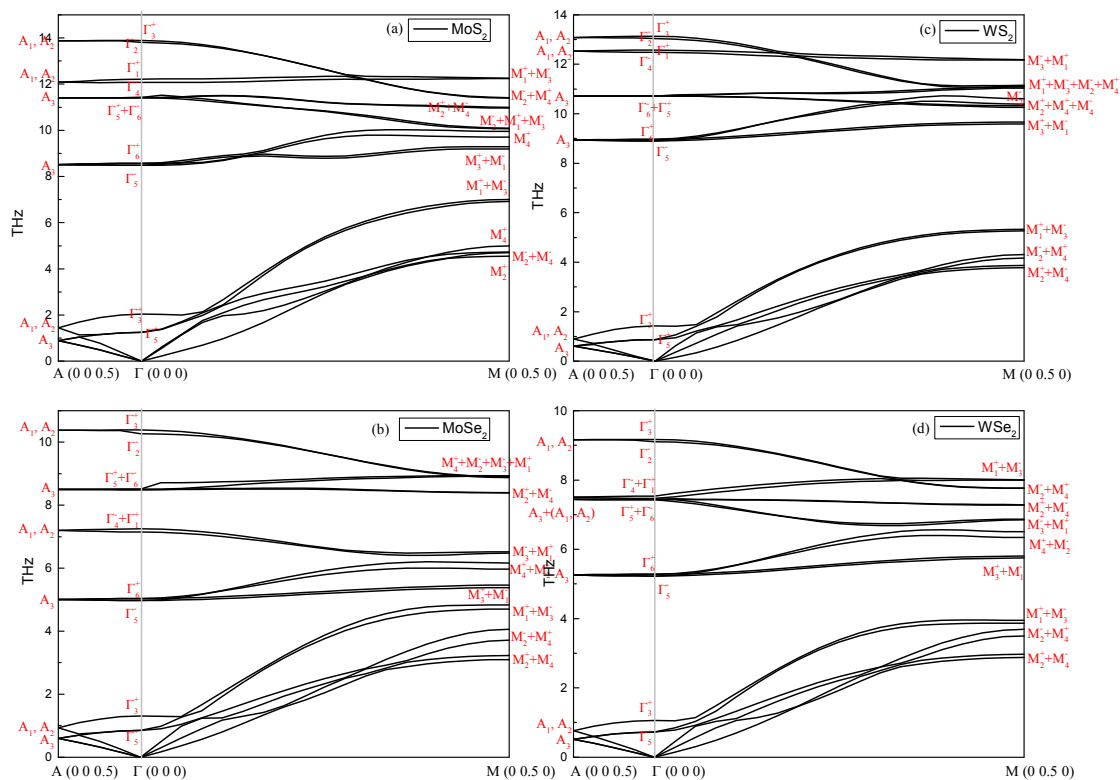
Figure.2 The phonon spectra and irreducible representations of phonon modes at A, \Gamma and M points are shown for (a): 2H-MoS 2 ; (b): 2H-MoSe 2 ; (c): 2H-WS 2 ; (d): 2H-WSe 2 . Note that the path \Gamma -A refers to [001] direction, and \Gamma -M is parallel to [010] direction.
