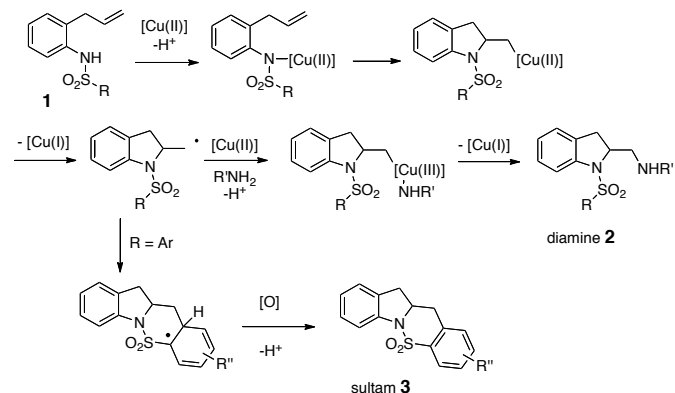
Scheme 2. Proposed copper(II)-catalyzed diamination mechanism.
