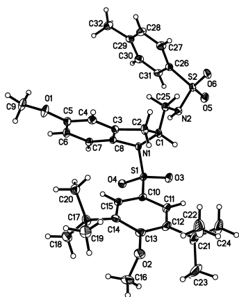
Figure 1. X-ray structure of diamine 2j .
