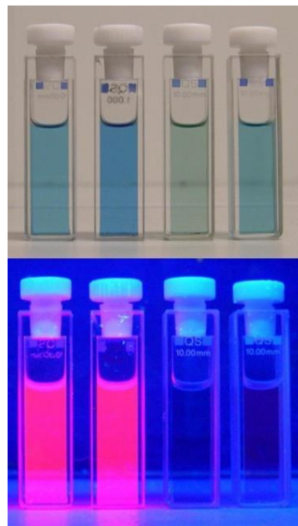
Fig. 10 Solutions of metal complexes M-1 of the PiCC 1 in MeOH (with M = Zn(II), Cd(II), Cu(II), Ni(II)), as observed under day light (top), or under UV light at a wavelength of 366 nm (bottom).
