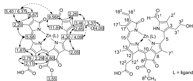
Fig. 6 Left: Graphical representation of 1 H-chemical shift data from a 500 MHz 1 H-NMR spectrum of Zn-1 in CD 3 CN/d 6 -DMSO (10:1) with correlations from H,H-ROESY-spectra (solid and dashed arrows). Right: Deduced constitutional formula of Zn-1 (atom numbering used follows a convention for linear tetrapyrroles 16 and is exemplified here).
