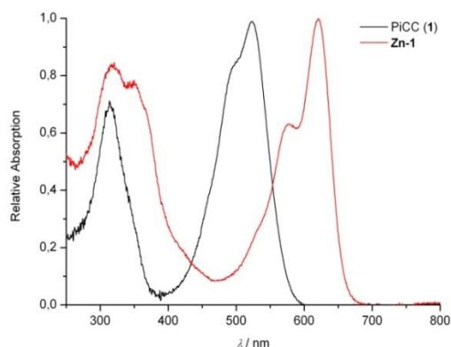
Fig. 2 UV/Vis-spectra of the PiCC 1 (6.97 \mu\text{M} ) and of its zinc-complex Zn-1 (9.67 \mu\text{M} ) in MeOH, normalized to 1.00 at the absorption maxima of both spectra.
