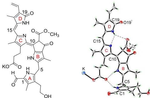
Fig. 3 Chemical formula of the potassium salt ( K-1 ) of the pink phyllobiladiene-b,c (PiCC) 1 and ORTEP-model based on the crystal structure of K-1 (atoms are coloured black (C), red (O), blue (N), green (H), and cyan (K)).
