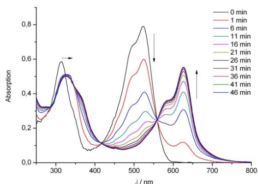
Fig. 8 UV/Vis-spectroscopic analysis of Ni-incorporation into the PiCC 1 . Reaction of 1 (20 \mu\text{M} ) with 10 eq. of Ni(OAc) 2 in MeOH at 22 °C gives Ni-1 cleanly.
