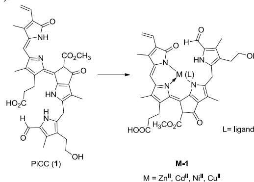
Fig. 4 Incorporation of divalent transition metal ions into the PiCC 1 gives the complexes M-1 (e.g. with M = Zn, Cd, Cu, Ni).
