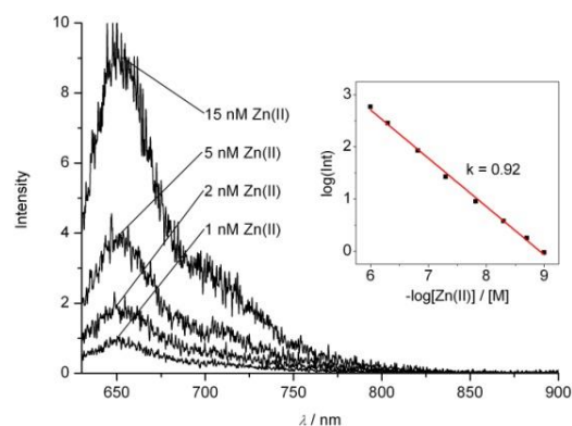
Fig. 9 Assay for Zn(II)-ions in solution by detection of the red fluorescence of the zinc complex Zn-1 . Top. Fluorescence spectra for solutions of PiCC ( 1 , 7.0 \mu\text{M} ) in MeOH and concentrations of Zn(II)-ions (total) from 1000 nM down to 15 nM. Bottom. Fluorescence spectra for solutions of PiCC ( 1 , 7.0 \mu\text{M} ) in MeOH and concentrations of Zn(II)-ions (total) from 15 nM down to 1 nM; Insets: Linear log/log plots of the fluorescence intensity at 650 nm vs. total concentration of zinc ions (see Experimental Part and Supporting Information for details). Fluorescence spectra and values of intensities at 650 nm were corrected for weak background luminescence of the solution of pure 1 (for uncorrected spectra and further details, see Supporting Information).
