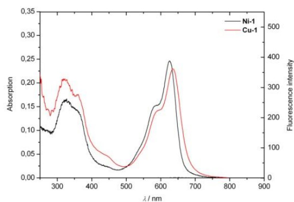
Fig. 5 UV/Vis-spectra and fluorescence emission spectra (full lines), as well as fluorescence excitation spectra (dashed lines) of solutions of M-1 in MeOH. Top. Spectra of Zn-1 and Cd-1 (9.67 \mu\text{M} ). Bottom. Spectra of Ni-1 and Cu-1 (9.67 \mu\text{M} ).
