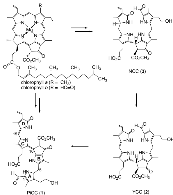
Fig. 1 Chlorophyll breakdown products in higher plants: Nonfluorescent chlorophyll catabolites (NCCs), such as to the colorless NCC 3 , 6, 14, 15 accumulate in various senescent leaves as rapidly formed products of the degradation of the chlorophylls a and b . In some leaves, the NCC 3 was oxidized to the yellow catabolite (YCC) 2 , 13 followed by further oxidation to the pink catabolite (PiCC) 1 . 11
