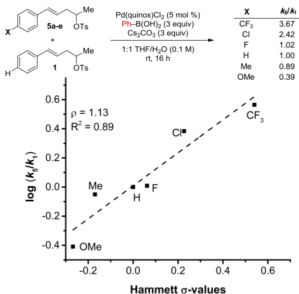
Scheme 2 Hammett correlation to the relative rates of consumption of para -unsubstituted- and para -substituted secondary homostyrenyl tosylates.
