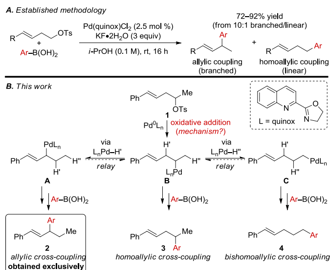
Scheme 1 A. Previous relay Suzuki cross-coupling of primary homostyrenyl tosylates. B. Mechanistic rationale to account for three potential products resulting from the reaction of a secondary homostyrenyl tosylate under Pd(quinox) catalysis.
