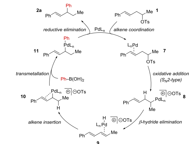
Scheme 3 Proposed mechanism for the relay Suzuki cross-coupling of a secondary homostyrenyl tosylate to phenylboronic acid.
