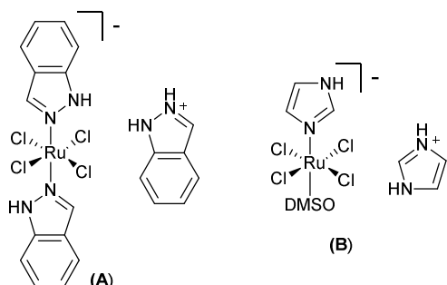
Chart 1. Structures of KP1019 (A) and NAMI-A (B).
