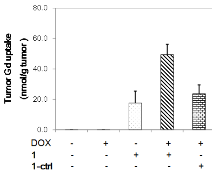
Fig. 7 ICP-MS analysis of tumor Gd uptake. Mice bearing subcutaneous HeLa tumors were untreated or treated with DOX ( 0.2 \text{ mg} \times 2 ). After treatment, 1 or 1-ctrl ( 0.1 \text{ mmol kg}^{-1} ) was injected i.v., and the mice were sacrificed after 1 h. The tumors were resected, weighted, and digested with 69% \text{HNO}_3 . The total Gd amount was analyzed by ICP-MS, and the tumor Gd uptake was normalized to tumor weight. Each data point and error bar represents the mean and standard deviation of 5 mice.
