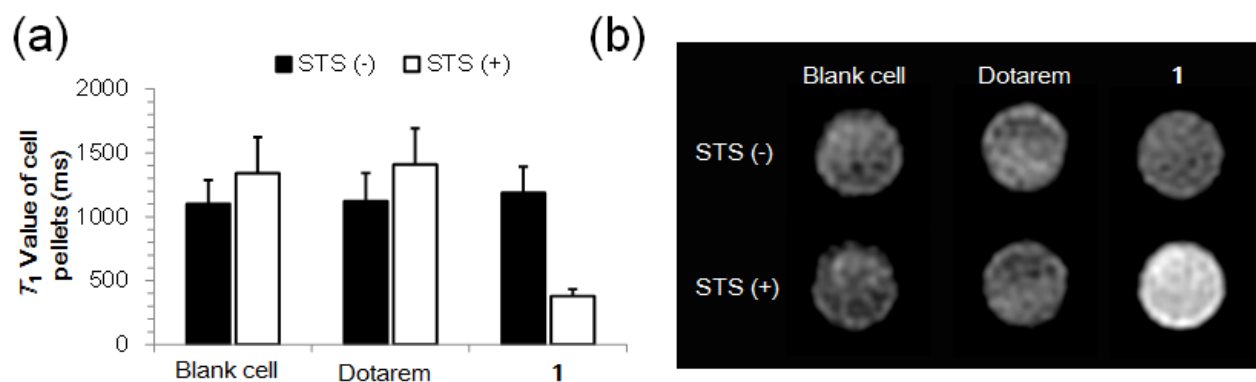
Fig. 5 MR studies of cell incubating with 1 . (a) T_1 values (1 T) of viable and apoptotic HeLa cell pellets after incubation with 250 \mu\text{M} of 1 or Dotarem for 24 h. (b) T_1 -weighted MR images (3T, TE/TR = 30/100 ms) of viable and apoptotic HeLa cell pellets after incubation with 250 \mu\text{M} 1 or Dotarem for 24 h.
