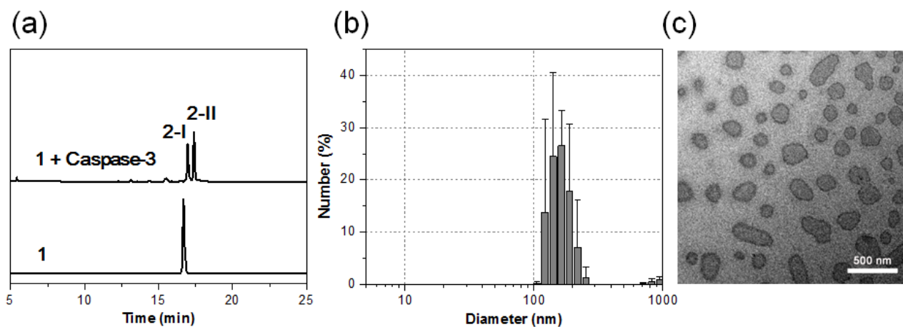
Fig. 2 Caspase-3 mediated macrocyclization and self-assembly into GdNPs in vitro . (a) HPLC traces of 1 (bottom) and the incubation of 1 (200 \mu M) with recombinant human caspase-3 (50 nM) in the caspase buffer at 37 ^{\circ} C for 5 h (top). (b) DLS analysis of 1 (200 \mu M) following incubation with caspase-3 (50 nM) in caspase buffer (pH 7.4) overnight. Error bars indicated standard deviation, coming from three repeated measurements. (c) TEM images of GdNPs formed in the solution shown in (b). Scale bar: 500 nm.
