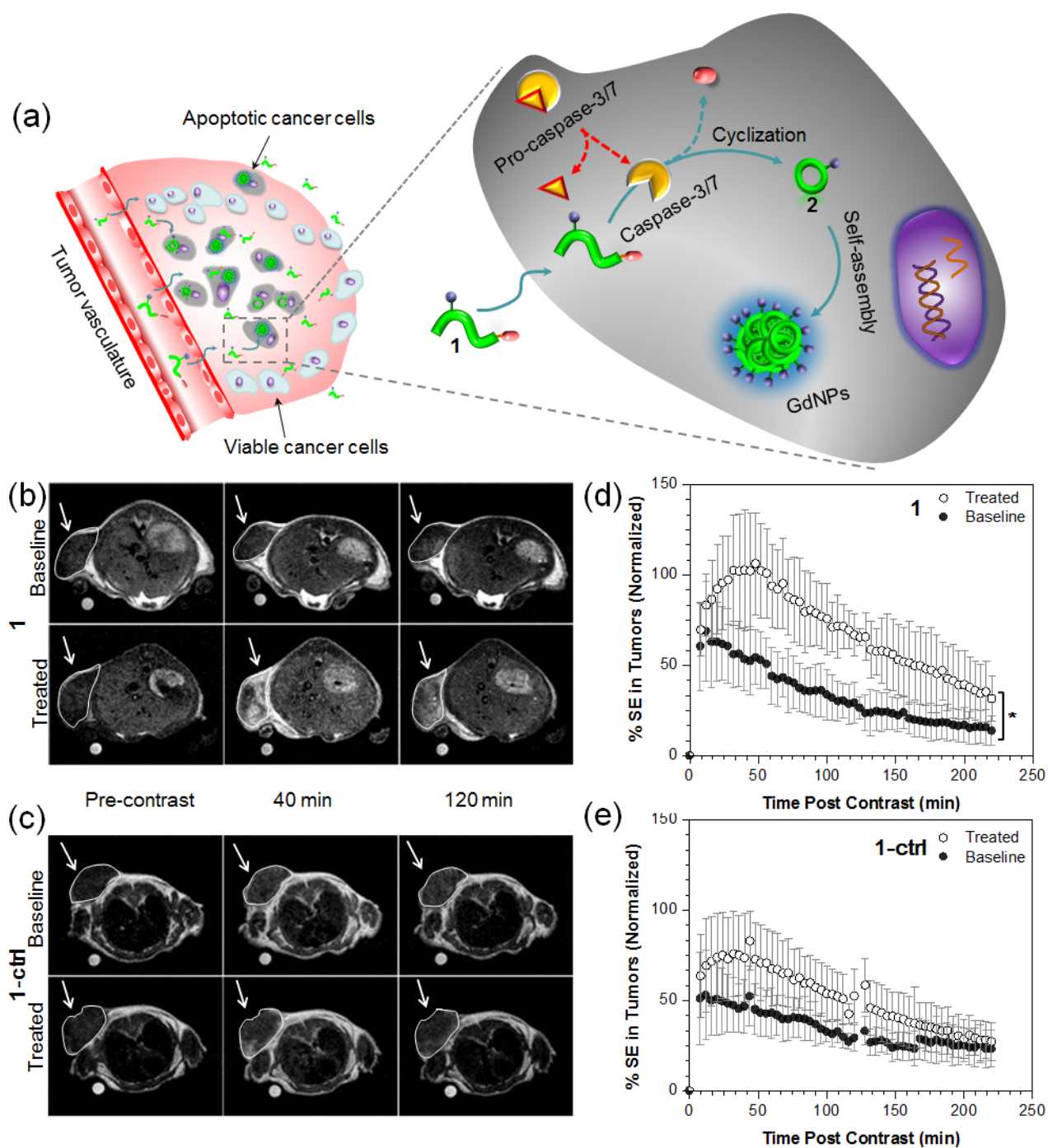
Fig. 6 Non-invasive MR imaging of tumor cell death in mice. (a) The proposed mechanism of 1 for in vivo MR imaging of caspase-3/7 activity in a chemotherapy-responsive tumor. (b, c) Representative T_1 -weighted MR images (1T) of HeLa tumors prior to (baseline) or following treatment with DOX (treated). Images were obtained before (pre-contrast), 40 and 120 min after i.v. injection of 0.1 mmol/kg of 1 (b) or 1-ctrl (c). (d, e) The average longitudinal % signal enhancement (% SE) in baseline (●) and treated (○) tumors after i.v. injection of 1 (n = 8, c) or 1-ctrl (n = 4, d) at 0.1 mmol/kg dose. The tumor signal intensity (SI) was normalized to the reference standard in a mini-NMR tube (1
