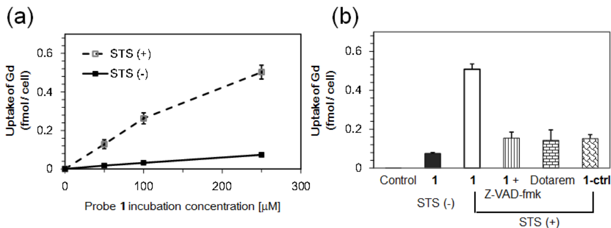
Fig. 4 Cell uptake studies with 1 . (a) ICP-MS analysis of Gd uptake in viable and STS-induced apoptotic HeLa cells with 1 . HeLa cells were untreated or treated with 2 μM STS for 4 h, and then incubated with 0, 50, 100, and 250 μM of 1 for 24 h. After incubation, the cell pellets were collected, washed with PBS, and digested with 69% HNO 3 . The uptake of Gd in cells was obtained from ICP-MS analysis, and normalized to cell number. Each data point and error bar represents the mean and standard deviation of three experiment results. (b) ICP-MS analysis of Gd uptake in apoptotic HeLa cells with different Gd-based MRI probes at 250 μM for 24 h. Each data point and error bar represents the mean and standard deviation of three experimental results.
