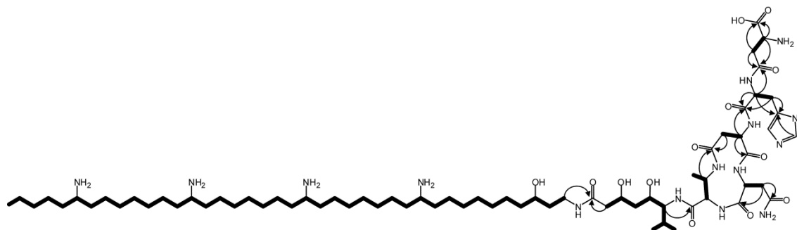
Fig. 6 Overview of key 2-D NMR correlations observed for prezeamine ( 4 ). Spin systems observed in the 2-D hetero-TOCSY spectrum are depicted as bold lines. Arrows indicate the ^1\text{H} to quaternary ^{13}\text{C} correlations observed in the 2-D HMBC spectrum.
