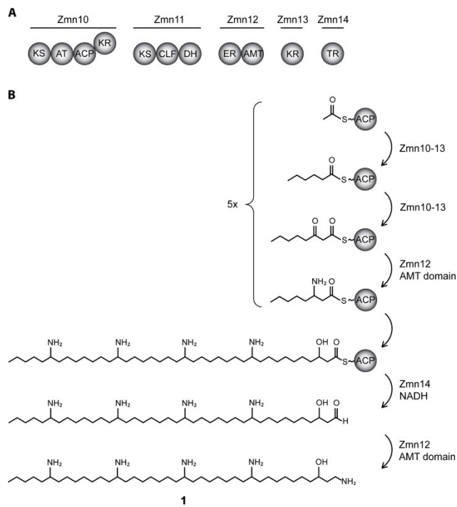
Fig. 1 Biosynthesis of zeamine II ( 1 ). A) Domain and module organization of Zmn10-14 which constitute a type I iterative FAS/PKS showing high homology to PUFA synthases. B) Proposed biosynthetic scheme for zeamine II. Domains are abbreviated as follows: KS = ketosynthase, KR = ketoreductase, ACP = acyl carrier protein, CLF = chain length factor, TR = thioester reductase, DH = dehydratase, ER = enoyl reductase, AMT = aminotransferase.
