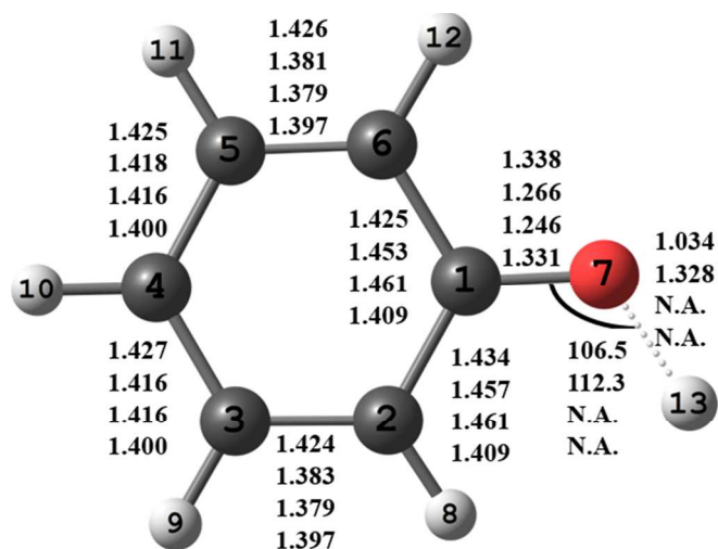
Figure 1. The figure shows the structure of the transition state on adiabatic surface S_1 , and it also shows four sets of bond distances for key eight C–C, C–O, and O–H bond lengths (in Å) and the C–O–H bond angle (in degrees). From top to bottom are values for the equilibrium geometry of the S_1 state of phenol, the saddle point of the S_1 state (the structure shown), the \tilde{X}^2B_1 state of phenoxyl radical, and the \tilde{A}^2B_2 state phenoxyl radical. “N.A.” denotes not applicable.
