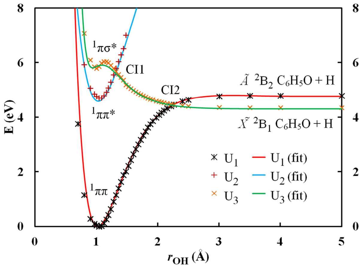
Figure 2. Calculated and APRP diabatic potential energy curves of phenol along the O–H dissociation coordinate. The other geometric parameters are fixed at their values at the equilibrium geometry of ground state phenol. The locations of the conical intersections on the APRP surfaces for these cuts are r = 1.316 Å and r = 2.231 Å, respectively.
