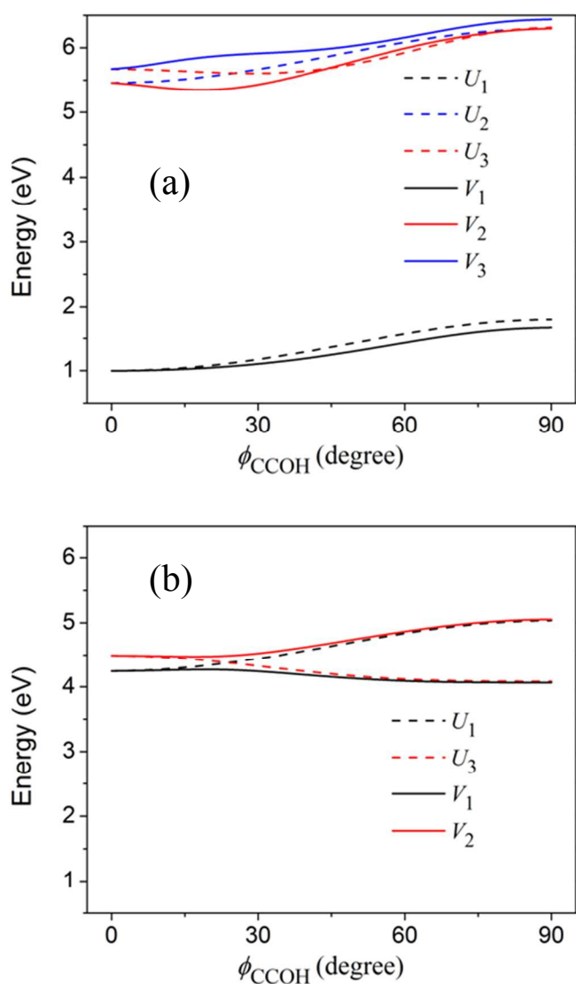
Figure 10. Diabatic potentials ( U_1 , U_2 , and U_3 ) and adiabatic potentials ( V_1 , V_2 , and V_3 ) versus C2-C1-O-H torsion \phi_{\text{CCOH}} (a) with r_{\text{OH}} = 1.29 \text{ \AA} and all other geometric parameters fixed at the ground state equilibrium geometry of phenol, (b) with r_{\text{OH}} = 2.10 \text{ \AA} and all other geometric parameters fixed at the ground state equilibrium geometry of phenol.
