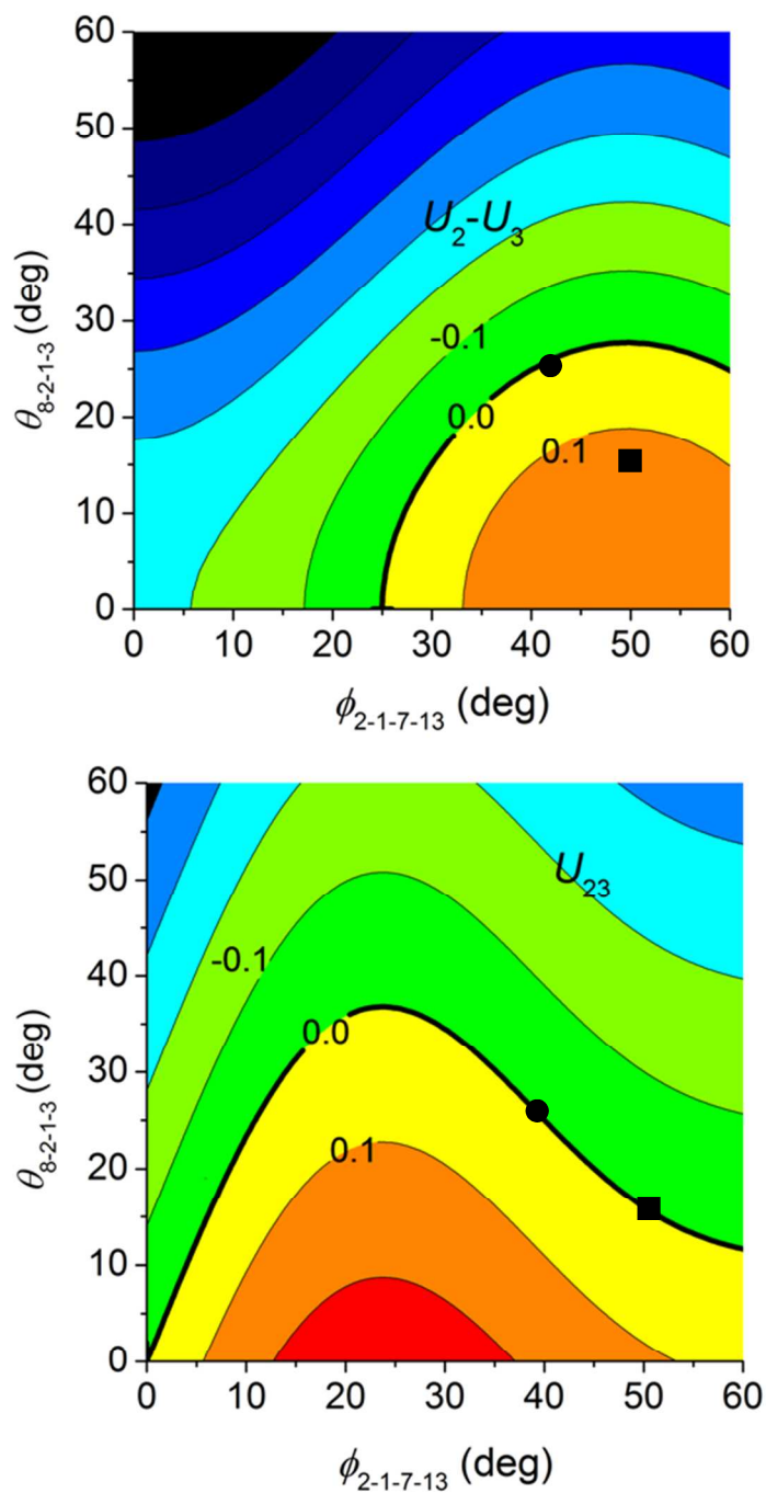
Figure 13. Contour plots of U_2 - U_3 and U_{23} (in eV) to locate the non-planar conical intersection of the {}^1\pi\pi^* and {}^1\pi\sigma^* states at r_{\text{OH}} = 1.29 \text{ \AA} . The solid square and circle are explained in Section 3.5.
