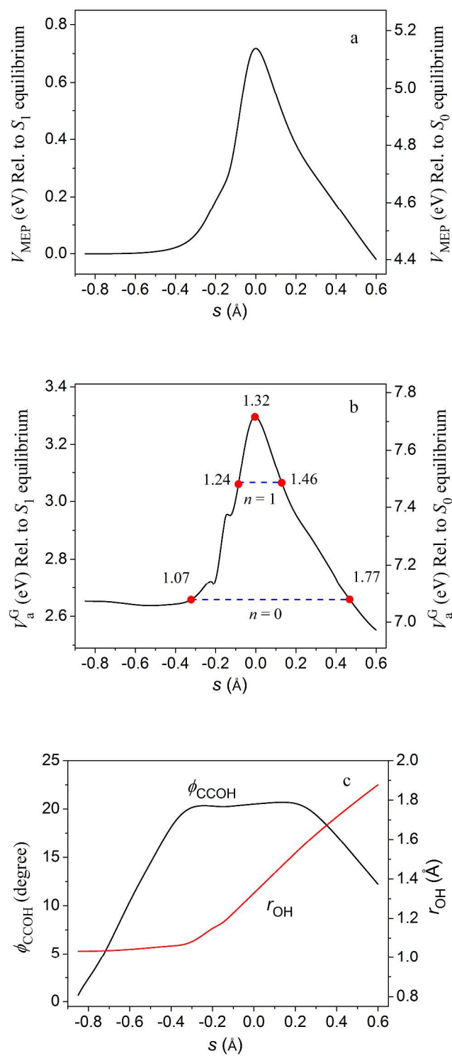
Figure 4. (a) Calculated V_{\text{MEP}} vs the reaction coordinate s (scaled to a reduced mass of one amu) for the O–H dissociation of phenol on the S_1 adiabatic surface. (b) Calculated ground-state
