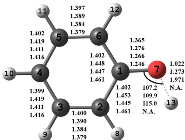
Figure 8. The figure shows the structure of MECI1 and four sets of bond distances for key eight C–C, C–O, and O–H bond lengths (in Å) and the C–O–H bond angle (in degrees). From top to bottom are values for the equilibrium geometry of the S_0 state of phenol, MECI1, MECI2, and the \tilde{X}^2B_1 state phenoxyl radical. “N.A.” denotes not applicable.
