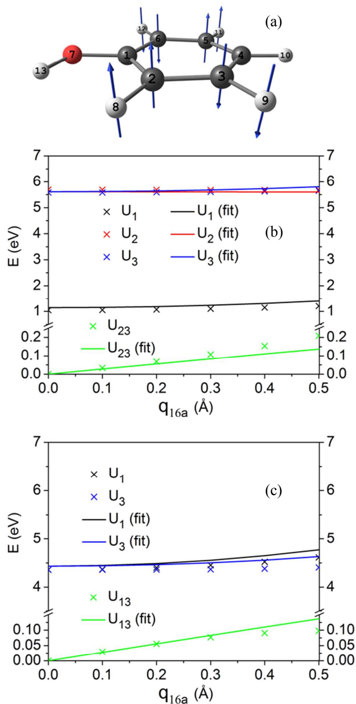
Figure 11. The atomic displacements of vibrational mode \nu_{16a} (a), and calculated and APRP diabatic potentials and the most relevant diabatic couplings at conical intersections of the {}^1\pi\pi^* and {}^1\pi\sigma^* states (b) and the {}^1\pi\pi and {}^1\pi\sigma^* states (c) along scaled Cartesian normal-mode displacements.
