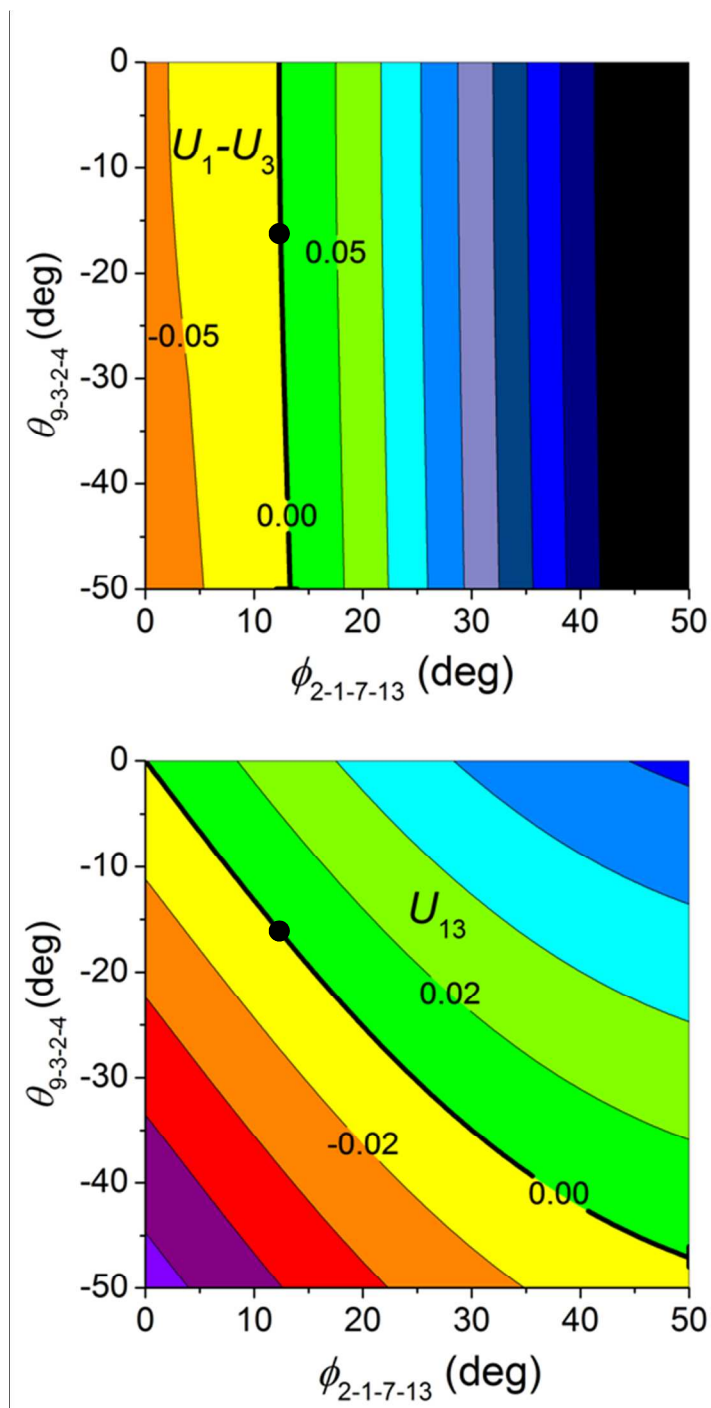
Figure 14. Contour plots of U_1 - U_3 and U_{13} (in eV) to locate the non-planar conical intersection of the ^1\pi\pi and ^1\pi\sigma^* states at r = 2.20 Å.
