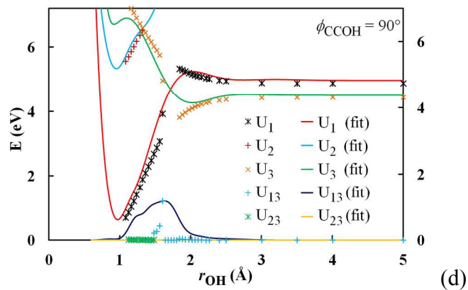
Figure 5. Calculated and APRP diabatic potentials ( U_1 , U_2 , and U_3 and U_{13} and U_{23} ) of phenol along the O–H dissociation coordinate r at various C2–C1–O–H torsion angles \phi . The other geometric parameters are fixed at their values at the equilibrium geometry of ground state phenol.
