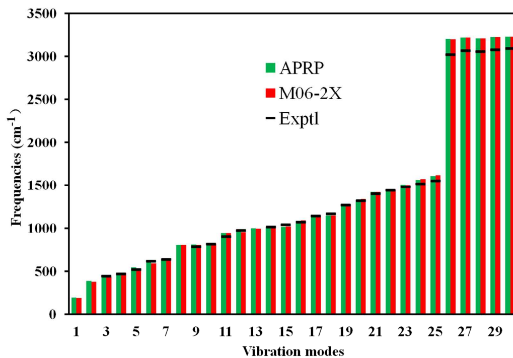
Figure 3. Comparison of vibrational frequencies calculated from the ground-state APRP surface, from M06-2X calculations with available experimental results. Top: the {}^1\pi\pi state of phenol; bottom: the \tilde{X} {}^2B_1 state of phenoxy radical.
