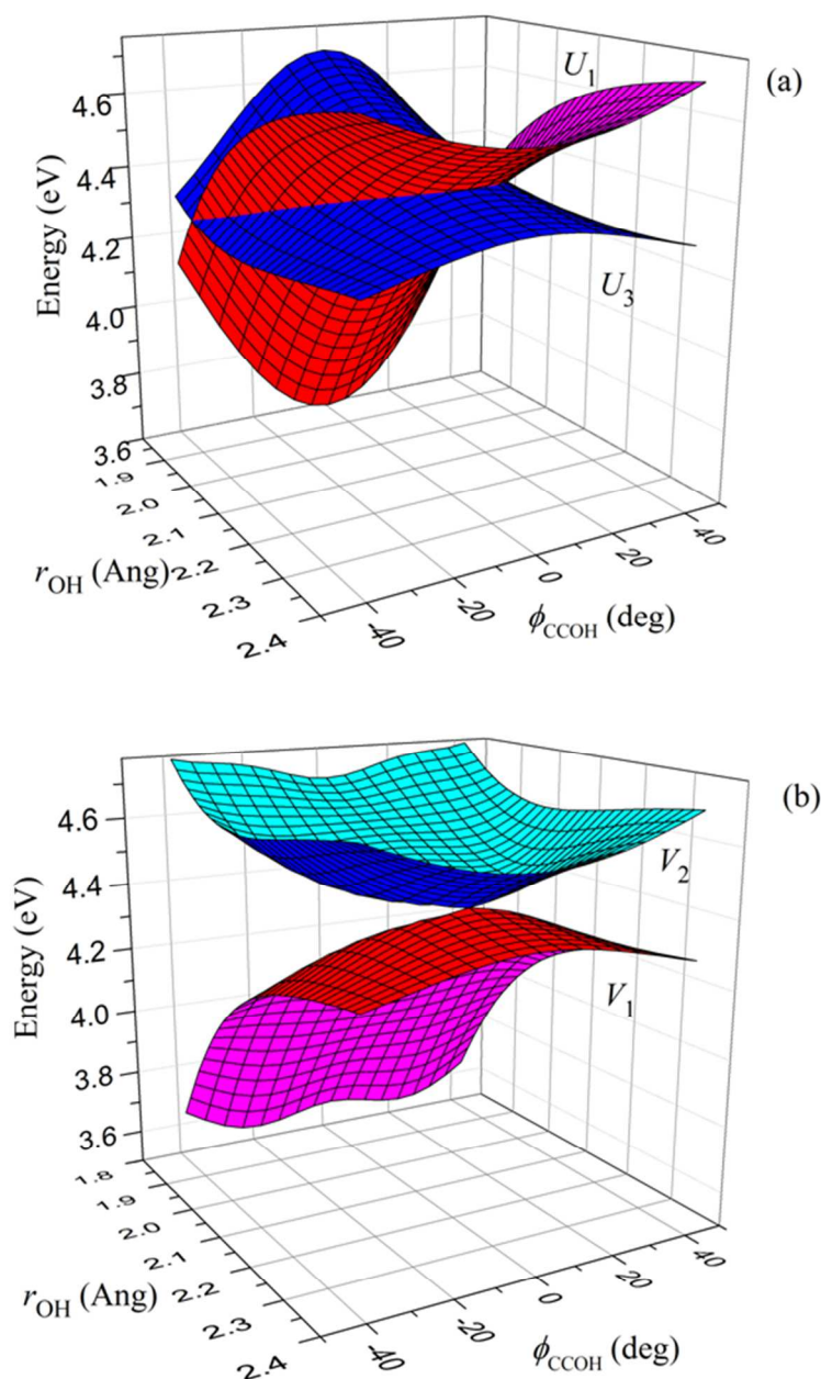
Figure 7. Three-dimensional plots of (a) the U_1 and U_3 diabatic potential-energy surfaces showing the diabatic crossing of the ^1\pi\pi and ^1\pi\sigma^* states and (b) the V_1 and V_2 adiabatic potential-energy surfaces of phenol as functions of r and \phi . The conical intersection (CI2) is seen at r = 2.23 Å and \phi = 0^\circ with all other geometric parameters fixed at the ground state equilibrium geometry of phenol.
