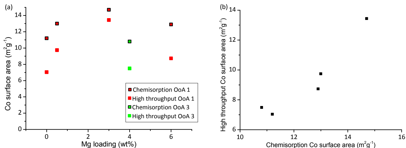
Figure 5. Cobalt surface area measurement by conventional and high-throughput methods. (a) Plot showing Co surface area measured by chemisorption directly and calculated high-throughput surface area, both of which show the same trends for the catalysts studied. High-throughput surface area is calculated from Co particle size measured by XRD (as shown in Figure 2) and reducibility measured by high-throughput TGA in 5% H 2 for samples with different Mg loadings using OoA 1 (red) and OoA 3 (green). (b) shows the same data plotted as high-throughput surface area against surface area measured by chemisorption, showing the linear correlation.
