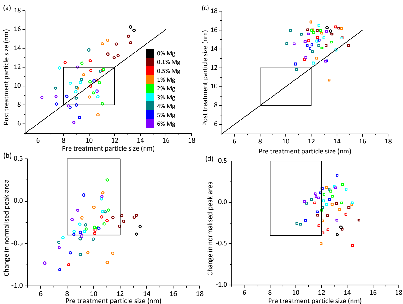
Figure 3. Particle size and peak area ratio changes on ageing treatment. (a) Particle sizes before and after ageing treatment for Mg added before Co and calcined (OoA 1), showing that smaller Co particles made by this route are not generally more prone to sintering than larger ones. Each Mg loading has 6 data points as there are three Ru loadings and two points per unique sample. Ru loadings are not distinguished in this figure as the regression analysis showed little effect of Ru loading. Versions with Ru loadings distinguished are shown in Figure S9. If points lie above the superimposed y=x line, sintering has occurred. Points below the line are likely due to error (the validation work showed a standard deviation in particle size of 1.5 nm), but could also be due to metal particle reaction with support. The box shows the hit region defined by particle sizes of 8-12 nm pre- and post- ageing treatment, (b) change in normalised Co peak area against pre-treatment particle size for OoA 1 samples, showing that smaller particles generally lose more Co peak area than larger ones. The box shows the hit region defined by pre-treatment particle size of 8-12 nm and a change in normalised Co peak area of 0 to -0.4, (c) Particle sizes before and after ageing treatment for OoA 3 showing a large degree of sintering of around 3 nm, (d) change in normalised Co peak area against pre-treatment particle size for OoA 3 samples, showing that these samples generally lose less Co peak area than OoA 1 samples, and the protective effect of Mg in this respect.
