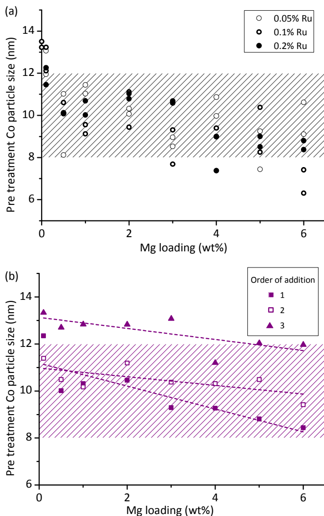
Figure 2. Control of cobalt metal particle sizes by catalyst synthesis protocol. The raw data was subjected to multiple linear regression which allows quantification of the effect of different synthesis variables: (a) shows the results of this analysis for the particle size data, showing that increasing Mg loading decreases particle size, while adding Mg before cobalt (OoA 2) reduces particle size, and calcining the support after addition of Mg reduces it further (OoA 1). The interaction between these two variables can also be seen, meaning that Mg loading has a larger effect on particle size when it is added before (OoA 1 and 2) rather than after (OoA 3) Co. (b) shows particle sizes as calculated by the Scherrer equation vs. Mg loading for samples where Mg was added to the support and calcined before Co addition (OoA1) showing that Ru loading has little effect on particle size. Hashed areas show 8 – 12 nm target particle size range.
