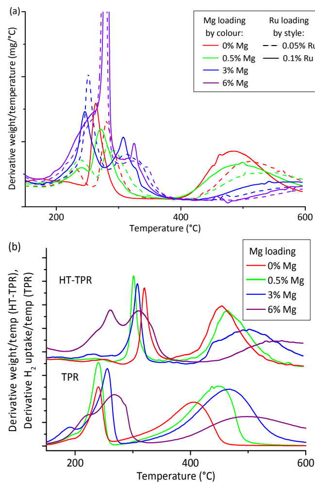
Figure 4. High-throughput TPR measurement of reducibility. (a) High-throughput TGA in 5% H 2 acts as a high-throughput TPR (HT-TPR) screen to assess reducibility for OoA 1 samples. Mg lowers reducibility while Ru increases it. (b) Comparison of HT-TPR and conventional TPR traces for the scaled up samples showing that both methods show the same features, but these are shifted around 75 °C to higher temperatures in the case of the HT-TPR traces.
