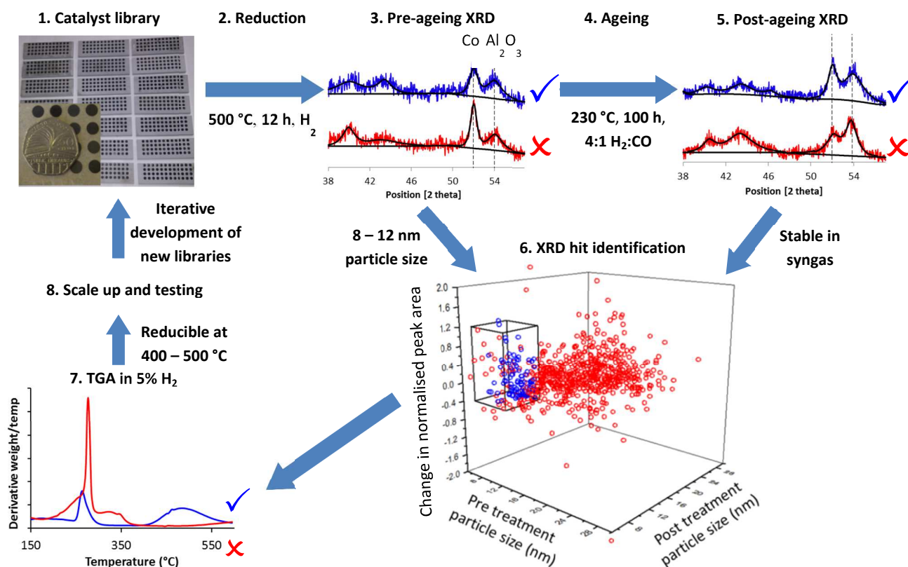
Figure 1. Accelerated discovery of stable Fischer-Tropsch catalysts. Catalyst libraries are synthesised by impregnation, producing oxides (Step 1) and reduced to form the Co metal particles in well plates (Step 2) before XRD is performed (Step 3) to measure the Co metal particle size and amount of Co metal with respect to the support. Libraries are aged in syngas (Step 4) before having XRD performed again (Step 5). Sintering and loss of metallic Co is measured by comparison of XRD before and after the ageing treatment which acts as a proxy for stability. Hits identified (Step 6) are in blue and are samples with Co particles in the range 8-12 nm before and after ageing treatment and which are stable with respect to loss of metallic Co (as measured by the difference in normalised peak area before and after treatment). XRD patterns in red are misses due to too large particle size (Step 3) and too great a loss in metallic Co (Step 5), whereas data from samples passing the individual criteria are in blue. Hits from XRD have their reducibility assessed by TGA in 5% H 2 /N 2 (Step 7). The blue trace is reducible at 400-500 °C while the red trace will be poorly reduced at 500 °C. Samples are selected for scale-up and catalytic testing (Step 8) followed by feedback to inform the design of the next library.
