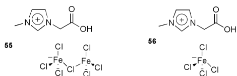
Figure 6. Ion-tagged iron catalyst used in the Biginelli reaction.
