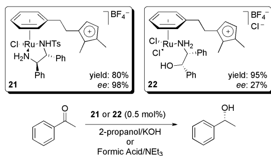
Scheme 8. Ionophilic ruthenium-complexes-catalysed transfer hydrogenation reactions.
