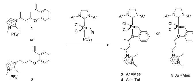
Scheme 2. Structure of CTL 1 and 2 and the synthesis of charge-tagged Hoveyda-type catalysts 3 , 4 and 5 .
