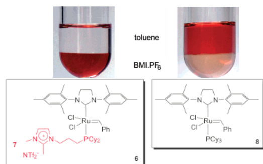
Figure 1. Comparison of the distribution of 6 and 8 in a biphasic system composed of BMI-PF 6 and toluene. Adapted from ref. 24 .
