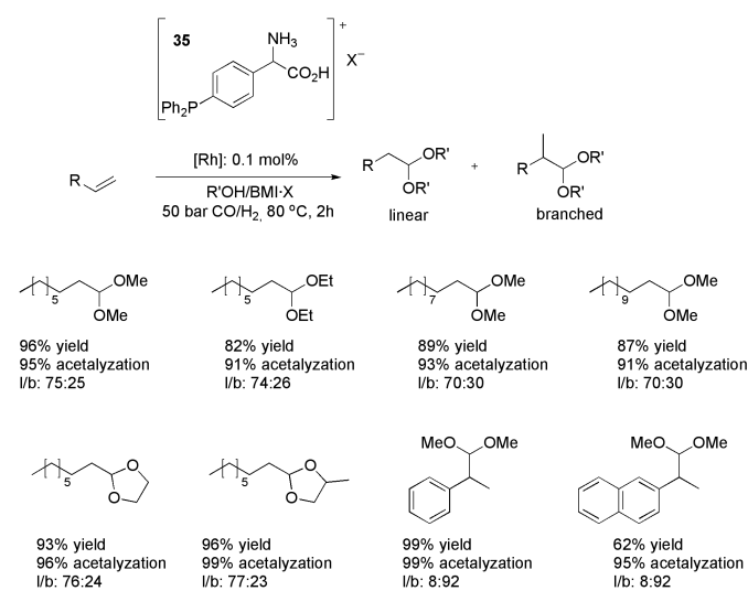
Scheme 16. CTL 35 applied in rhodium-catalysed tandem hydroformylation/acetalization of olefins in ionic liquid/alcohol media.
