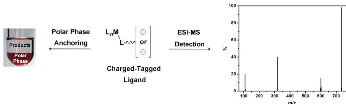
Scheme 1. CTLs for polar-phase anchoring and ESI-MS detection.
