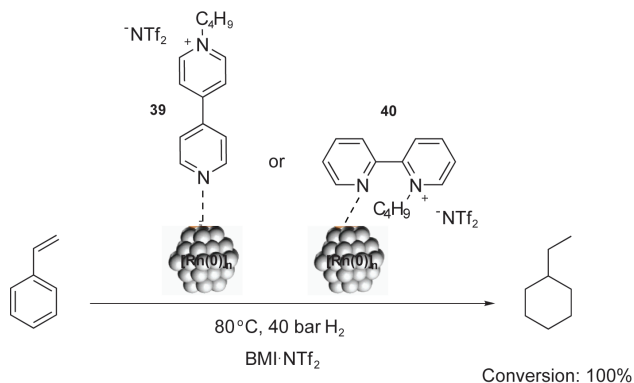
Scheme 18. Hydrogenation of styrene catalysed by [\text{Rh}(0)]_n NPs, which are stabilised by bipyridinium CTLs 39 and 40 .
