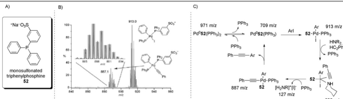
Scheme 28. A) Structure of monosulfonated triphenylphosphine ( 52 ). B) ESI(-)-MS of \text{Pd}(\text{PPh}_3)_4 + [\text{PPN}][\mathbf{52}] + 100 \times (\text{PhI} + \text{PhC}_2\text{H} + \text{NEt}_3) in \text{CH}_2\text{Cl}_2 . Inset: isotope pattern match for [\text{Pd}(\mathbf{52})(\text{PPh}_3)(\text{Ph})(\text{C}_2\text{Ph})] . C) Intermediates that were directly observed by ESI(-)-MS and the proposed catalytic cycle.
