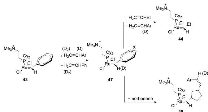
Scheme 22. Reaction of electron-sprayed intermediate 43 with substituted styrenes, generating 47 and subsequently 44 and 48 .
