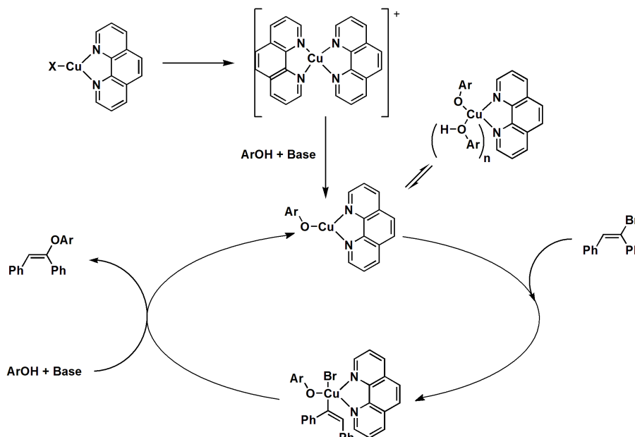
Scheme 25. Catalytic cycle proposed for the copper-catalysed vinylation of phenols.
