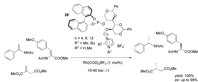
Scheme 12. Mannitol-based charge-tagged monophosphites that were used as ligands in the rhodium-catalysed hydrogenation of olefins.
