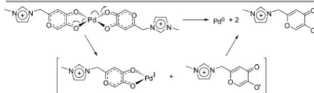
Scheme 27. Proposed Pd-reduction by ligand decomposition.
