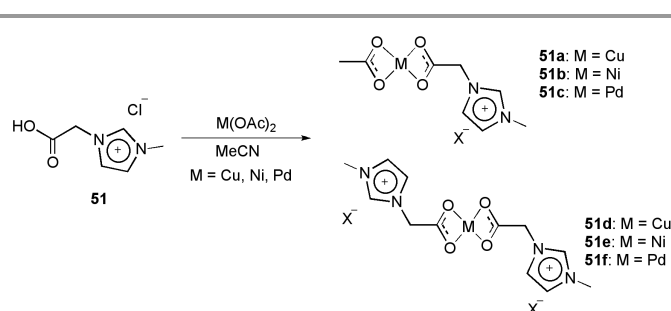
Scheme 26. Reaction of charge-tagged carboxylate ligand 51 with Cu(OAc)_2 , Ni(OAc)_2 and Pd(OAc)_2 , generating the corresponding mono- and dicationic charge-tagged metal complexes.
