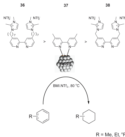
Scheme 17. Hydrogenation of arenes, catalysed by [\text{Rh}(0)]_n NPs stabilised by CTLs in ILs, and the activity observed for the different ligands.
