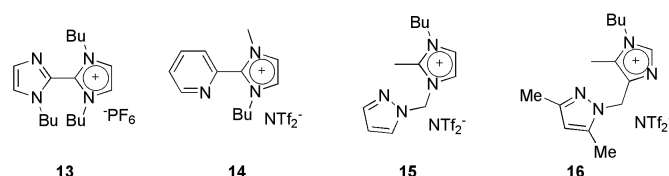
Figure 2. CTLs used as the solvent/ligand in palladium-catalysed cross-coupling reactions.
