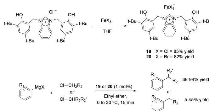
Scheme 7. Synthesis of ionic Iron-benzimidazole complexes and its application in cross-coupling of aryl-Grignard reagents with alkyl halides.
