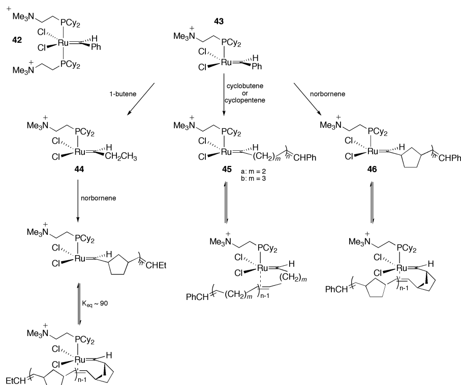
Scheme 21. CTLs in ESI-MS detection of olefin metathesis intermediates.
