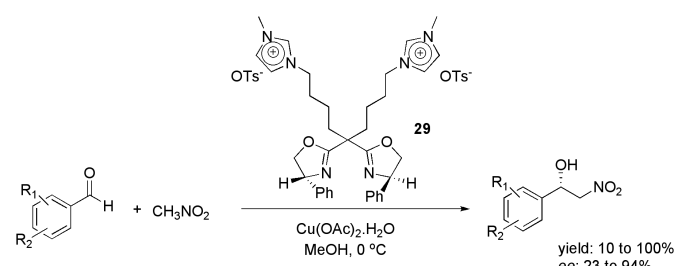
Scheme 13. Imidazolium-tagged bis(oxazoline) ligand that was used in the copper-catalysed, asymmetric Henry reaction.
