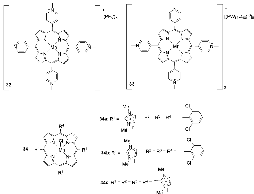
Figure 3. Manganese porphyrins that were used in oxidation reactions.
