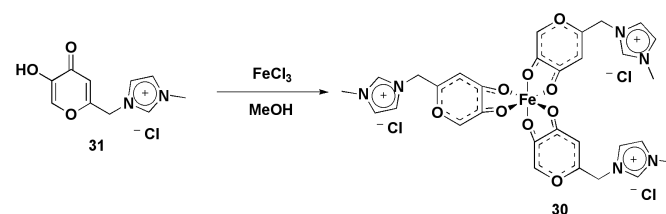
Scheme 14. Fe(III) complex bearing imidazolium moieties that was applied in olefin epoxidation reactions.
