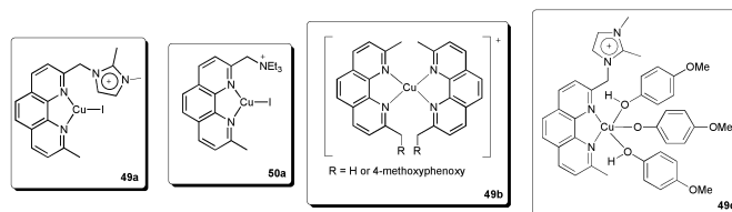
Figure 4. Intermediates detected in ESI(+)-MS.
