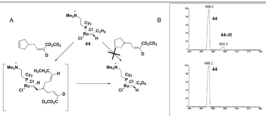
Scheme 23. A) Reaction of 44 with 4-[[Z]-2-pentenyl-3,4,4,5,5-d6]-cyclopentene or 4-[[Z]-2-pentenyl-3,4,4,5,5-d6]-cyclopentane. B) Top: ESI(+)-MS spectra of the reaction of 44 with a cyclopentene derivative, with the detection of 44-d6 . Bottom: ESI(+)-MS spectra of the reaction of 44 with a cyclopentane derivative, with no detection of 44-d6 .
