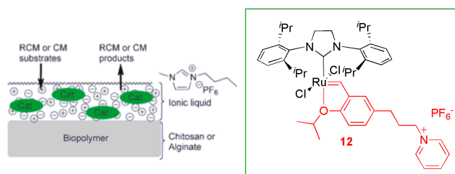
Scheme 4. Schematic representation of the ruthenium bio-SILP.
