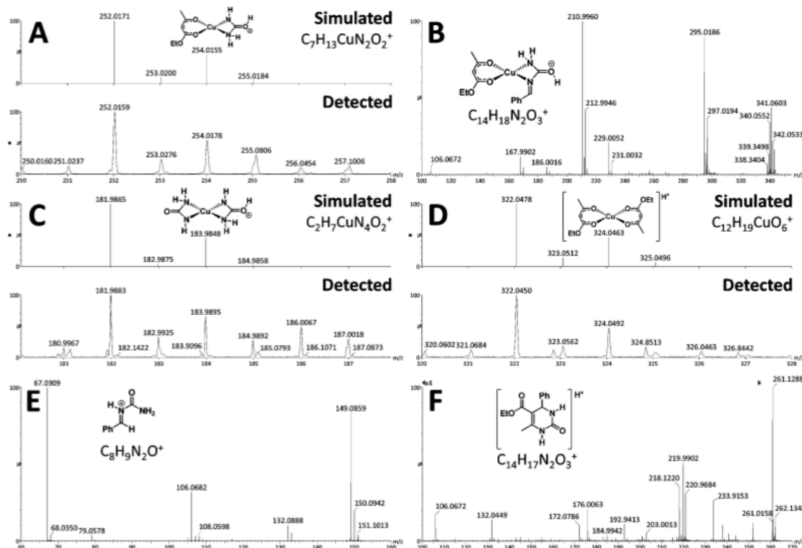
Figure 5. Key intermediates and products detected (and characterised) by ESI(+)-MS(/MS): A) ESI(+)-MS of [I + H] + ; B) ESI(+)-MS/MS of [III + H] + ; C) ESI(+)-MS of [V + H] + ; D) ESI(+)-MS of [VI + H] + ; E) ESI(+)-MS/MS of the key Biginelli reaction intermediate [A + H] + , i.e., the so-called iminium intermediate; F) ESI(+)-MS/MS of the Biginelli adduct [DHPM + H] + .
