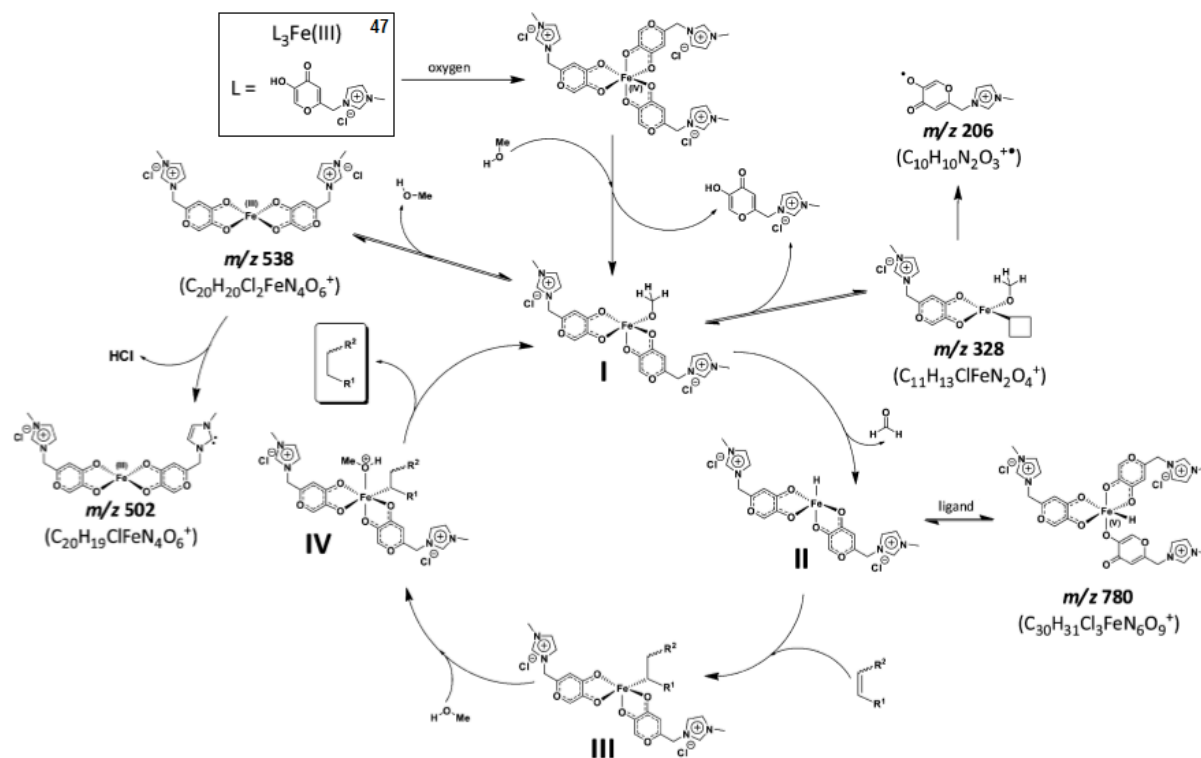
Scheme 30. Proposed catalytic cycle for olefin reduction catalysed by 54 in the presence of methanol. Major ions detected in ESI(+)-QTOF-MS experiments are indicated by their m/z values, and proposals for the origins of the intermediates are shown.
