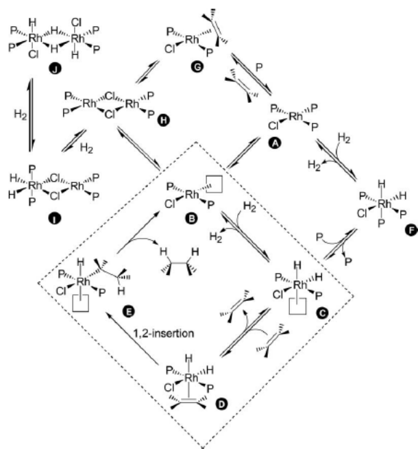
Scheme 29. Catalytic cycle of \text{RhCl}(\text{PPh}_3)_3 -catalysed hydrogenation of olefins.
