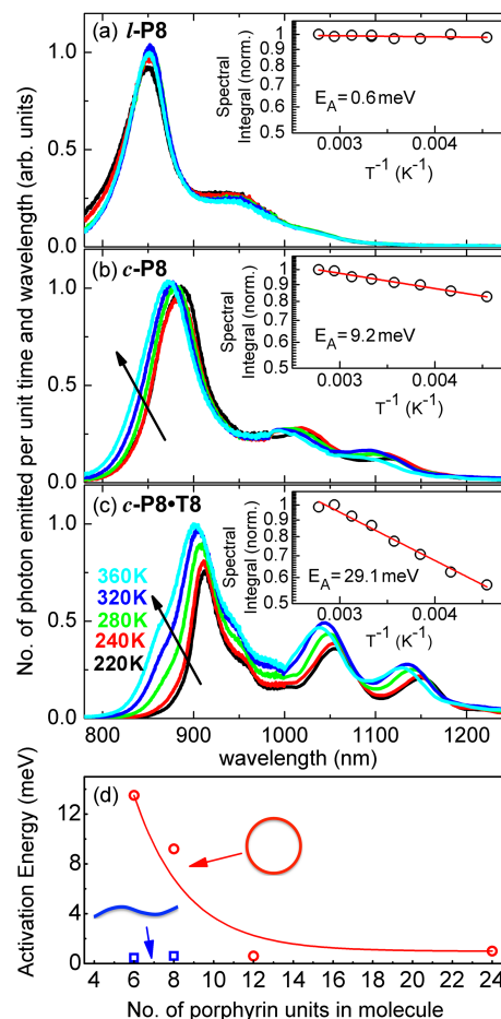
Fig. 7. Steady-state PL spectra for (a) l -P8, (b) c -P8 in toluene/1% pyridine and (c) c -P8·T8 in toluene, at solution temperatures of 220 K (black line), 240 K (red), 260 K (green), 320 K (blue) and 360 K (cyan). The insets show the spectral integral over these spectra (which is proportional to the total number of photons emitted from the sample) as a function of inverse temperature. From these data, the shown activation energy E_A for thermally enhanced emission was extracted through exponential fitting. (d) Plot of the activation energy, E_A , as a function of the number of porphyrins in the molecule for non-templated, cyclic (open circles) and linear porphyrin oligomers (full squares). Lines are guides to the eye.
