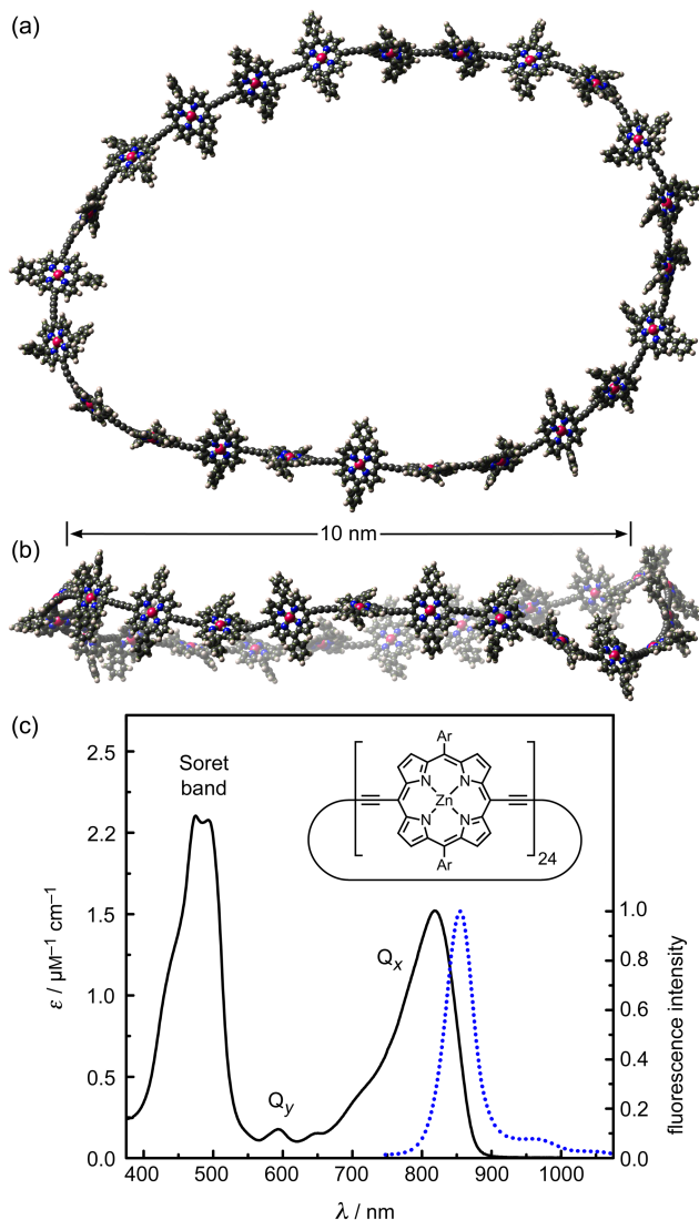
Fig. 1. (a) and (b) Two orthogonal views of a snapshot of c-P24 from a molecular dynamics simulation at 300 K (using the MM+ force field implemented in HyperChem). (c) Molar extinction (black line) and normalized photoluminescence (blue dashed line) spectra at 295 K of c-P24 cyclic porphyrins in toluene/1% pyridine. The emission was recorded after excitation at 770 nm (1.61 eV). The insert shows the chemical structure of c-P24 (Ar = 3,5-bis(octyloxy)phenyl).
