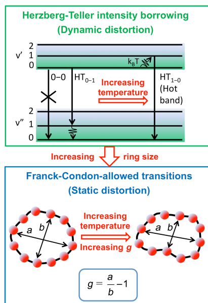
Fig. 6. Schematic diagram illustrating the processes leading to coupled electronic-vibrational transitions in porphyrin nanorings. Large rings are more flexible, and hence static distortions from symmetry yield lowest vibronic transitions that are allowed within the standard Franck-Condon approximation. For small rings, Herzberg-Teller intensity borrowing from higher-lying allowed transitions yields emission from the lowest state through involvement of a non-totally symmetric vibration quantum.
