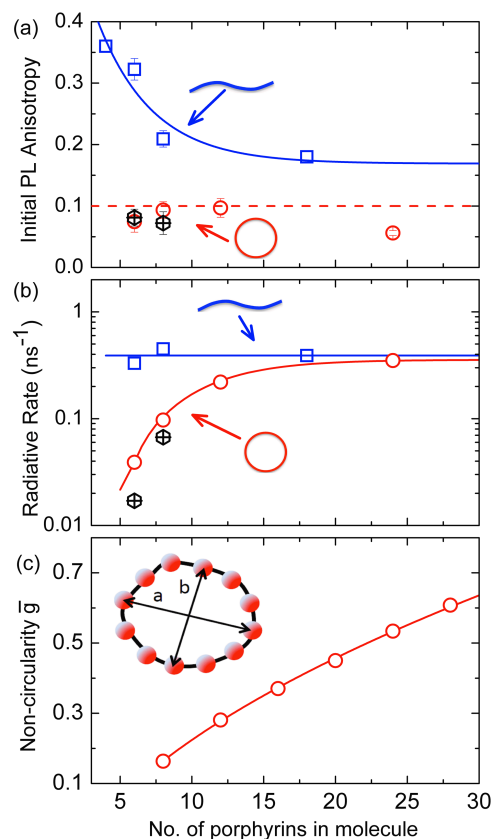
Fig. 5. (a) Initial PL polarization anisotropy within the first few hundred femtoseconds after excitation at 770 nm, as a function of the number of porphyrins contained in the molecule, for free nanorings (red open circles), template-bound nanorings (black crossed hexagons) and linear oligomers (blue open squares) in solution. (b) Radiative transition rate as a function of the number of porphyrins. The transition rates for free porphyrin nanorings, template-bound porphyrin nanorings and porphyrin linear oligomers are represented by the red open circles, black crossed hexagons and blue open squares, respectively. (c) Ensemble-averaged deviation \bar{g} = \langle \frac{a}{b} - 1 \rangle of nanorings from circularity, where a and b are the long and short axes of each nanoring. \bar{g} was determined from Monte Carlo modeling at 290 K as described in the main text, using parameters defined by correlation with conformations observed in STM images. All lines are guides to the eye.
