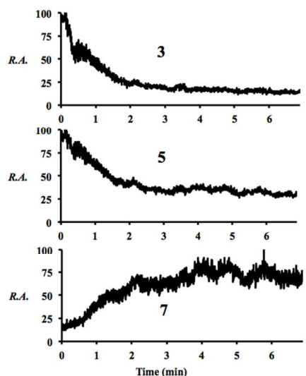
Figure 2 Chronograms showing relative abundances of compounds 3 , 5 , and 7 as the temperature is increased from room temperature to 80°C (~3 min) at l = 30 cm.
