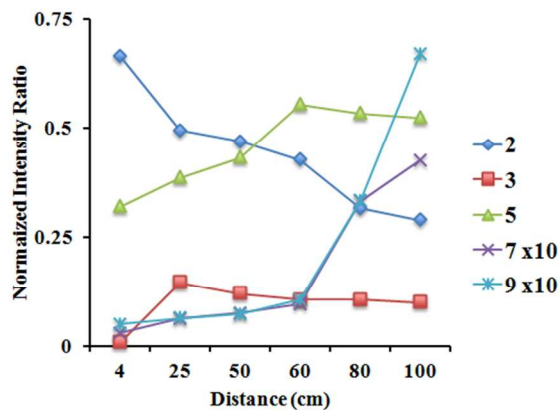
Figure 3 Progress of the off-line cold surface reaction at various distances between the ESI source and the collection surface under conditions where reaction at the surface is minimized by operating at low temperature.
