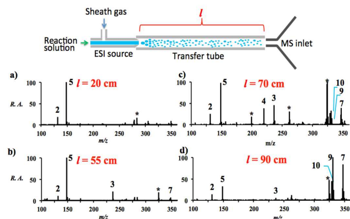
Figure 1 Extent of reaction as a function of distance ( l ) between the MS inlet and the spray source. The data are accounted for by desolvation to give smaller more rapidly reacting droplets. *denotes known impurities thought to be from the guiding tube.
