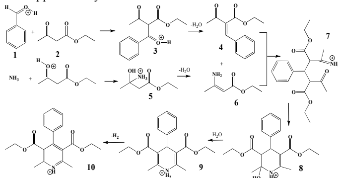
Scheme 1 Knoevenagel condensation product ( 4 ) reacts with the enamine ester ( 6 ) via a Michael addition to form 7 , which undergoes proton transfers and intramolecular enamine formation to give 9 . In a separate step, dehydrogenation yields the pyridine ( 10 ). All species are shown in their charged forms where appropriate.
