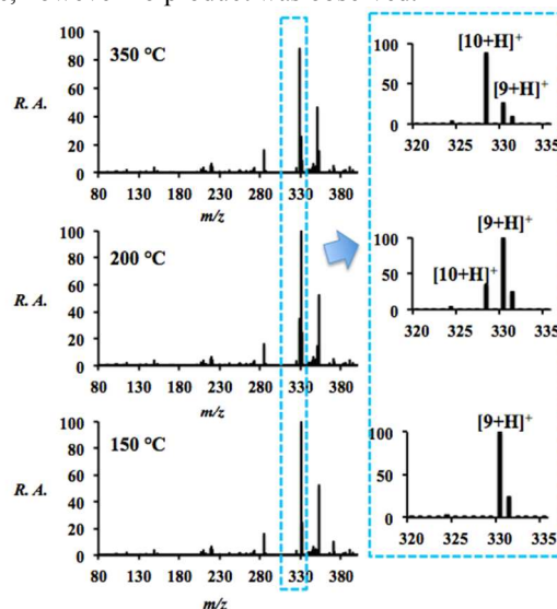
Figure 4 On-line reaction ( l = 100 cm) at various ion transfer capillary temperatures. Spectra on the right are expansions showing 9 and 10 . Note that 9 and 10 occur as protonated, sodiated, and potassiated forms. The signal at m/z 282 is due to background.
