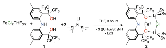
Scheme 1. Synthesis of the square-planar S = 2 complex 2 . Sv: THF, Et 2 O
