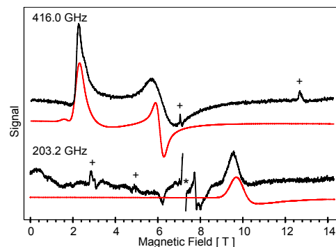
Figure 3. High-field EPR spectra recorded at 5 K for 2 brown, at 416.0 (top) and 203.2 GHz (bottom). The solid red traces are simulations obtained for a S = 2 with D = 17.4 \text{ cm}^{-1} , E/D = 0.14 , g_x = 2.19 , g_y = 2.18 and g_z = 2.04 . The features marked by (+) account for the molecular \text{O}_2(\text{g}) adsorbed on the surface of the sample containers. The resonance marked by (*) appears at g = 2.0023 and arises from a radical contaminant.
