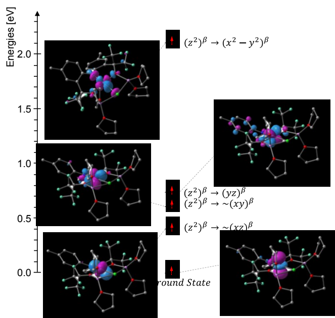
Figure 6. Molecular orbital diagram derived from the TD-DFT calculations.
