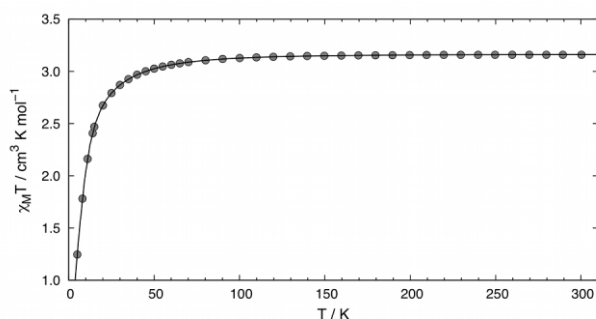
Figure 2. Temperature dependence of \chi_M T for 2 measured using an applied field of 0.1 T. The line depicts the fit obtained using |D| = 20.9(4) \text{ cm}^{-1} , g = 2.05(3) , and \Theta = 0.8 \text{ K} .
