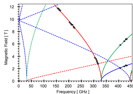
Figure 4. Black dots mark the field and frequency dependencies of the prominent resonances observed for the low-temperature, high-field EPR spectra of microcrystalline brown 2 . The solid lines account for the ground state resonances and the dotted lines account for the excited state resonances. The red, blue and green colors mark the z , y and x molecular orientations, respectively.
