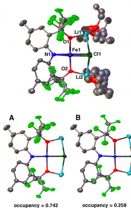
Figure 1. Molecular structure, refined into parts A and B , with ellipsoids presented at 50% probability level. Hydrogen atoms were removed for clarity. Selected bond lengths ( \text{\AA} ) for A : Fe1-N1: 1.9704(19) , Fe1-Cl1: 2.3888(9) , Fe1-O1: 1.9261(19) , Fe1-O2: 2.0174(18) and for B : Fe1-N1: 1.960(2) , Fe1-Cl1: 2.338(3) , Fe1-O1: 2.113(2) , Fe1-O2: 1.848(2) .
