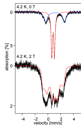
Figure 7. ^{57}\text{Fe} Mössbauer spectra recorded at 4.2 K in 0 T (top) and 2 T (bottom) for a 5.4 nM ^{57}\text{Fe} enriched solution sample of 2 . The solid red lines are simulations obtained using the same parameters as for 2 brown in the solid state.
