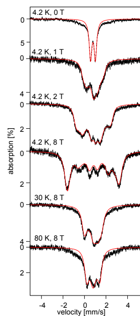
Figure 4. Black dots mark the field and frequency dependencies of the prominent resonances observed for the low-temperature, high-field EPR spectra of microcrystalline brown 2 . The solid lines account for the ground state resonances and the dotted lines account for the excited state resonances. The red, blue and green colors mark the z , y and x molecular orientations, respectively.
