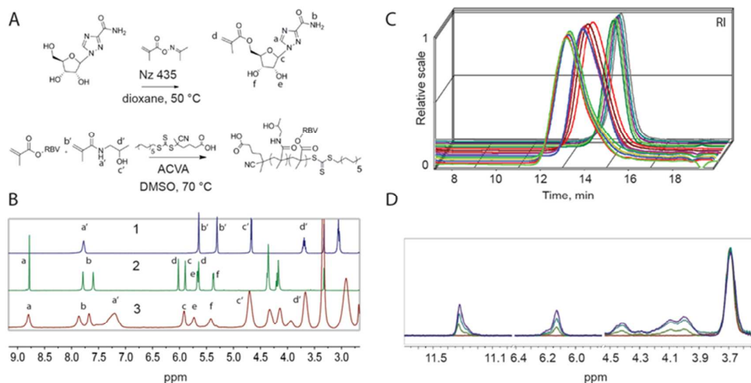
Figure 1. (A) Schematic illustration of the synthesis of RBV methacrylate and macromolecular prodrugs for RBV based on HPMA. (B) 1 H NMR ( d 6 -DMSO) spectra for HPMA (1), RBV methacrylate (2), and a representative MP (3) with the peaks at 5.4 and 5.7 ppm being the hydroxyls of RBV. (C) Size exclusion chromatography elution profiles for 15 representative polymers comprising polymer series with target degree of polymerization (left to right) 260, 150, and 50 (non-fluorescent series with [M]/[RAFT] 500, 250 and 50). (D): the superimposition of 1 H NMR spectra (D 2 O) showing increasing RBV loading within one set of polymers with having a narrow mass range of 5–6 kDa with RBV loading increasing from 0% to 23 mol%. The signals stemming from RBV (3.9–4.5, 6.1–6.2, 11.2–11.4 ppm) are normalized to a signal from the PHPMA carrier (3.7 ppm).
