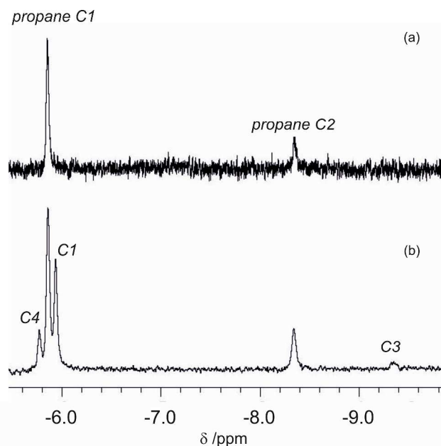
Fig. 5. ^1\text{H} NMR spectrum in the high-field region obtained after 355 nm laser irradiation of (a) \text{CpMn}(\text{CO})_3 in liquid propane; (b) a 60:40 mixture of liquid propane and isopentane at 133 K. The labels indicate the positions of Mn coordination for propane (above) and isopentane (below).
