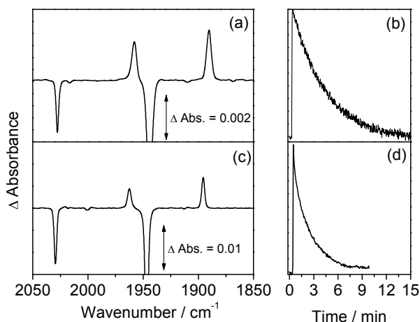
Fig. 3. Rapid-scan FTIR difference spectra obtained 2 s after 355 nm photolysis of CpMn(CO) 3 at 135 K in (a) isopentane and (c) liquid ethane. Kinetic traces showing decay of (b) the Mn-isopentane complex at 1958 cm -1 and (d) the Mn-ethane complex at 1962 cm -1 .
