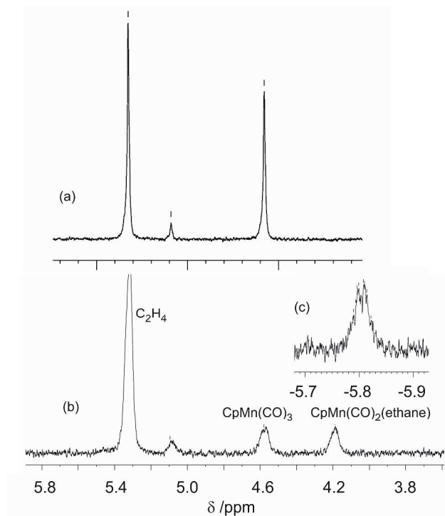
Fig. 4. (a) ^1\text{H} NMR spectrum of \text{CpMn}(\text{CO})_3 in ethane prior to irradiation in cyclopentadienyl region (b) spectrum after 355 nm laser irradiation. (c) inset showing high field region after irradiation.
