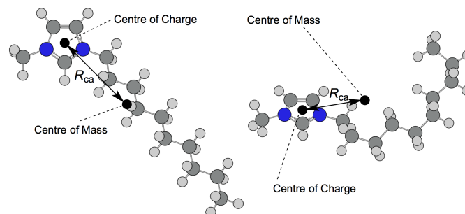
Fig. 9 Schematic diagram representing the dramatic influence of ion geometry on the ‘charge arm’, R_{ca} , using the example of the 1-decyl-3-methylimidazolium cation, [\text{C}_{10}\text{C}_1\text{im}]^+ , in both an ‘extended’ all-anti conformer (left), R_{ca} = 4.49 Å, and ‘coiled’, part-gauche conformer (right), R_{ca} = 3.64 Å.
