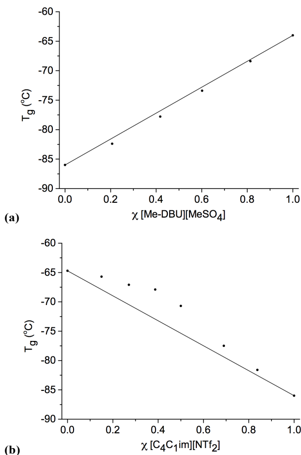
Fig. 4 Glass transition temperatures ( T_g ) for ionic liquid mixture series: (a) [\text{C}_4\text{C}_1\text{im}][\text{Me-DBU}][\text{MeSO}_4][\text{NTf}_2] , 10 ; (b) [\text{C}_4\text{C}_1\text{im}][\text{NTf}_2][\text{Me}_2\text{PO}_4] , 7 .
