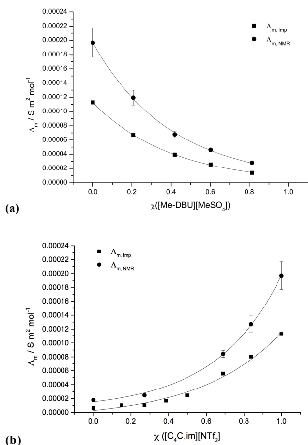
Fig. 6 Conductivities of binary and reciprocal binary ionic liquid mixture series, both from impedance spectroscopy, \Lambda_{m,Imp} , and from the self-diffusion coefficients, \Lambda_{m,NMR} : (a) [C_4C_1im][Me-DBU][MeSO_4][NTf_2] , 10 ; (b) [C_4C_1im][NTf_2][Me_2PO_4] , 7 .
