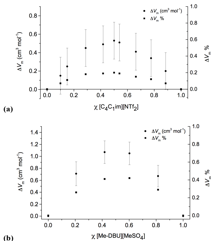
Fig. 3 Excess molar volumes, represented as absolute values, \text{cm}^3 \text{ mol}^{-1} , and as % relative to the expected molar volume: (a) [\text{C}_4\text{C}_1\text{im}][\text{Me}_2\text{PO}_4][\text{NTf}_2] , 7 ; (b) [\text{C}_4\text{C}_1\text{im}][\text{Me-DBU}][\text{MeSO}_4][\text{NTf}_2] , 10 .
