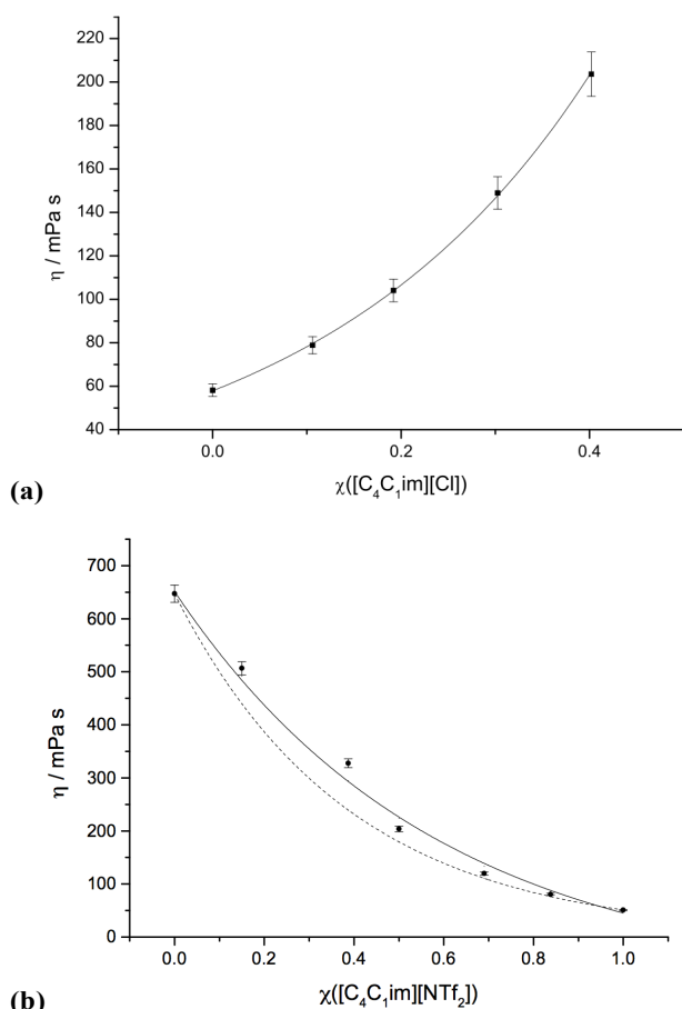
Fig. 5 Viscosities of mixture series: (a) [C 4 C 1 im]Cl[OTf], 1 ; (b) [C 4 C 1 im][NTf 2 ][Me 2 PO 4 ], 7 . The dashed line in (b) represents the ideal Katti and Chaudhri mixing law (equation 2), continuous lines include the additional ' f ' non-ideality parameter of Grunberg and Nissan (equation 3).
