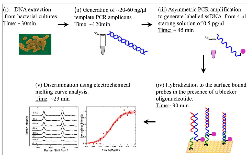
Figure 1: Schematic flow diagram of the SERS detection assay illustrating each operational step involved. First, the DNA is extracted from bacterial cultures and the amplified DNA product is used as a template to generate single stranded labelled DNA during asymmetric PCR. The step (ii) could be omitted for future assays as it is possible to perform asymmetric PCR on genomic DNA directly. 31 The labelled target is then hybridized to surface bound probes in the presence of a blocker oligonucleotide. Following electrochemical analysis monitored by SERS the pathogenic strains can be discriminated on the basis of the differences in their melting potential.
