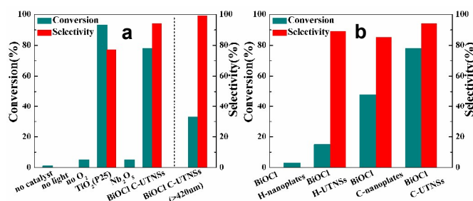
Fig. 4. Photocatalytic aerobic oxidation of 1a using different (a) semiconductor catalysts and (b) BiOCl materials. Reaction conditions: catalyst (0.077 mmol), substrate (0.1 mmol), \text{CH}_3\text{CN} (4 mL), \text{O}_2 atmosphere, 1 h, Xe lamp irradiation.
