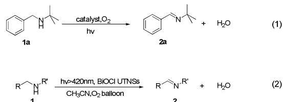
Scheme 2 Photocatalytic reactions of different secondary amines to imines.
