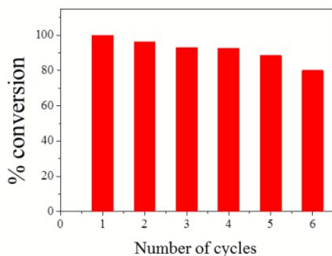
Figure 4. Catalytic recyclability of CalB@cap for the transesterification of 1 and 2 in acetone. The catalyst was removed following 8 hrs of reaction and conversion to 3 calculated by ^1\text{H} NMR for each cycle.
