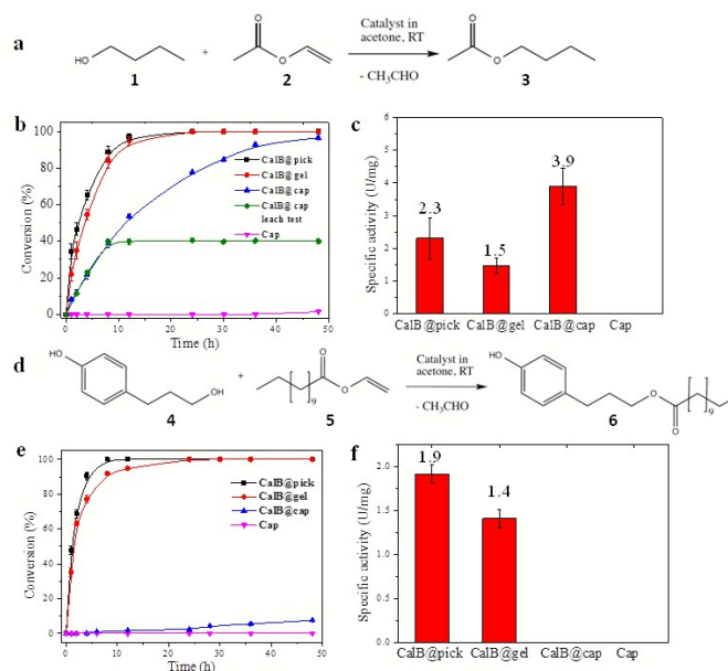
Figure 3. Biocatalysis using CalB loaded MOF microcapsules. (a) Reaction scheme for the transesterification between 1-butanol ( 1 ) and vinyl acetate ( 2 ) to yield butyl acetate ( 3 ); (b) Observed time dependent conversion of 1 and 2 catalyzed by CalB under different conditions; (c) Normalized activities ( U = \mu\text{mol}\cdot\text{min}^{-1} ) of the capsules and controls for the formation of 3 ; (d) Scheme of transesterification between 3-(4-hydroxyphenyl) propan-1-ol ( 4 ) and vinyl laurate ( 5 ) to yield 3-(4-hydroxyphenyl)propyl dodecanoate ( 6 ). (e) Observed time dependent conversion of 4 and 5 catalyzed by CalB under different conditions; (f) Normalized activities of the capsules and controls for the formation of 6 .
