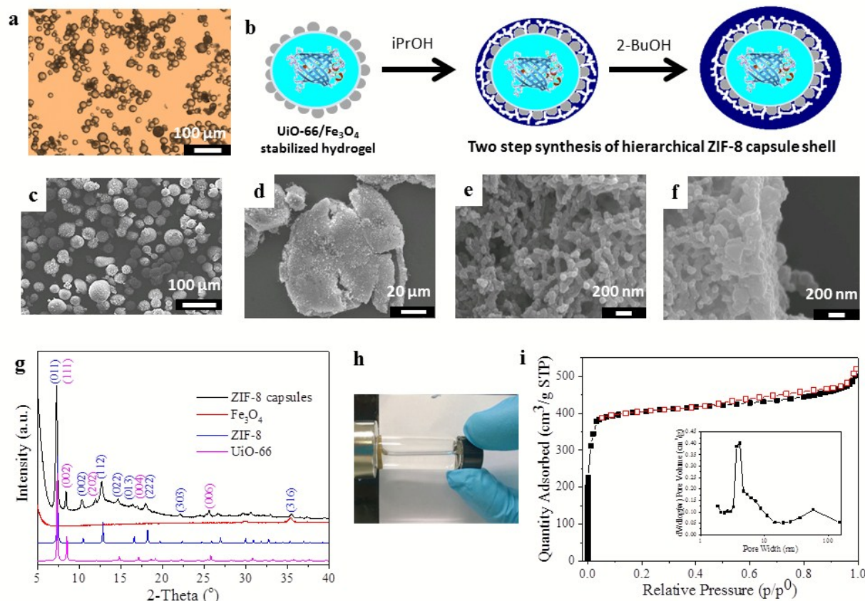
Figure 1. Synthesis and characterization of the magnetic MOF microcapsules. (a) Optical microscopy image of agarose hydrogel droplets Pickering-stabilized by UiO-66/Fe 3 O 4 nanoparticles; (b) idealized representation of the two-step synthesis protocol to form the ZIF-8 shell, (c) SEM image of the intact capsules and (d) the crushed sample, showing their hollow nature and hierarchically structured shell comprising of (e) a network-like interior and (f) a dense outer-layer of ZIF-8; (g) PXRD data of the microcapsules compared to the single components, revealing the presence of both MOFs; (h) demonstration of the magnetic recovery of the capsules; (i) Nitrogen adsorption-desorption isotherm of the capsules at 77 K (black squares, adsorption; red squares, desorption). The inset shows the BJH pore size distribution calculated from the adsorption branch of the isotherm.
