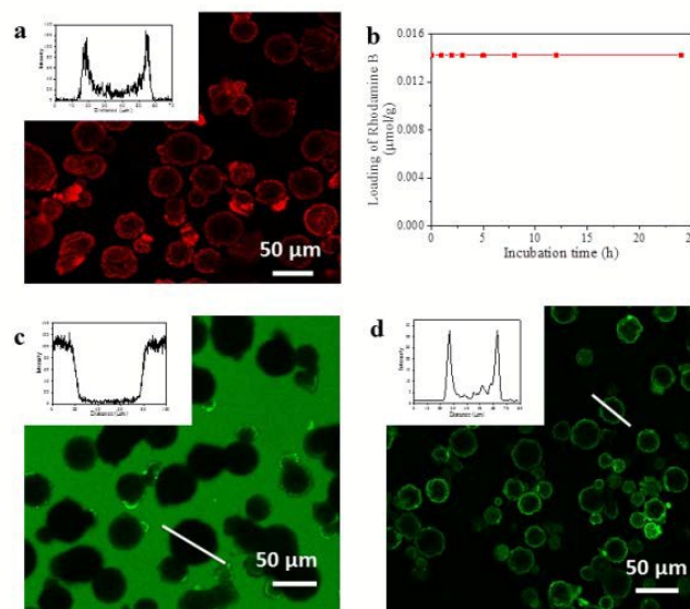
Figure 2. Encapsulation properties of the MOF composite microcapsules. (a) CLSM image of capsules loaded with RhB, and inset a typical fluorescence profile; (b) RhB retention vs. capsule incubation time in water at ambient temperature; (c) CLSM image and fluorescence intensity profile of the highlighted capsule (inset) after soaking capsules in methanolic solutions of FITC; (d) CLSM image of the capsules loaded with FITC-labelled CalB, and inset the fluorescence profile of the highlighted capsule.
