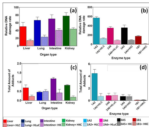
Fig. 3 DNA damage rates and amounts of adducts from 2-AAF. Top panel - Relative DNA damage rate ( \{\mu\text{g of protein}\}^{-1} \text{s}^{-1} \text{mM}^{-1} ) from ECL arrays exposed to 250 \mu\text{M} of 2-AAF in pH = 7.4 for (a) human organ tissue fractions, (b) cyt P450 supersomes. Bottom panel - Total amount of DNA adducts found (pmol \{\mu\text{g of protein}\}^{-1} \{\text{mM of 2-AAF}\}^{-1} ) after reactions with 250 \mu\text{M} 2-AAF at pH = 7.4 for 4 hrs, (c) human organ microsomes, (d) cyt P450 supersomes. The ECL images and single reaction monitoring LC-MS/MS chromatograms are in SI file (Figure S4 and Figure S7).
