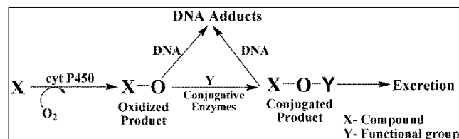
Scheme 3 Simplified metabolic pathways of drugs and chemicals in humans (X) representing oxidative metabolism and conjugative metabolism to facilitate excretion, which can result in DNA adducts due to reactions of nucleobases with reactive intermediates.
