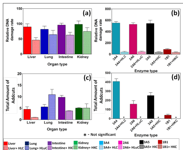
Fig. 4 DNA damage rates and adduct amounts from styrene. Top panel - 20 Relative DNA damage rate ( \mu\text{g of protein}^{-1} \text{ s}^{-1} \text{ mM}^{-1} ) from ECL arrays exposed to 1 mM of styrene in pH = 7.4 for (a) human organ tissue enzymes, (b) cyt P450 supersomes. Bottom panel - Total amount of DNA adducts found (pmol \{\mu\text{g of protein}^{-1} \text{ mM of styrene}\}^{-1} ) after reactions with 1 mM of styrene at pH = 7.4 for 1 hr, (c) human organ microsomes, 25 (d) cyt P450 supersomes. The ECL images and single reaction monitoring LC-MS chromatograms are in SI file (Figure S5 and Figure S8).
