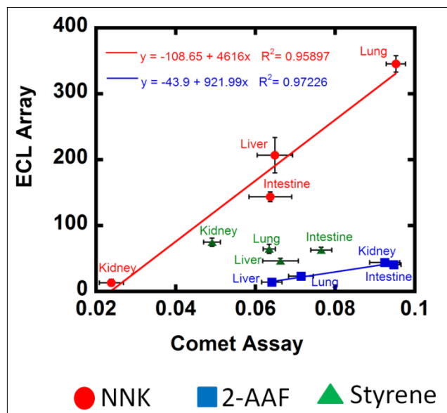
Fig. 5 Correlation plots of relative DNA damage rate from ECL arrays ( \mu\text{g of protein}^{-1} \text{ s}^{-1} \text{ mM}^{-1} ) using microsomal and cytosolic enzymes with comet assay tail migration ( \text{hr}^{-1} ) for test compounds on human cell lines from liver, lung, intestine and kidney.
