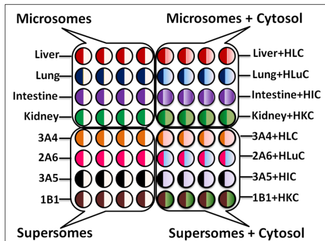
Scheme 2: Experimental design of 64-nanowell ECL chip with films of enzymes/Ru II PVP/DNA for metabolic toxicity assays of test compounds. Symbols: HLC, H=human, L=liver, C= cytosol, Lu-lung, I=intestine, K=kidney, number-letter such as 3A4 indicate supersomes containing the denoted single cyt P450 manifold.
