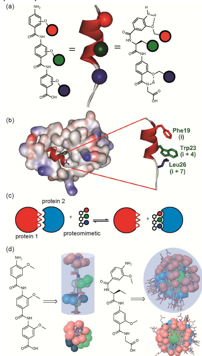
Figure 1 (a) Schematic representing the design of a hybrid \alpha -helix mimetic (right) and its comparison with an O-alkylated benzamide mimetic (left) and an \alpha -helix (middle). (b) p53/ hDM2 PPI with expansion on the native p53 peptide (PDB ID: 1YCR). (c) Schematic illustrating the process of PPI inhibition with a proteomimetic. (d) Investigation of the accessible conformational space (shown as a shaded 3D object) highlighting the orientation of the side chains (shown in CPK format): side (top left) and top (bottom left) view of a 3-O-alkylated trimer; side (top right) and top (bottom right) view of a hybrid mimetic. ( i , i + 4 and i + 7 side chains together with residues that mimic them are shown in red, green and blue respectively)
