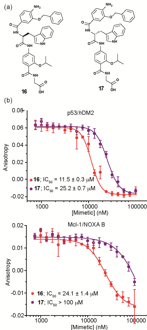
Figure 6 (a) Chemical structure of the Trp-functionalised hybrid mimetics 16 and 17 . (b) Dose-response curves of hybrid mimetics in FA competition assays against p53/ hDM2 (top) and Mcl-1/NOXA-B (bottom)
