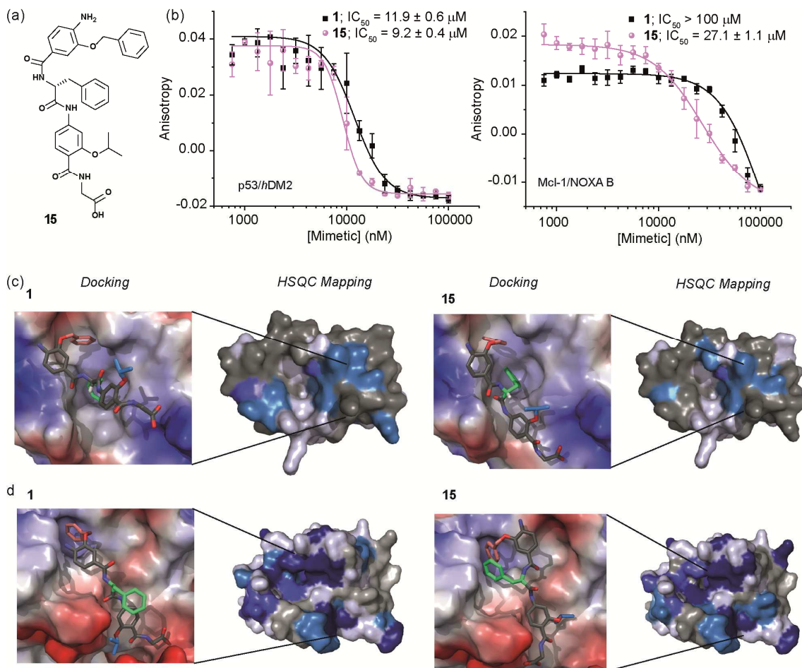
Figure 5 (a) Chemical structure of the D-Phe functionalised hybrid mimetic 15 . (b) Dose-response curves of L-Phe ( 1 ) and D-Phe ( 15 ) hybrid mimetics in FA competition assays against p53/hDM2 (left) and Mcl-1/NOXA-B (right). (c) Docking and 1 H- 15 N HSQC perturbation shift studies (dark blue; large shift/ peak disappears, light blue; medium shift, grey; no shift, white unassigned) with hDM2 (PDB ID: 1YCR): docked hybrid 1 with protein surface 3D representation and chemical shift mapping (left), docked hybrid 15 with protein surface 3D representation and chemical shift mapping (right). (d) Docking and 1 H- 15 N HSQC perturbation shift studies with Mcl-1 (PDB ID: 2JM6): docked hybrid 1 with protein surface 3D representation and chemical shift mapping (left), docked hybrid 15 with protein surface 3D representation and chemical shift mapping (right). Spectra recorded at 600 MHz, in 20mM HEPES pH 7.0, 50mM NaCl, 0.5mM DTT, 2.5% Glycerol, 5% DMSO at 25 °C
