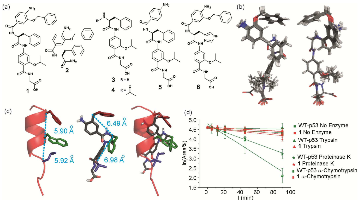
Figure 2 (a) Structures of a model hybrid mimetic 1 and five control derivatives 2-6 . (b) NMR derived structure of compound 1 (left, front and right rear). (c) overlay of the NMR structure of mimetic 1 and p53 transactivation domain illustrating good matching of side chains between mimetic and helix together with distances between key positions (d) Kinetics of degradation from proteolytic studies performed on hybrid 1 (red) and WT-p53 (green) treated with no enzyme (square), trypsin (triangle), \alpha -chymotrypsin (sphere) and proteinase K (star) in 1:10000 enzyme/substrate ratio.
