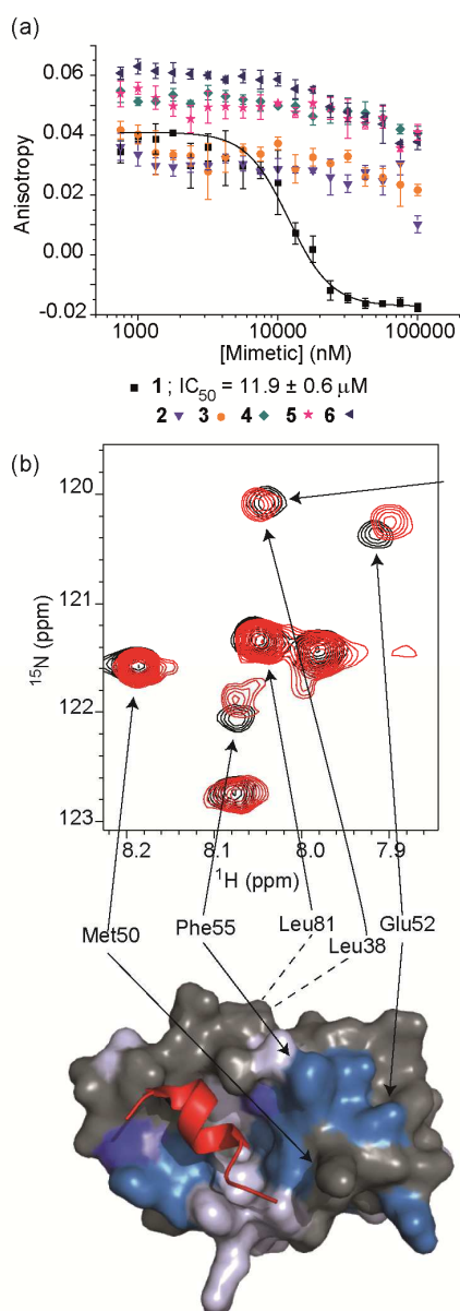
Figure 3. (a) Dose-response curves of hybrids 1 (black), 2 (purple), 3 (orange), 4 (dark cyan), 5 (magenta) and 6 (dark blue) in a FA competition assay against the p53/hDM2 PPI (errors bars correspond to three experimental replicates). (b) Left; Partial ^1\text{H} - ^{15}\text{N} HSQC spectrum of the ^{15}\text{N} -labelled 125 \mu\text{M} solution of hDM2 (black) overlaid with the HSQC spectrum of hDM2 (125 \mu\text{M} ) in complex with a 200 \mu\text{M} solution of 1 (red), highlighting shift changes (dark blue; large shift, light blue; medium shift, grey; no shift, white unassigned), of pertinent residues (600 MHz, 100 mM sodium phosphate buffer pH 7.3, 2.5% glycerol, 1 mM DTT, 6% DMSO, 25 ^\circ\text{C} ). Right; chemical shift perturbation mapping onto the crystal structure of p53/hDM2 (PDB ID: 1YCR).
