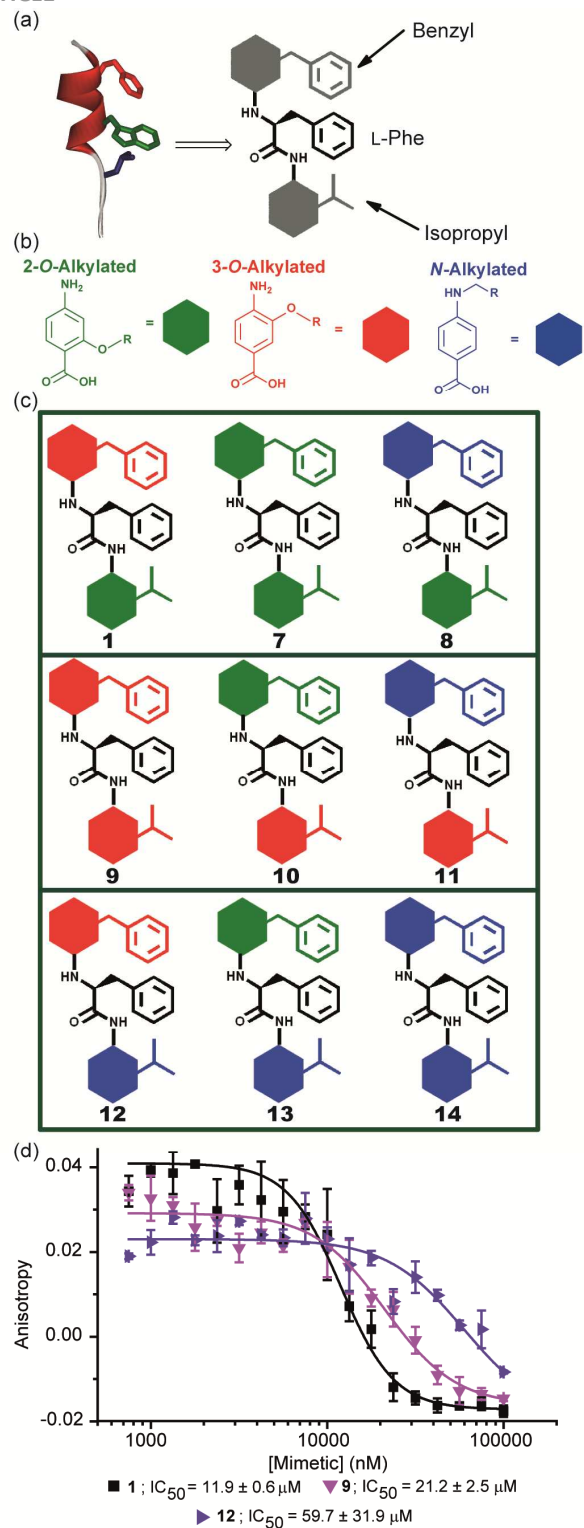
Figure 4 (a) Cartoon depicting the design of a library of hybrid mimetics for sequence-dependent SAR studies. (b) 2- O (green), 3- O (red) and N -alkylated (blue) aminobenzoic acid building blocks; (c) Cartoon representation of the library of hybrid mimetics for sequence-dependent SAR studies; (d) Dose-response curves of hybrids 1 (black), 9 (magenta) and 12 (violet) in a FA competition assay against the p53/hDM2 PPI.
