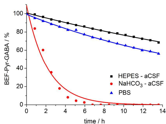
Figure 6. Stability of BEF-Pyr-GABA (20 \mu M) in aqueous buffers at pH 7.4 at 20 ^{\circ} C: HEPES-based aCSF – black, NaHCO 3 based aCSF – red, PBS – blue; HEPES: 4-(2-hydroxyethyl)piperazine-1-ethanesulfonic acid, aCSF: artificial cerebrospinal fluid, PBS: phosphate-buffered saline. Changes in concentration of BEF-Pyr-GABA were determined by HPLC. Mono-exponential fitting curves were applied to the data.
