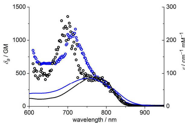
Figure 4. TPA spectra (circles) overlaid with double-wavelength one-photon absorption spectra (lines); blue - BEF-OH recorded in water, black - BEF-OTBDMS ( t -butyldimethylsilyl ether derivative) recorded in EtOH.
