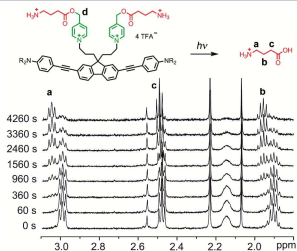
Figure 7. 1 H-NMR spectra from a representative uncaging experiment, which shows the disappearance of caged-GABA signals with a concurrent increase of a new set of multiplets later found to be free GABA (signals “a-c”). Decrease in intensity of signal “d” (5.29 ppm) is not shown.
