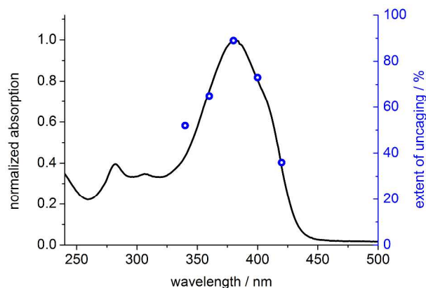
Figure 10. Normalized absorption spectrum of BEF-Pyr-Trp in citric acid/sodium citrate buffer (pH 3.0) (black line) plotted in the scale with extent of photolysis, expressed as yield of released tryptophan upon 3800 s of irradiation of BEF-Pyr-Trp at 340–420 nm (blue circles).
