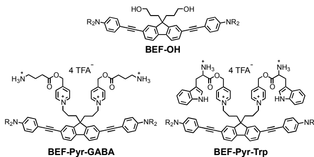
Figure 2. Structure of model electron-donor BEF-OH , caged tryptophan, BEF-Pyr-Trp , and caged GABA, BEF-Pyr-GABA ; R = (CH 2 CH 2 O) 7 CH 3 .
