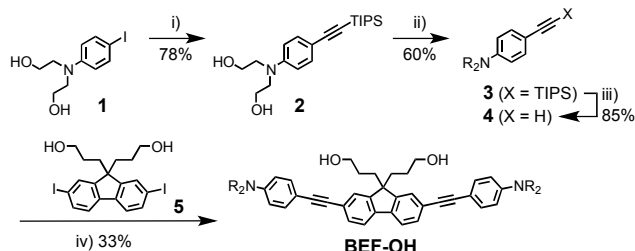
Scheme 1. Reagents: i) TIPS-acetylene, Pd(OAc) 2 , PPh 3 , CuI, DIPA, 50 °C, 16 h, ii) CH 3 (OCH 2 CH 2 ) 6 OTs, NaH, THF, reflux, 48 h, iii) TBAF, THF, 20 °C, 12 h, iv) 4 , Pd(OAc) 2 , PPh 3 , CuI, DIPA, MeCN, 20 °C, 3 h; Ts = p -toluenesulfonate, TIPS = triisopropylsilyl, THF = tetrahydrofuran, DIPA = diisopropylamine, TBAF = tetra- n -butylammonium fluoride, R = (CH 2 CH 2 O) 7 CH 3 .
