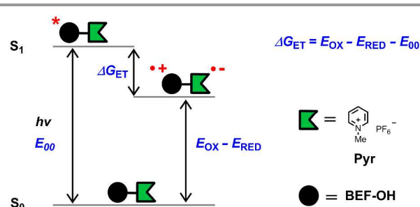
Figure 5. Diagram representing the energy levels of the species involved in electron transfer. Right: structure of N -methyl pyridinium hexafluorophosphate ( Pyr ), the model compound used in electrochemical measurements.
