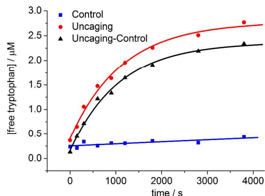
Figure 9. The change in concentration of tryptophan upon photolysis of BEF-Pyr-Trp at pH 3.0 and 360 nm; red circles – photolyzed sample, blue squares – control samples stored in the dark, black triangles – net concentration of tryptophan released upon uncaging. The concentration of tryptophan was determined by HPLC.
