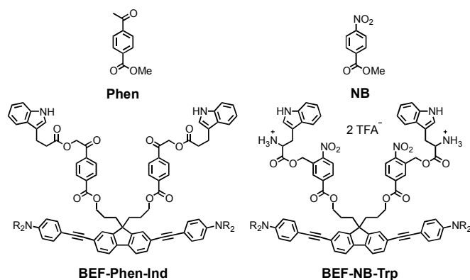
Figure 11. The structures of alternative electron acceptor units: methyl 4-acetylbenzoate ( Phen ) and methyl 4-nitrobenzoate ( NB ) and corresponding protecting groups based on the banana-shaped fluorene dye BEF-Phen-Ind and BEF-NB-Trp ; \text{R} = (\text{CH}_2\text{CH}_2\text{O})_7\text{CH}_3 .
