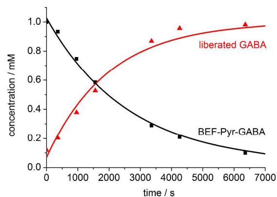
Figure 8. The change in concentration of BEF-Pyr-GABA (black squares) and free GABA (red triangles) over time. Concentration of free GABA and BEF-Pyr-GABA were determined by integration of signal “c” and “d” respectively relative to t -butanol. The presence of free GABA was confirmed by doping an irradiated solution with an authentic sample, which resulted in no new signals and an increase in the intensity of the suspected GABA signals (Figure S30).
