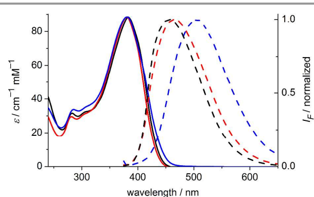
Figure 3. Absorption (solid) and emission (dashed) spectra of BEF-OH in THF (black), EtOH (red) and water (blue). Excitation wavelength: 366 nm.
