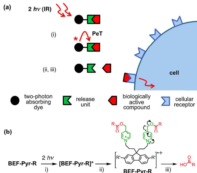
Figure 1. Concept of a photolabile protecting group operating via photoinduced electron transfer. Upon two-photon excitation (i) the dye unit donates an electron to the release unit (ii), which undergoes photochemical reaction and liberates the drug (iii).
