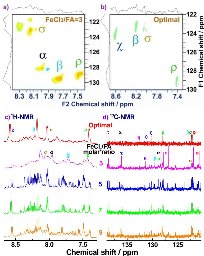
Fig. 5 ^1\text{H} - ^{13}\text{C} 2D HSQC spectra of (a) PFA synthesized with an \text{FeCl}_3 /FA molar ratio of 3 at fixed polymerization temperature of 50\text{ }^\circ\text{C} and polymerization time of 18 h and (b) PFA synthesized under the optimal conditions. (c) ^1\text{H} -NMR and (d) ^{13}\text{C} -NMR spectra of the PFAs synthesized with various \text{FeCl}_3 /FA molar ratios.
