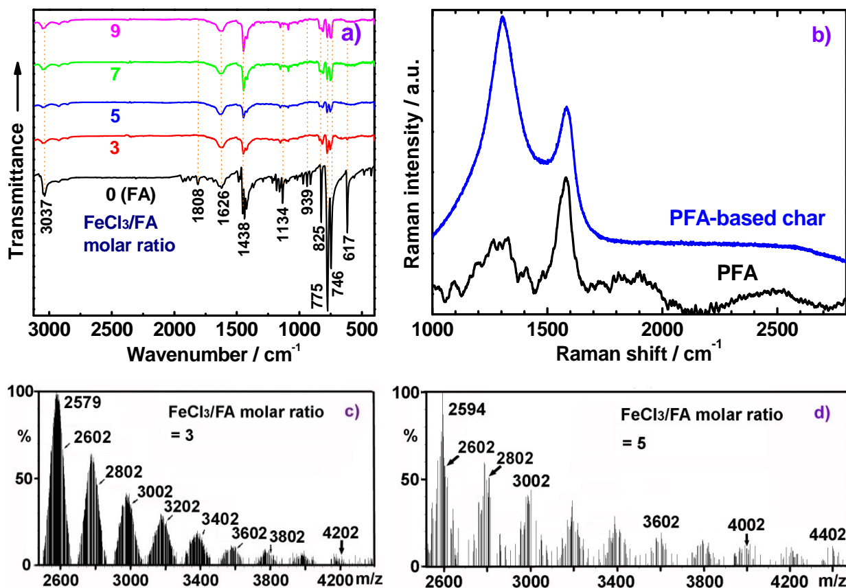
Fig. 3 a) IR spectra of FA monomer and PFA synthesized with various FeCl 3 /FA ratios at fixed conditions: drop-wise addition of FA monomer solution, C 6 H 14 /CH 3 NO 2 volume ratio of 3/2, polymerization temperature of 50 °C, and polymerization time of 18 h. b) Raman spectra of the PFA particles with FA/FeCl 3 molar ratio of 7 and the PFA particles-based char at high temperature in nitrogen; c-d) MALDI-TOF MS spectra of FA monomer and PFA synthesized with various FeCl 3 /FA ratios at fixed conditions: drop-wise addition of FA monomer solution, C 6 H 14 /CH 3 NO 2 volume ratio of 3/2, polymerization temperature of 50 °C, and polymerization time of 18 h.
