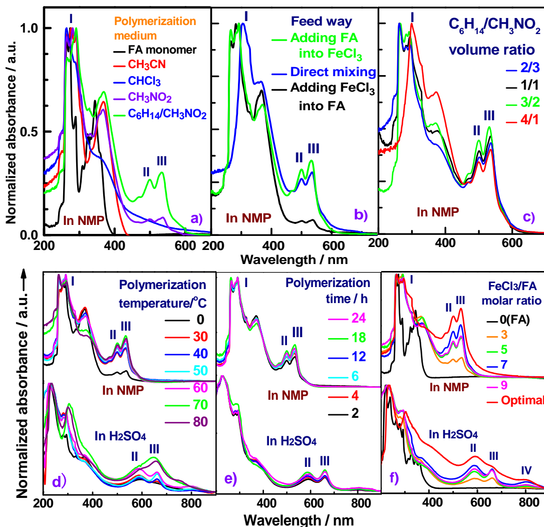
Fig. 1 UV-vis spectra of PFA synthesized a ) in four different polymerization media; b ) by three different feed methods: 1) drop-wise addition of a FA solution to a \text{FeCl}_3 solution, 2) direct mixing while holding the other conditions fixed ( \text{FeCl}_3/\text{FA} molar ratio of 5 in \text{C}_6\text{H}_{14}/\text{CH}_3\text{NO}_2 vol. ratio of 3/2 at 50 °C for 24 h), and 3) by drop-wise addition of a \text{FeCl}_3 solution into a FA solution; and by c ) using four different \text{C}_6\text{H}_{14}/\text{CH}_3\text{NO}_2 volume ratios: 2/3, 1/1, 3/2 and 4/1, while holding the other conditions constant (drop-wise addition of a FA solution into \text{FeCl}_3 solution and \text{FeCl}_3/\text{FA} molar ratio of 7 at 70 °C for 24 h). The effect of d ) polymerization temperature at a fixed \text{FeCl}_3/\text{FA} molar ratio of 5 for 24 h, e ) polymerization time at a fixed \text{FeCl}_3/\text{FA} molar ratio of 5 at 50 °C, and f ) \text{FeCl}_3/\text{FA} molar ratio at 50 °C for 18 h.
