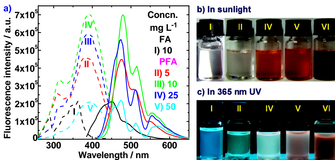
Fig. 7. (a) Fluorescence excitation spectra (dashed lines) taken at I) 452 nm, II) 472 nm, III) 478 nm, and IV-V) 474 nm emitting and fluorescence emission spectra (solid lines) taken at I) 363 nm, and II-V) 400 nm exciting. (b) DMSO solution in sunlight and (c) under 365 nm UV for I) 10 mg L -1 FA and the optimal PFA at different concentrations: II) 5, III) 10, IV) 25, V) 50, and VI) 50 mg L -1 .
