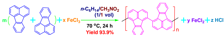
Scheme 1. Chemical oxidative polymerization of FA in a biphasic interface between hexane and nitromethane.
