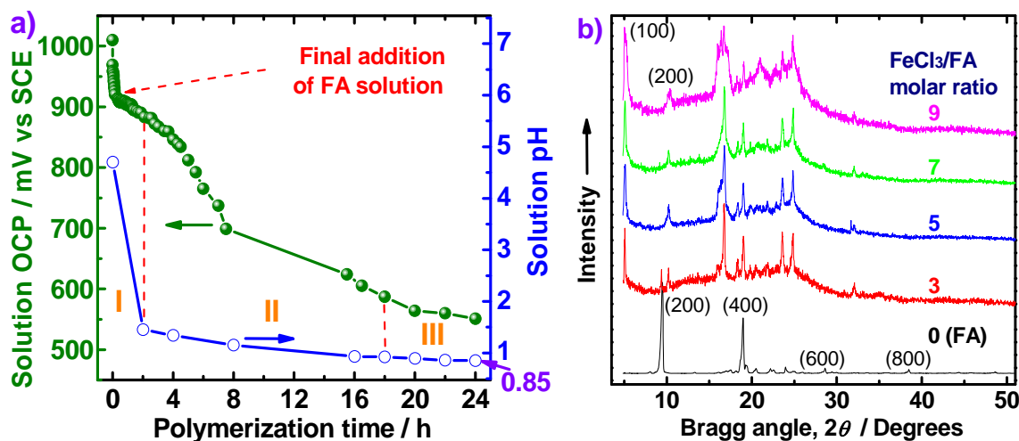
Fig. 6 a) The open-circuit potential (OCP) and pH variations of the FA polymerization solution with the polymerization time at a fixed FeCl 3 (28 mmol)/FA (4 mmol) molar ratio of 7 in C 6 H 14 /CH 3 NO 2 with a volume ratio of 30 mL/20 mL at 50 °C. The FA solution in C 6 H 14 has initial OCP and pH of 165 mV vs SCE and 5.6, respectively. The orange Roman numerals indicate the three polymerization stages. b) Wide-angle X-ray diffractograms of the FA monomer and PFA synthesized in C 6 H 14 /CH 3 NO 2 with a volume ratio of 30 mL/20 mL at 50 °C with four FeCl 3 /FA molar ratios.
