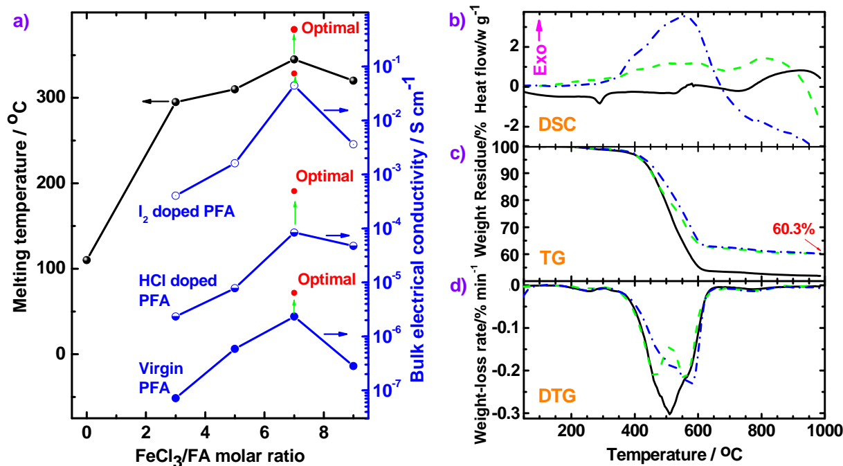
Fig. 9 a) Melting temperature and conductivities of FA and PFA synthesized with various \text{FeCl}_3/\text{FA} molar ratios and under optimal conditions. b) DSC, c) TG, and d) DTG curves of PFAs synthesized at different polymerization temperatures: (black solid) 50 ^{\circ}\text{C} and \text{FeCl}_3/\text{FA} molar ratio of 5 for 24 h; (green dash) 70 ^{\circ}\text{C} and \text{FeCl}_3/\text{FA} molar ratio of 5 for 24 h; (blue dash dot) 70 ^{\circ}\text{C} and \text{FeCl}_3/\text{FA} molar ratio of 7 for 18 h. Other synthetic conditions were fixed: drop-wise addition of FA to \text{FeCl}_3 solutions and \text{C}_6\text{H}_{14}/\text{CH}_3\text{NO}_2 volume ratio of 3/2.
