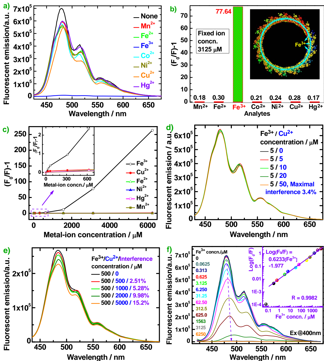
Fig. 8. a) Fluorescence emission spectra and b) (F 0 /F)-1 values of 10 mg L -1 optimal PFA in DMSO containing different metal ions at a fixed concentration of 3125 μM (inset: schematic diagram of the amplified quenching of PFA fluorescence by Fe 3+ ); c) relationship between (F 0 /F)-1 and metal-ion concentration of 10 mg L -1 optimal PFA in DMSO; d-e) the influence of coexisted Cu 2+ on the PL emission of the optimal PFA solution containing Fe 3+ ; f) PL emission spectra of 10 mg L -1 optimal PFA in DMSO containing Fe 3+ of 0 to 6250 μM.
