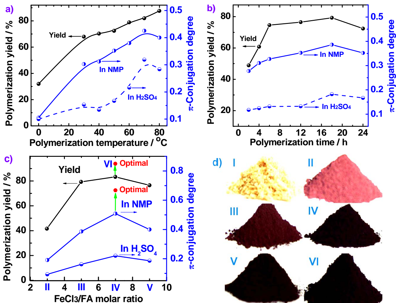
Fig. 2 Effect of a) polymerization temperature, b) polymerization time, and c) \text{FeCl}_3/\text{FA} molar ratios on the polymerization yield and conjugation degree of PFA, and d) the powder in sunlight of I) FA and PFAs synthesized with various \text{FeCl}_3/\text{FA} molar ratios: II) 3, III) 5, IV) 7, V) 9, and VI) optimal PFA in \text{C}_6\text{H}_4/\text{CH}_3\text{NO}_2 as a biphasic medium with a volume ratio of 30 mL/20 mL at 50 ^{\circ}\text{C} .
