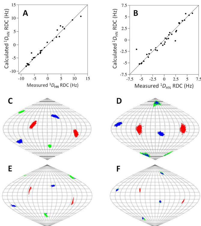
Figure 5 Correlations between experimental and calculated ^1D_{\text{HN}} RDCs recorded at a ^1\text{H} NMR frequency of 600 MHz for C7-Tm 3+ (A) and C8-Tm 3+ (B) tagged ubiquitin A28C. Solid lines represent perfect correlation. Orientations of the principal axes of the alignment (C C7 , D C8 ) and \Delta\chi (E C7 , F C8 ) tensors. The points show where the principal axes of the spheres penetrate the sphere with the axes coloured as follows: z (blue), y (green), x (red). For the alignment tensors, 1,000 replicates of SVD calculation using the structural noise Monte-Carlo method (‘-mcStruc’) within PALES are shown. For the \Delta\chi -tensors, 1,000 replicates with a random 10% of the PCS data removed each time are shown. The convention |z| > |y| > |x| is used to name the axes, resulting in swapping of the |z| and |y| axes in different fits when their magnitudes are similar.
