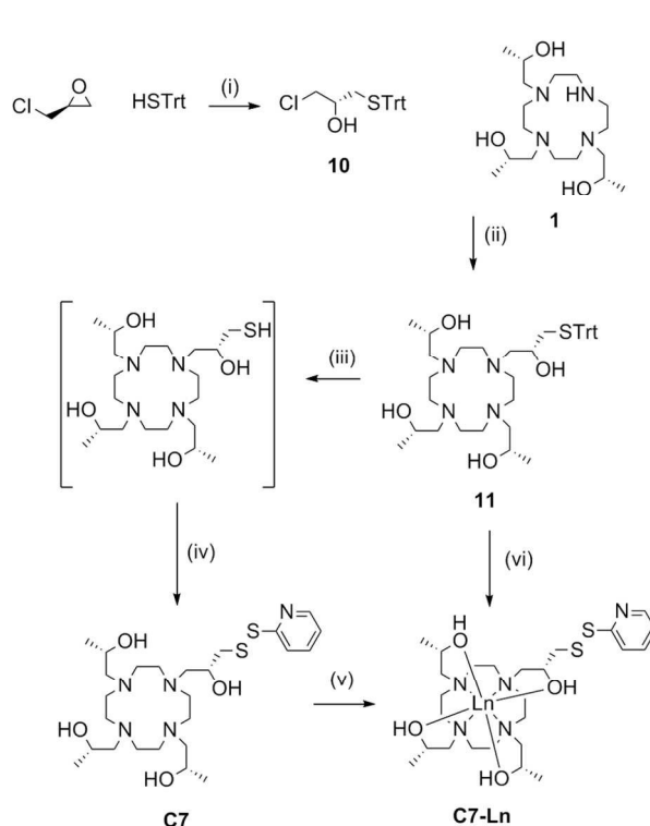
Scheme 3 Synthesis of C7 and its lanthanide complexes. Reagents and conditions: (i) KF, MeOH, RT, 72 h, 95%; (ii) K 2 CO 3 , ACN, reflux, overnight, 60%; (iii) TFA, triethylsilane, DCM, RT, 1 h; (iv) 2,2'-dipyridyl disulfide, MeOH, RT, 15 min, 39% (from 11 ); (v) LnCl 3 , EtOH, DIPEA, reflux, overnight; (vi) LnCl 3 , MeOH, reflux, 4 h, 2,2'-dipyridyl disulfide, silver nitrate, RT, 2 h, 34%.
