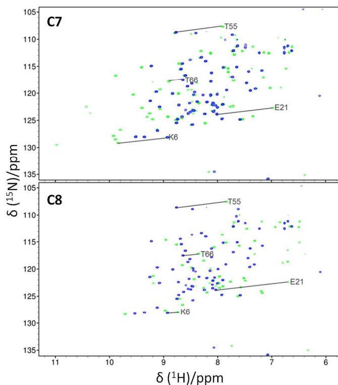
Figure 2 Overlays of ^{15}\text{N} -HSQC spectra of C7 (top spectra) and C8 (bottom spectra) tagged ubiquitin A28C, loaded with either \text{Y}^{3+} (blue) or \text{Tm}^{3+} (green). The spectra were recorded at 25 °C and pH 8.0 at a ^1\text{H} NMR frequency of 600 MHz. Selected PCSs are indicated with solid lines.
