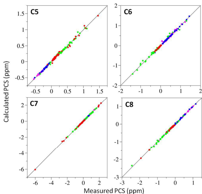
Figure 3 Correlations between experimental and back-calculated PCSs for C5–C8 bound to ubiquitin A28C loaded with either \text{Dy}^{3+} (magenta), \text{Tb}^{3+} (blue), \text{Tm}^{3+} (green) or \text{Yb}^{3+} (red). Solid lines represent perfect correlation.
