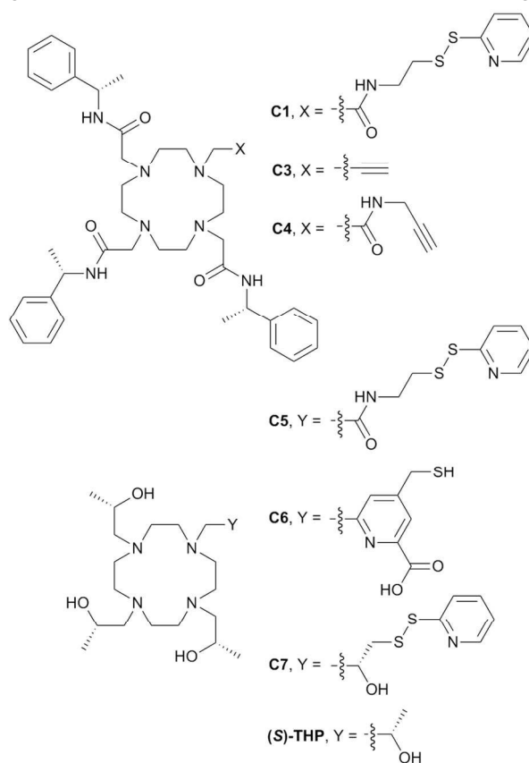
Figure 1 Existing and newly developed LBTs referred to in the text. C2 and C8 are the enantiomers of C1 and C7 , respectively.
