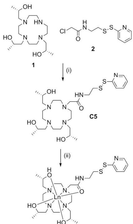
Scheme 1 Synthesis of C5 and its lanthanide complexes. Reagents and conditions: (i) DIPEA, ACN, RT, 72h, 61%; (ii) LnCl 3 , ACN, H 2 O, pH 7, reflux, overnight, quant.
