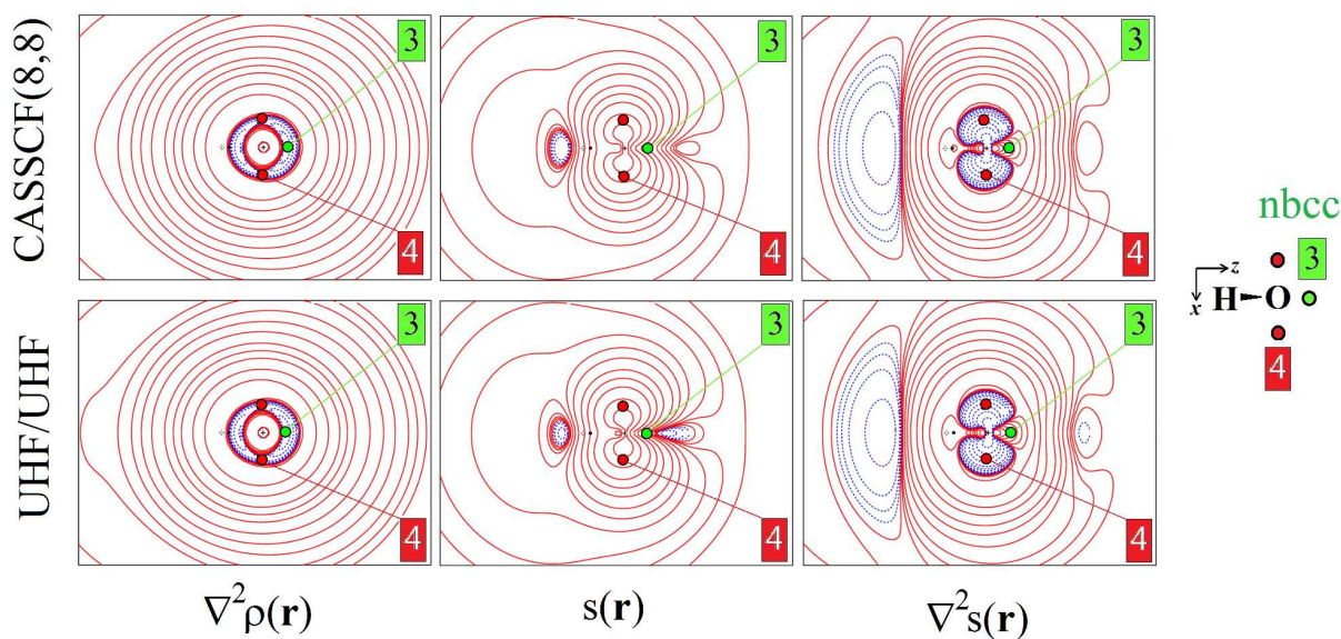
Figure 2. Electron density Laplacian, spin density and its Laplacian in the (x,z) plane, at at (top) CASSCF(8,8) and (bottom) UHF/UHF spin contamination annihilated computational levels. Contour levels as in Figure 1. The non-bonded charge concentration (nbcc, 3 ) and the (3,+1) L(\mathbf{r}) rcps ( 4 ) are shown as green and red dots.
