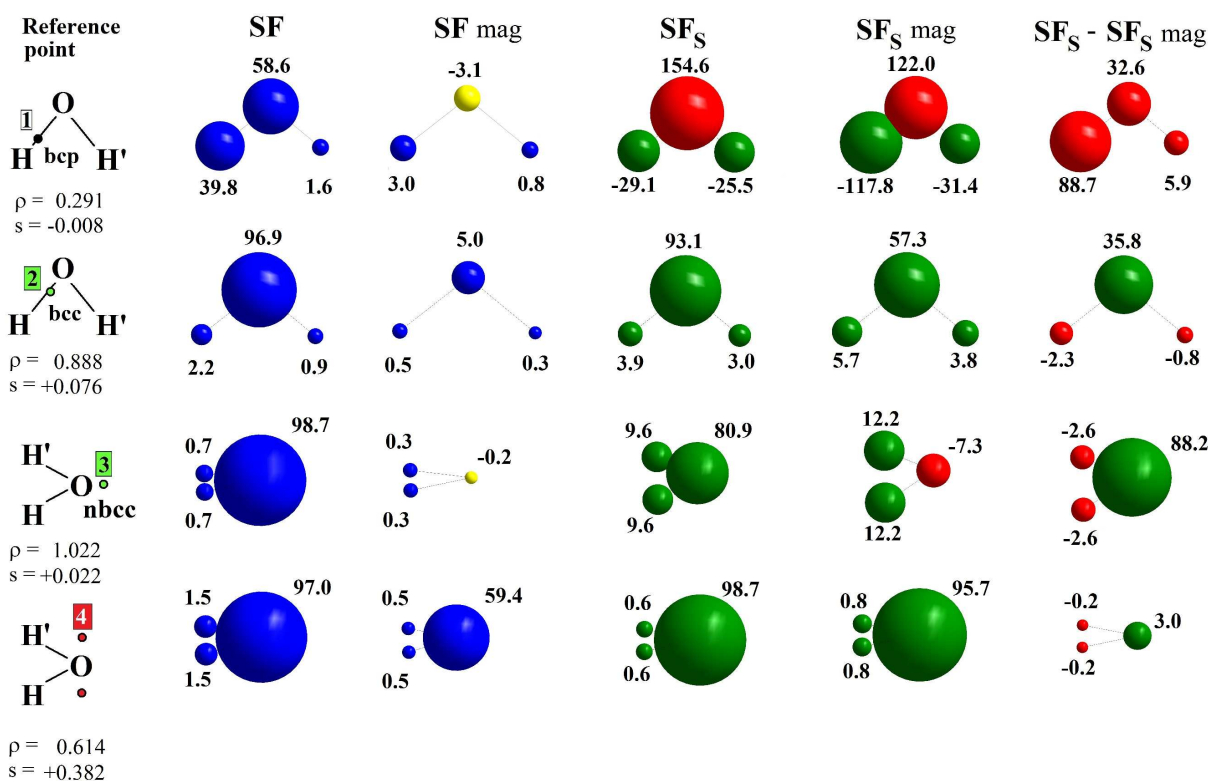
Figure 3. SF and SF S percentage contributions at some reference points (rps) for 3 B 1 H 2 O at the CASSCF(8,8) level. The separate contributions to SF S due to the magnetic (SF S mag) and the remaining (SF S - SF S mag) natural orbitals are also shown (for SF only those due to magnetic orbitals, denoted as SF mag). Each atom is displayed as a sphere, whose volume is proportional to the Source percentage contribution to ρ( r ) or s( r ) values at the rp (first column). Colour codes: blue (yellow) atoms act as positive (negative) sources for ρ at rps; green (red) atoms act as positive (negative) sources for s at rp, hence yielding a α (β) effect at rp (the sign of percentage sources is instead positive or negative whether the atomic source concurs or opposes to s at rp).
