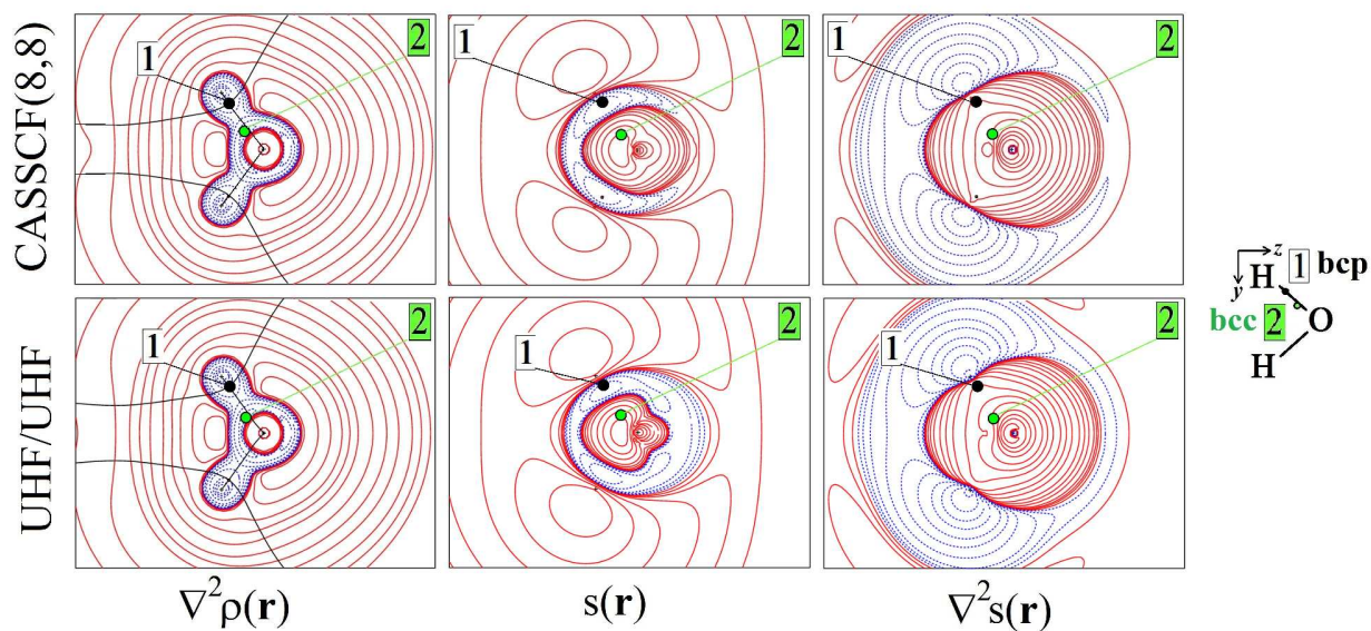
Figure 1. Electron density Laplacian, electron spin density s(\mathbf{r}) and its Laplacian in the (y,z) plane for ^3B_1 H_2O , at (top) CASSCF(8,8) and (bottom) UHF/UHF spin-contamination annihilated computational levels. Atomic units (a.u.) are used throughout. Contour maps are drawn at interval of \pm(2,4,8) \cdot 10^n , -4 \leq n \leq 0 ( s , \nabla^2 s ) and -3 \leq n \leq 0 ( \nabla^2 \rho ). Dotted blue (full red) lines indicate negative (positive) values and full black lines mark boundaries of atomic basins. The O–H bond critical point (bcp, 1 ) and the bonded charge concentration point (bcc, 2 ) are shown as black and green dots.
