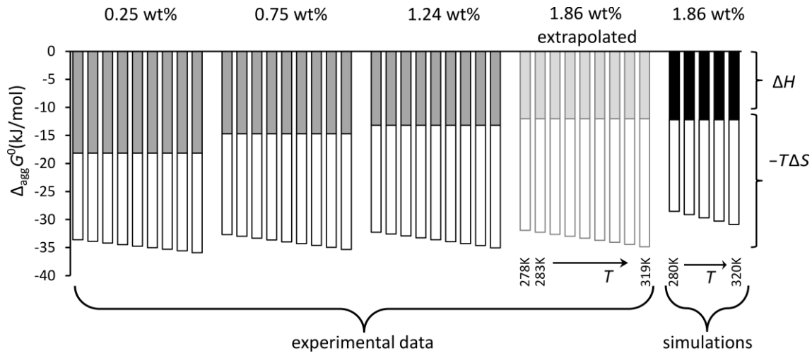
Figure 6. Free energy of association \Delta_{\text{agg}} G^0(T) decomposed into \Delta H and T\Delta S(T) contributions. First three sets of data are for experimental results at different concentrations. The fourth set of data is obtained using extrapolated experimental results for \Delta_{\text{agg}} G^0 . For experimental data \Delta H is shown as grey and T\Delta S(T) as white columns. The temperature in experiment was sampled in a range of 278 – 319 K with an increment of 5 K except for the last value of 319 K. The last set of data is our simulation results, where \Delta_{\text{agg}} G^0 is obtained using Wertheim approach applied to the PMF profiles for binding a molecule to a stack of three molecules. For simulation data \Delta H is shown as black and T\Delta S(T) as hatched columns. The temperature range in simulation was 280 – 320 K with an increment of 10 K.
