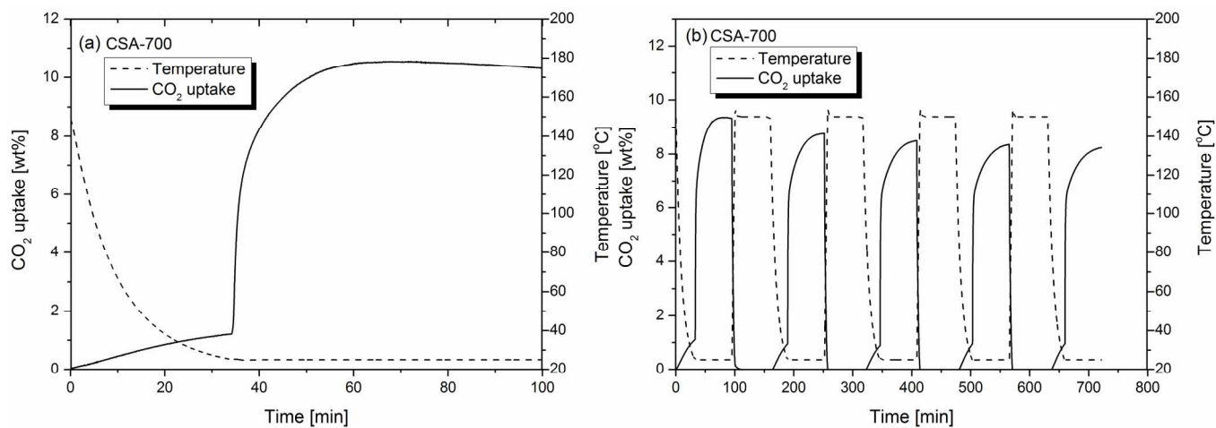
Figure 6: CO 2 sorption characteristics of CSA-700 under flowing gas mixture of 15 vol% CO 2 and 85 vol% N 2 at 25 °C: (a) a single cycle adsorption; and (b) five cycles of adsorption and desorption.
