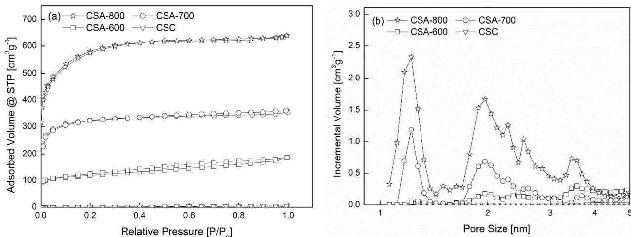
Figure 3: (a) Nitrogen sorption isotherms of samples prepared under different conditions and (b) their corresponding pore size distributions (Log).
