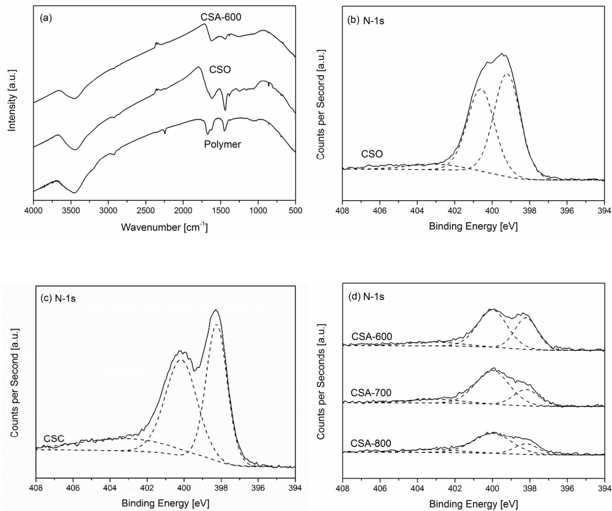
Figure 4: (a) Infrared spectra of the polymer, oxidized polymer (CSO) and activated carbon sphere. XPS N-1s spectra of (b) the oxidized polymer spheres, (c) carbonized sphere (CSC) and (d) activated carbon spheres CSA prepared under different conditions.
