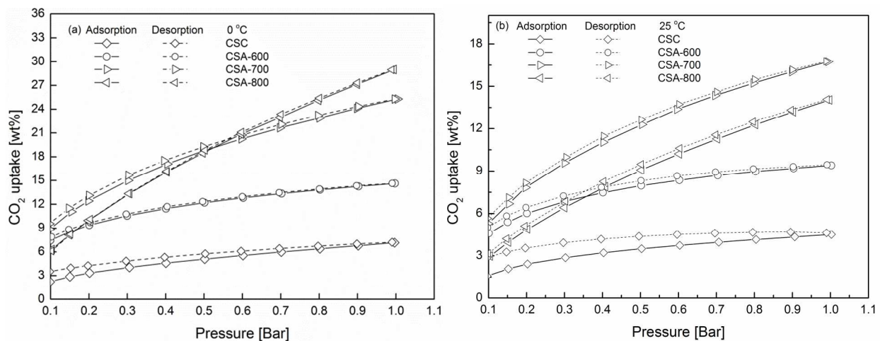
Figure 5: CO 2 adsorption isotherms of carbon spheres prepared under different conditions at (a) 0 and (b) 25 °C from 0.1 to 1 bar.
