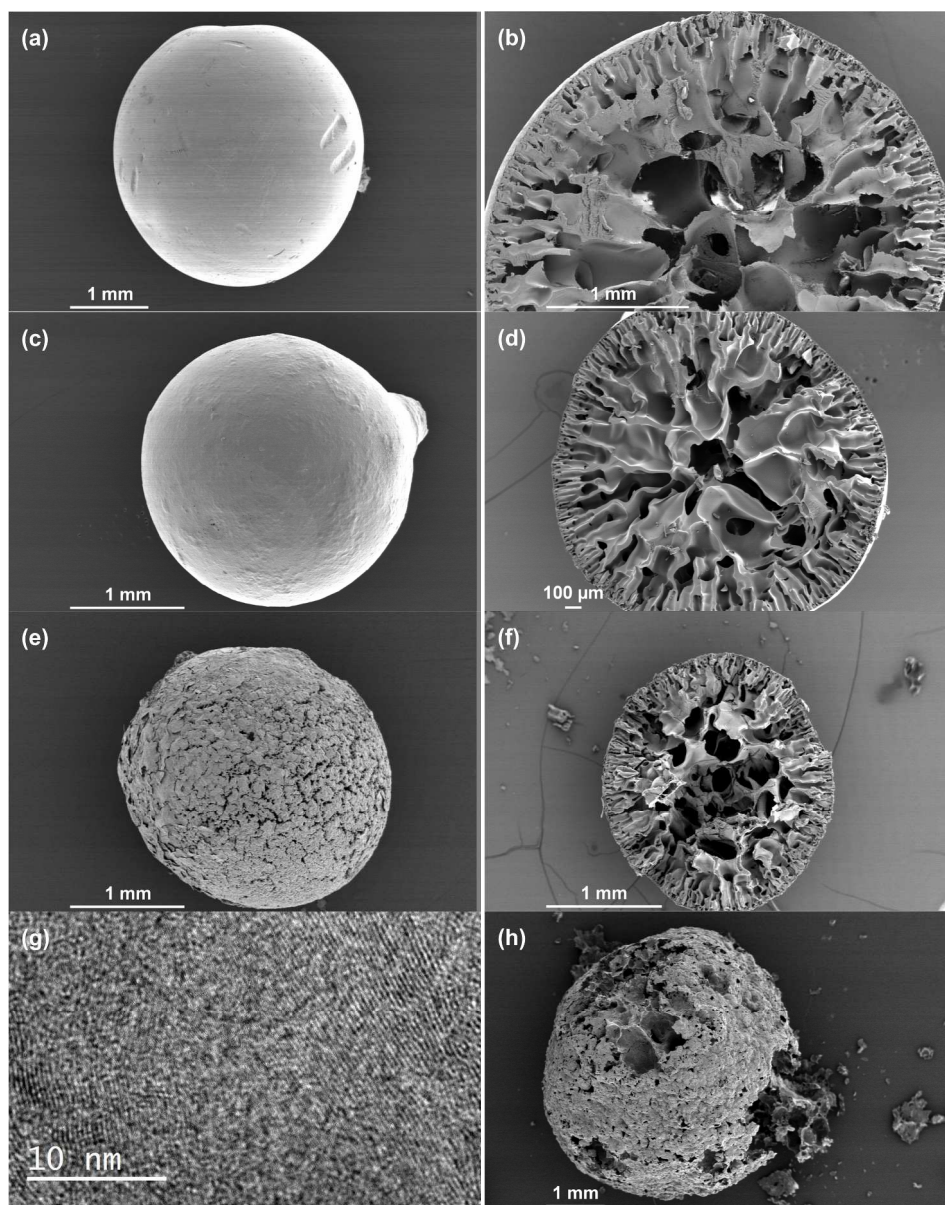
Figure 1: SEM images of (a) a typical polymer sphere, (c) an oxidized polymer sphere and (e) an carbon sphere activated with a KOH/sphere weight ratio of 1:1. (b, d, f) are their corresponding cross-sectional images. (g) A high resolution TEM image of the activated carbon sphere. (h) A fragment from a carbon sphere activated with a higher KOH/sphere weight ratio of 2:1- the original sample has already lost its structural integrity.
