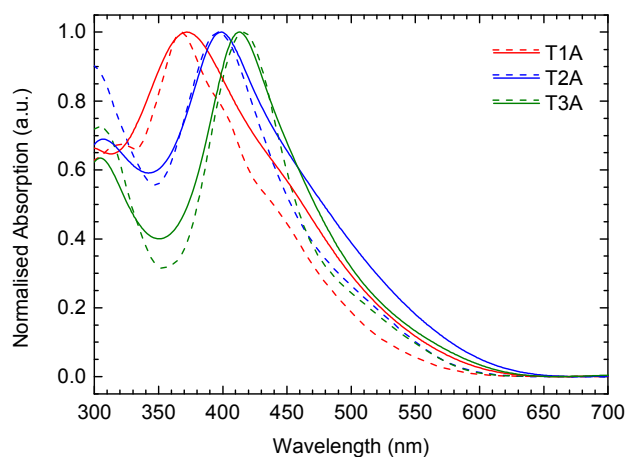
Figure 5. UV-vis absorption spectra for the three truxenone adducts in dichloromethane solution (dashed lines) and as thin films spin-cast from chloroform (solid lines).
