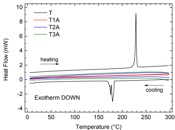
Figure 2. DSC traces (exotherm down) for the truxenone precursor ( T ) and the three truxenone adducts recorded with a heating and cooling rate of 10 °C/min.
