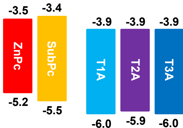
Figure 8. Frontier energy levels (all values in eV) of electron donor and acceptor materials used herein.
