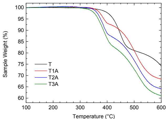
Figure 1. TGA traces for the truxenone precursor ( T ) and the three truxenone adducts recorded in a nitrogen atmosphere at a heating rate of 10 °C/min.
