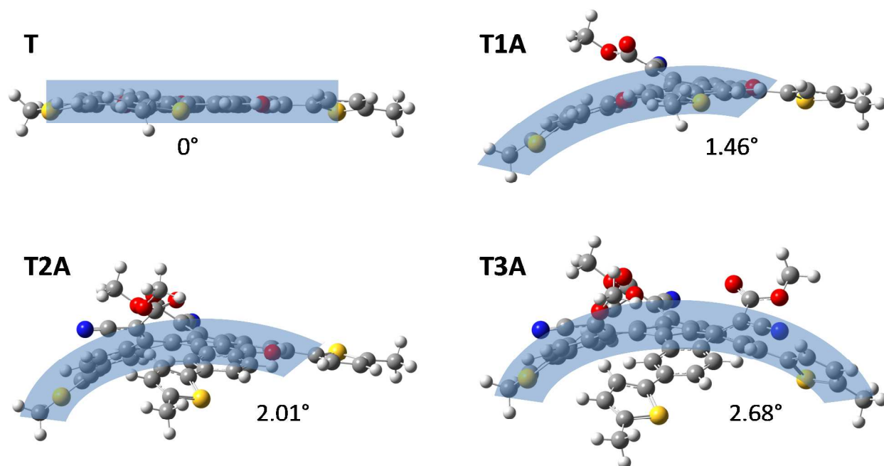
Figure 3. Energy-minimised (Gaussian B3LYP/6-31G*) side-view conformations of the truxenone precursor and the three truxenone adducts with POAV pyramidalization angles indicating the curvature of each molecule.
