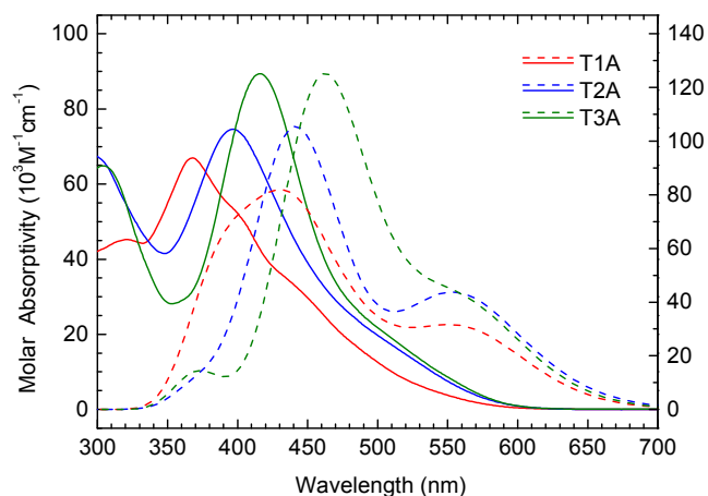
Figure 6. Experimental (solid lines, left y-axis) and theoretical (dashed lines, right y-axis) UV-Vis absorption spectra for the three truxenone adducts in dichloromethane solution.
