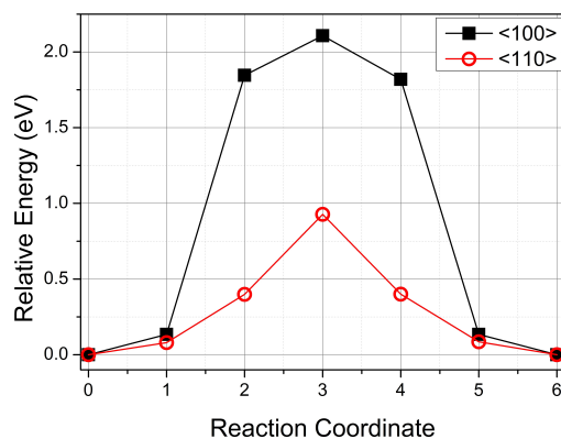
Figure 3: Variation in system energy of tetragonal BaZrO 3 as a constituent oxygen from a peroxide ion migrates in the <100> (black square) and <110> (red circle) directions (in the pseudo-cubic setting). The migration pathway is sampled at five steps along the reaction coordinate.
