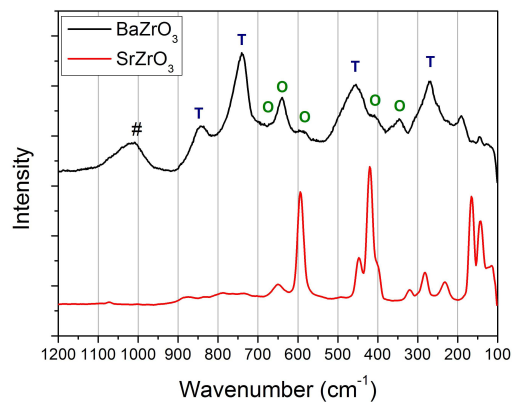
Figure 4: Raman spectra of BaZrO 3 (black) and SrZrO 3 (red) from powder samples before treatment with H 2 O 2 . The tetragonal (T) and orthorhombic (O) peaks are shown for the BaZrO 3 powder (assigned according to [17]). The peak labelled by # is assigned to the O 2 2- stretching mode within the BaZrO 3 crystal.
