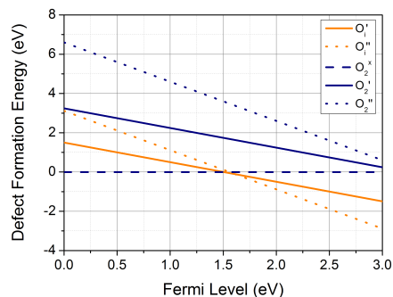
Figure 1: Excess oxygen defect formation energy in \text{BaZrO}_3 as a function of Fermi energy from the top of the valence band to the bottom of the conduction band. Two types of defects are considered, oxygen interstitials (red) and two-oxygen complexes (blue) (where the \text{O}_2^\times is the peroxide ion).
