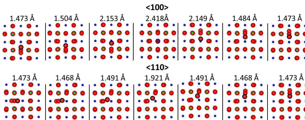
Figure 2: Migration of a constituent oxygen in a peroxide ion in tetragonal \text{BaZrO}_3 from one site to another in the \langle 100 \rangle and \langle 110 \rangle pseudo-cubic directions. The shortest O-O bond distance of the migrating oxygen is shown for each snapshot, the length of \sim 1.47 \text{ \AA} corresponds to the expected peroxide bond length. Oxygen species are represented by large red spheres, zirconium as small blue spheres and barium as small green spheres.
