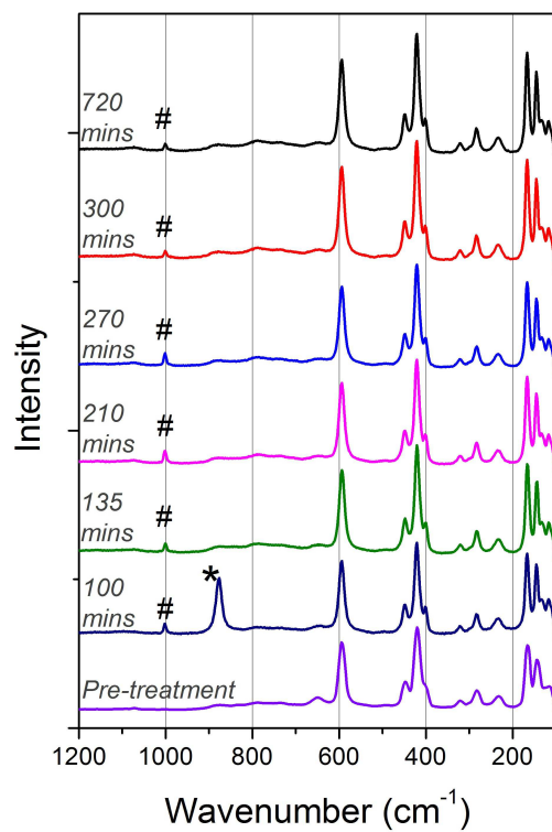
Figure 5: Raman spectra of SrZrO 3 treated with H 2 O 2 taken at various times after removal from H 2 O 2 solution. The peak labelled with * is assigned to the H 2 O 2 solution. The peak labelled with # is assigned to the peroxide ion in the SrZrO 3 lattice.
