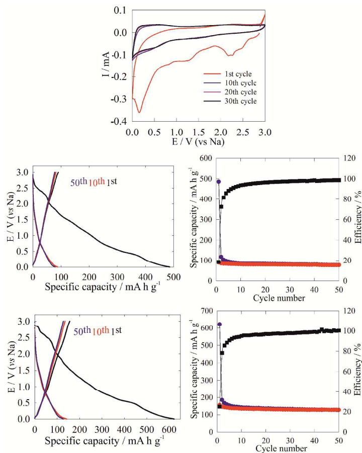
Fig. 7 CV ( 10 \text{ mV s}^{-1} ) in a sodium half cell ( 1\text{M NaPF}_6 in EC/DEC) of an electrode prepared with \text{Mn}_3\text{N}_2 made at 350^\circ\text{C} (top), and voltage profile during galvanostatic reduction and oxidation (left) and specific capacity vs cycle number (right) at 200 \text{ mA g}^{-1} (centre) and 50 \text{ mA g}^{-1} (bottom). In the capacity vs cycle number plots reduction capacity is marked in blue, oxidation capacity in red and Coulombic efficiency in black.
