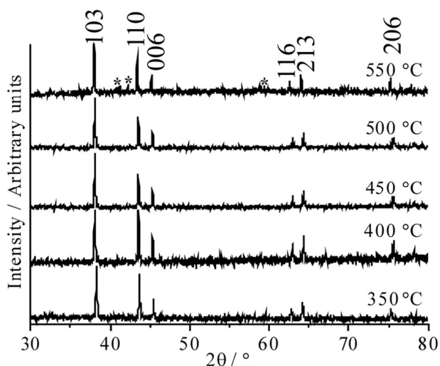
Fig. 1 PXD patterns of \text{Mn}_3\text{N}_2 samples prepared under solvothermal conditions at various temperatures. Reflections due to \text{Mn}_3\text{N}_2 are labelled with Miller indices and those due to \text{Mn}_2\text{N} at 550 °C labelled with asterisks.
