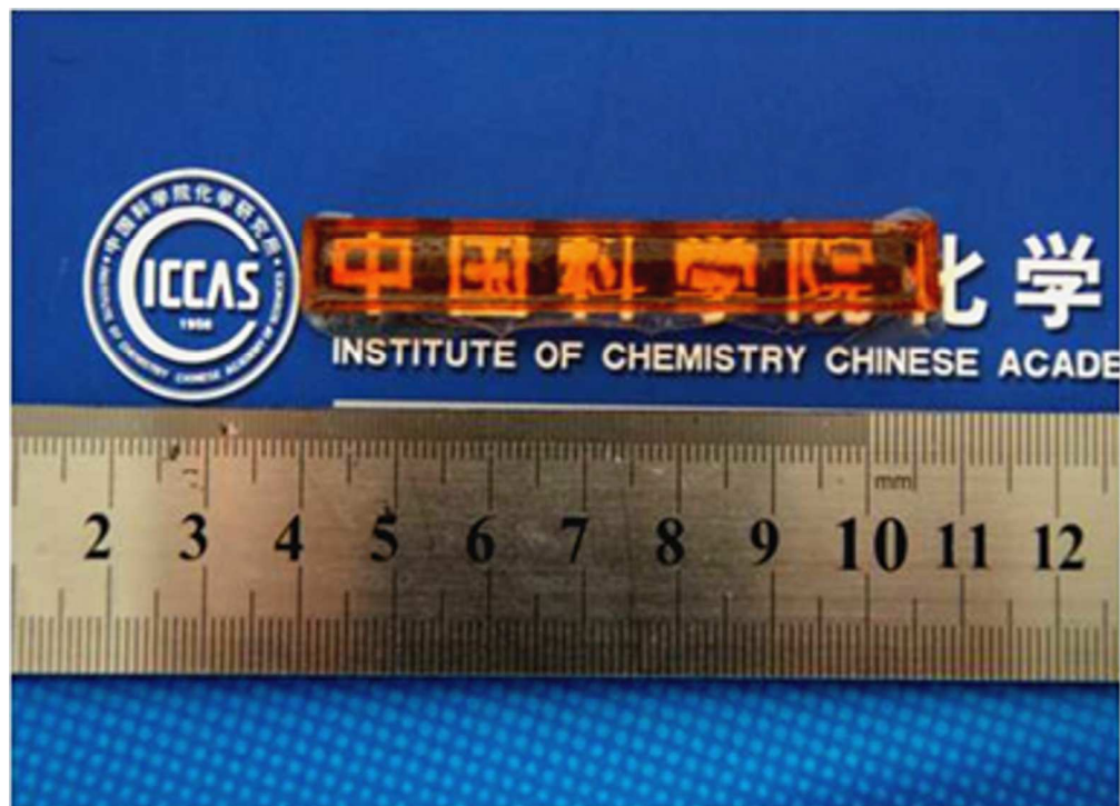
Figure 4. Photo of the 60:40 (organic /inorganic) PEGM600 monolith. 85x61mm (300 x 300 DPI)
