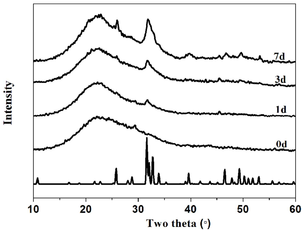
Figure 7. The XRD spectra of hybrid materials (PEGM600, organic/inorganic =60:40, molar ratio) after immersed in SBF for different times. 85x64mm (300 x 300 DPI)
