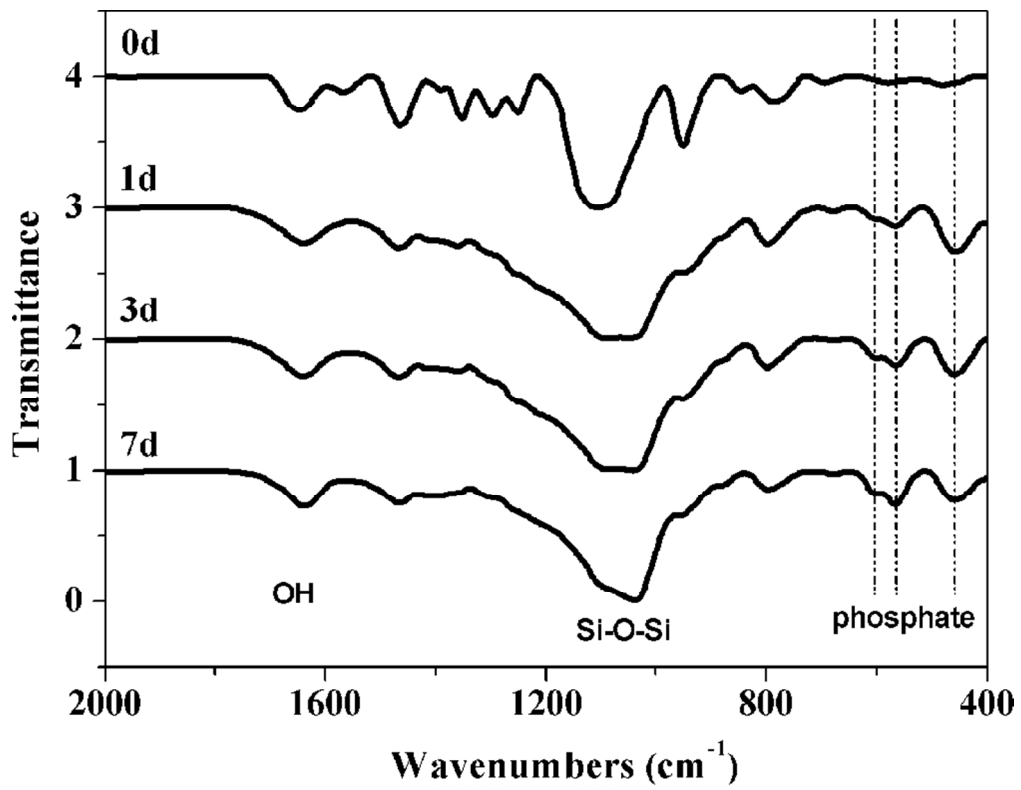
Figure 11. FTIR spectra of the hybrid materials after immersing SBF for 0, 1, 3 and 7 days. 85x65mm (300 x 300 DPI)
