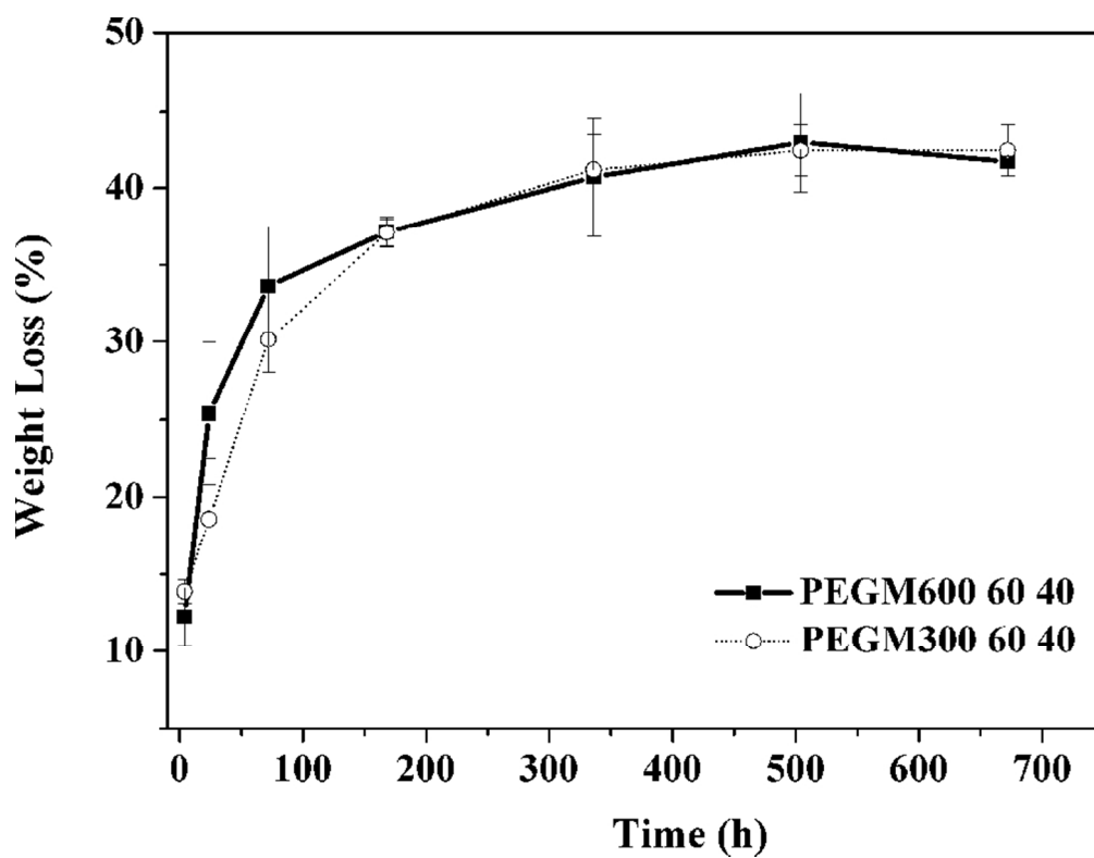
Figure 14. Degradation assay into SBF solution as a function of soaking time for hybrid materials obtained from PEGM600 and PEGM300 with the organic/inorganic ratio of 60:40. 85x65mm (300 x 300 DPI)
