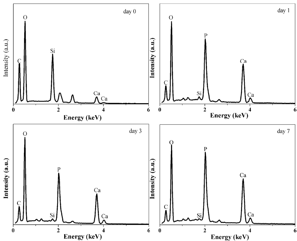
Figure 10. EDXS spectra of the hybrids surface after immersing SBF for 0, 1, 3 and 7 days. 170x137mm (300 x 300 DPI)
