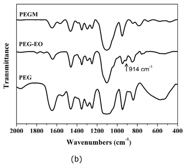
Figure 3. (a) Reaction process illustrating the modification of the PEG-EO end groups, (b) FTIR spectra of PEG, PEG-EO and PEGM. The epoxide group of PEG-EO appears at 914 \text{cm}^{-1} . 170x171mm (300 x 300 DPI)
