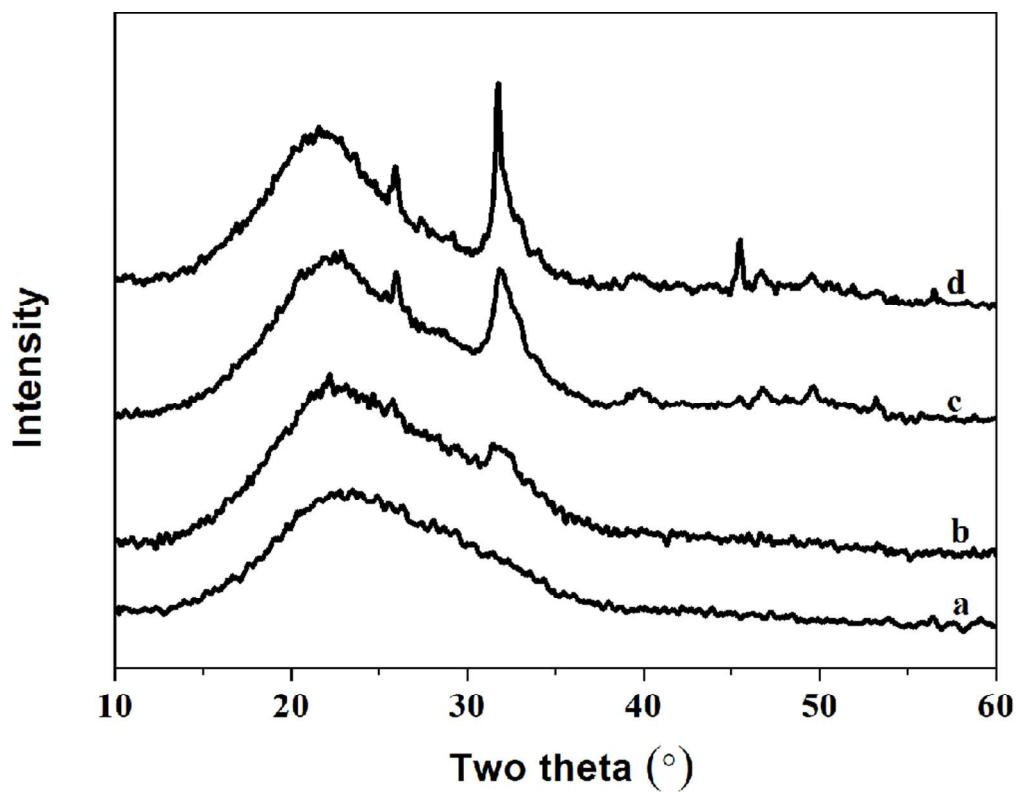
Figure 8. The XRD spectra of hybrid materials with different organic/inorganic (molar ratio, PEGM600) after immersed in SBF for 7 days: a-40:60; b-50:50; c-60:40; d-70:30. 85x66mm (300 x 300 DPI)
