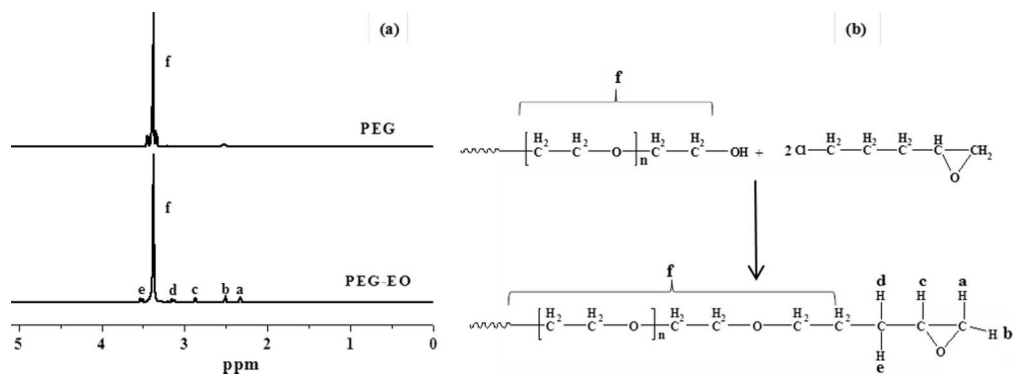
Figure 2(a) ^1\text{H} NMR spectra of PEG (top) and the modified PEG-EO polymer (bottom), illustrates the reaction process of PEG to PEG-EO. (b) 170x61mm (300 x 300 DPI)
