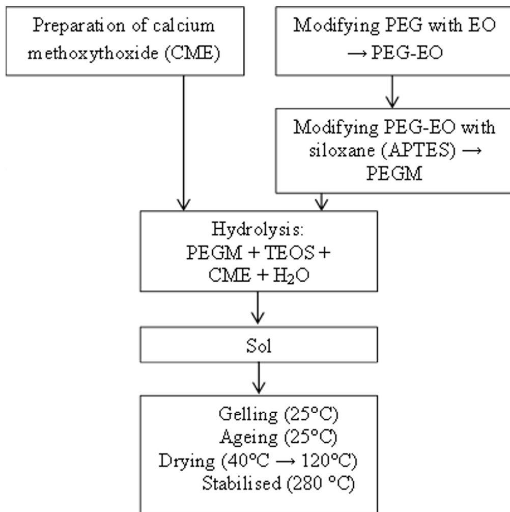
Figure 1. Flow diagram illustrating the hybrid preparation. 85x84mm (300 x 300 DPI)
