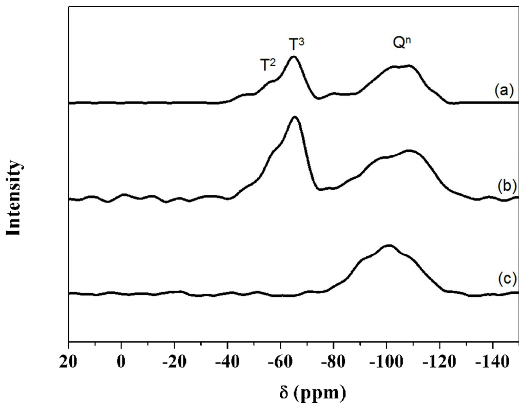
Figure 5. The ^{29}\text{Si} solid state MAS-NMR of the sample obtained from different precursors with the ratio of 60/40(organic/inorganic, molar%) : a—PEGM300/TEOS ; b—PEGM300/TEOS/CME ; c—PEG300/TEOS/CME 85x65mm (300 x 300 DPI)
