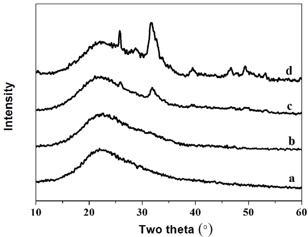
Figure 9. The XRD spectra of hybrid materials with different organic/inorganic (molar ratio, PEGM300) after immersed in SBF for 7 days: a-40:60; b-50:50; c-60:40; d-70:30. 85x65mm (300 x 300 DPI)
