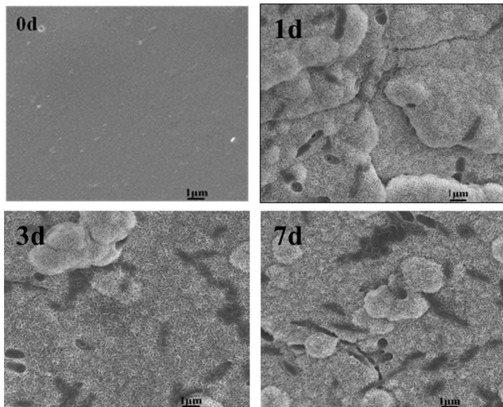
Figure 6. SEM image of hybrid glasses (PEGM600, organic/inorganic=60:40, molar ratio) after immersion in SBF for 0, 1, 3 and 7 days. 99x80mm (300 x 300 DPI)
